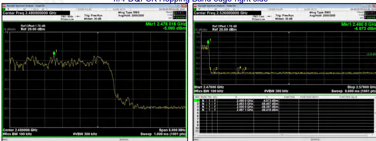
\pi/4 -DQPSK Hopping Band edge-right side
