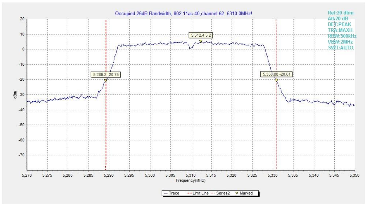
Fig.22 Occupied 26dB Bandwidth (802.11ac-HT40, 5310MHz)
