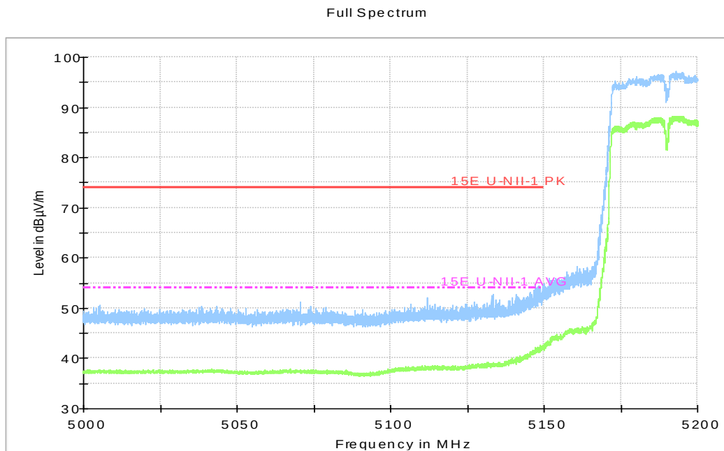
Fig.46 Band Edges (802.11ac-HT40, 5190MHz)
