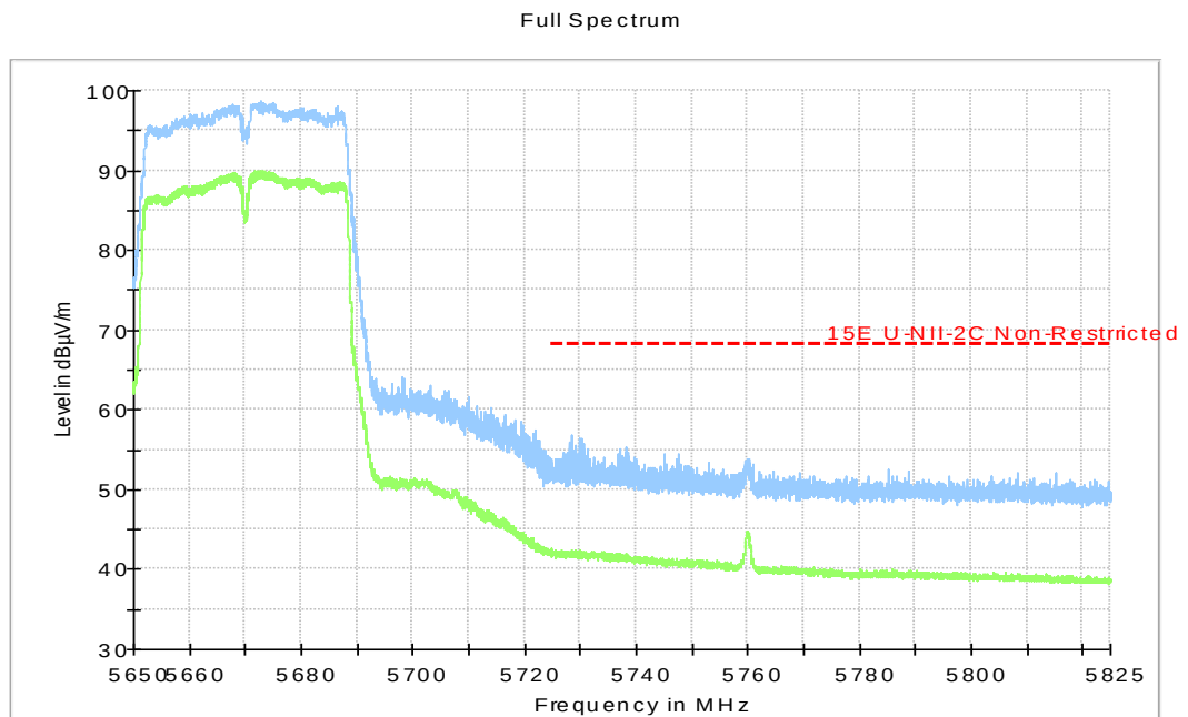
Fig.49 Band Edges (802.11ac-HT40, 5670MHz)
