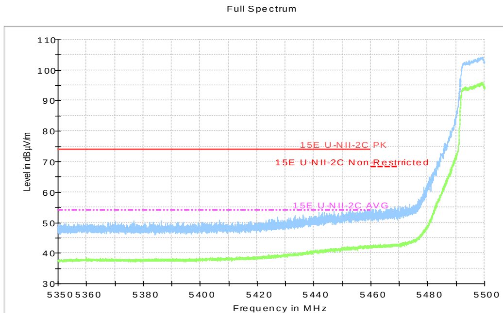
Fig.32 Band Edges (802.11a, 5500MHz)
