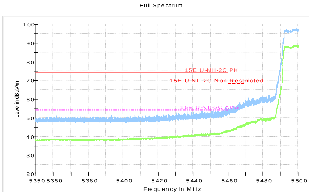
Fig.48 Band Edges (802.11ac-HT40, 5510MHz)
