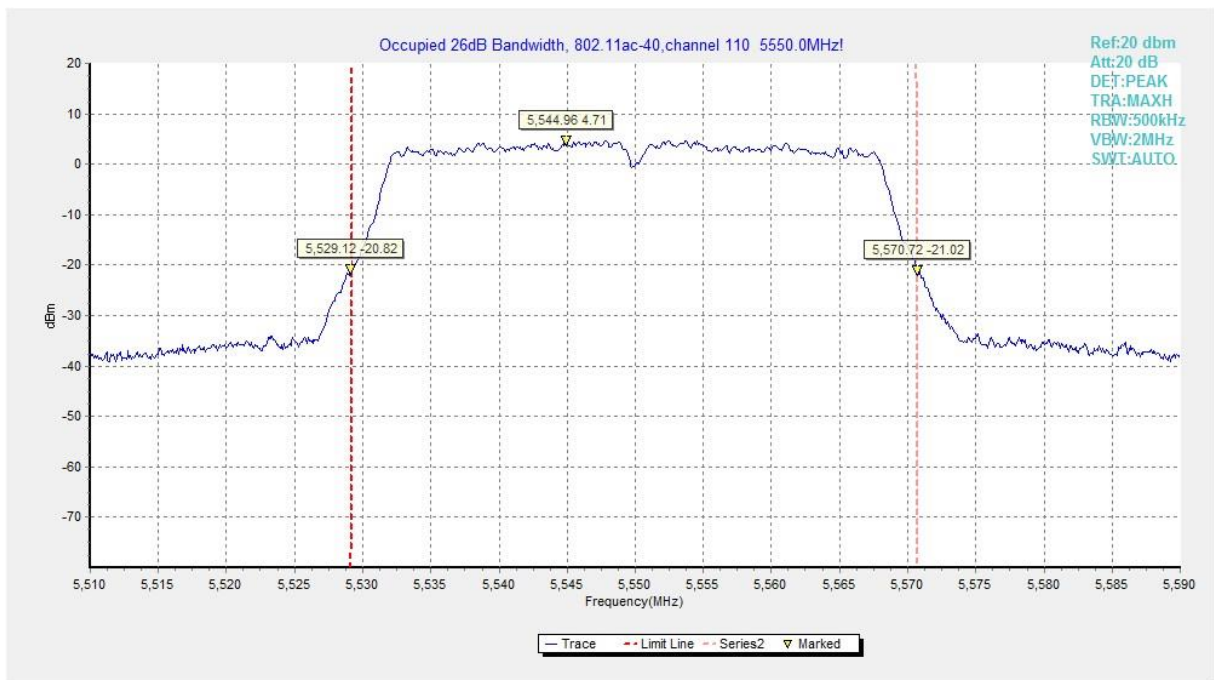
Fig.24 Occupied 26dB Bandwidth (802. 11ac-HT40, 5550MHz)
