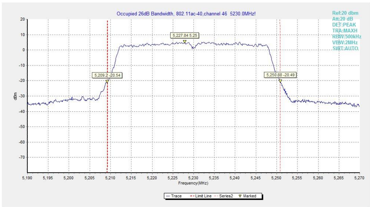
Fig.20 Occupied 26dB Bandwidth (802.11ac-HT40, 5230MHz)
