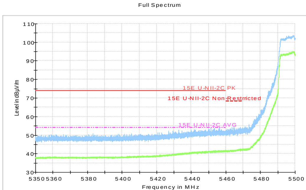
Fig.44 Band Edges (802.11ac-HT20, 5500MHz)
