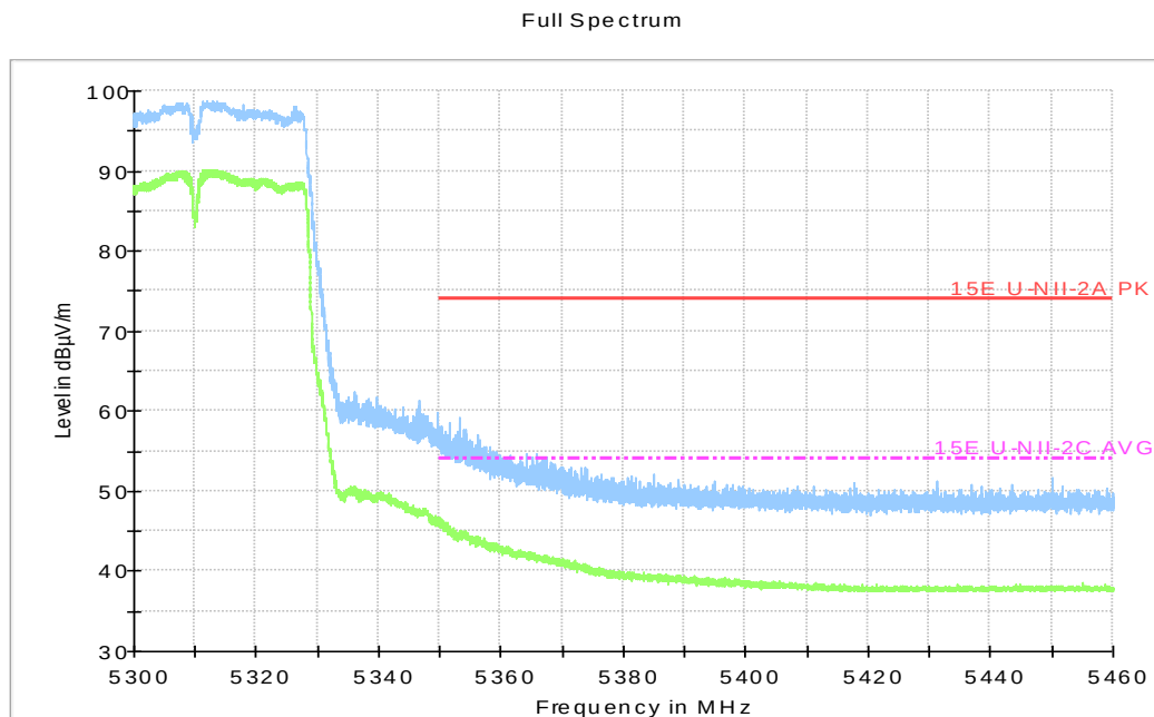
Fig.47 Band Edges (802.11ac-HT40, 5310MHz)
