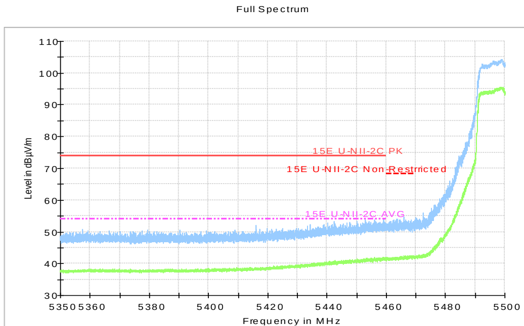
Fig.36 Band Edges (802.11n-HT20, 5500MHz)
