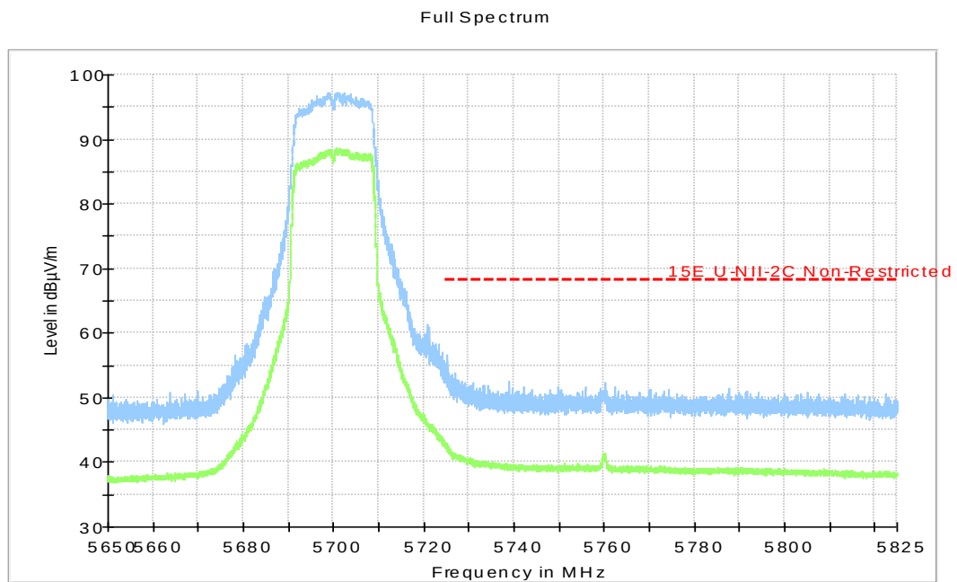
Fig.37 Band Edges (802.11n-HT20, 5700MHz)
