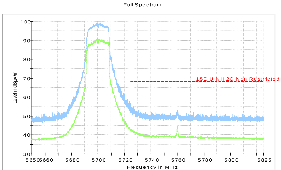
Fig.33 Band Edges (802.11a, 5700MHz)
