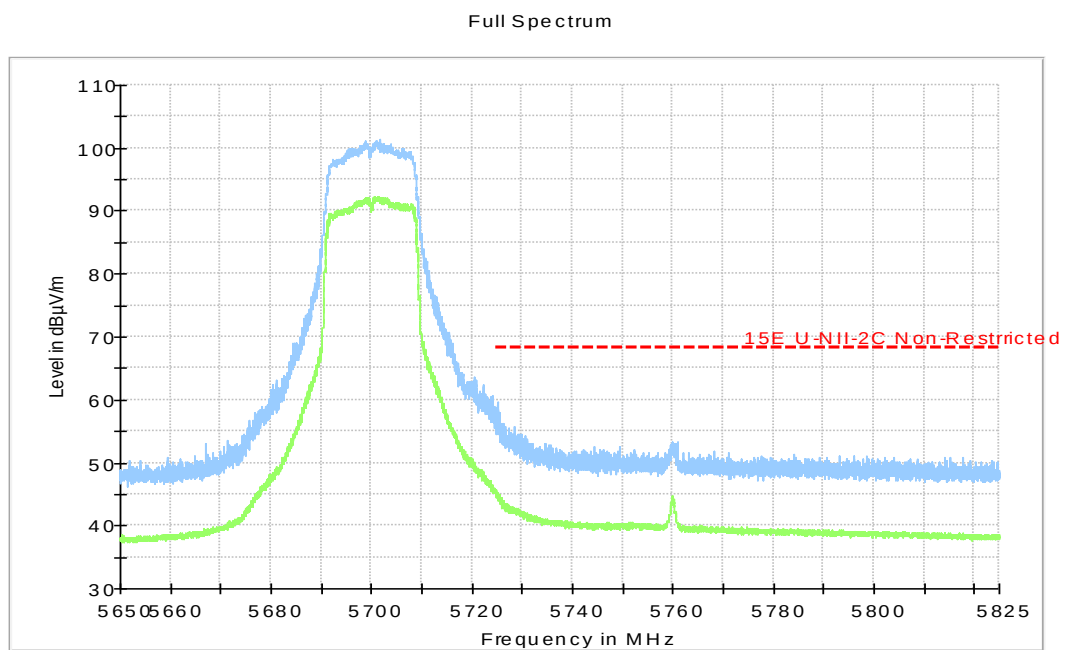
Fig.45 Band Edges (802.11ac-HT20, 5700MHz)
