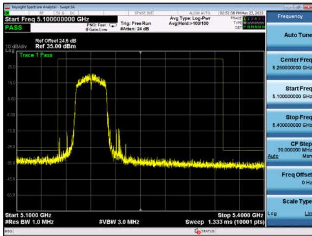
U-NII-1 ,802.11n-HT40, 5230MHz, Ant2
