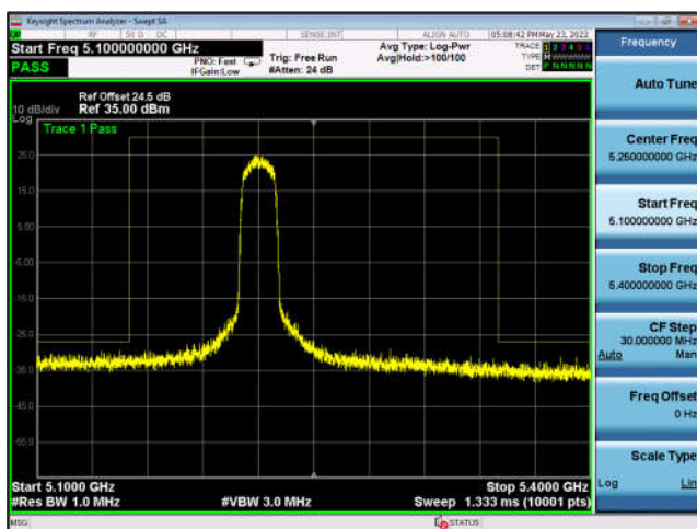
U-NII-1 ,802.11ac-VHT20, 5240MHz, Ant3
