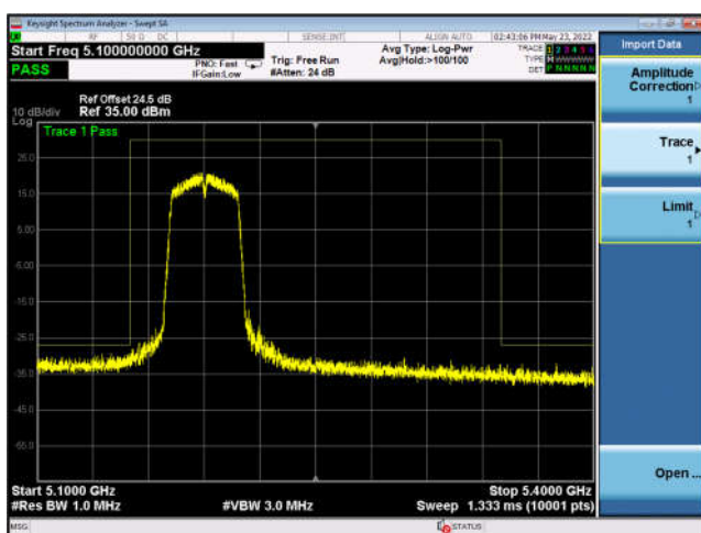
U-NII-1 ,802.11ac-VHT40, 5190MHz, Ant3
