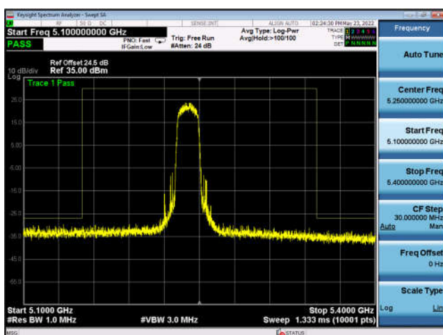
U-NII-1 ,802.11n-HT20, 5240MHz, Ant2
