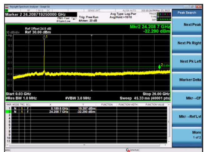
U-NII-1 ,802.11ac-VHT40, 5190MHz, Ant2
