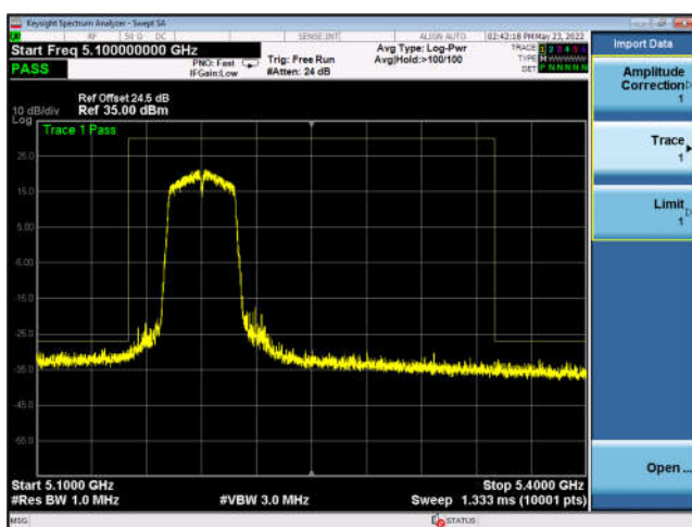
U-NII-1 ,802.11ac-VHT40, 5190MHz, Ant1
