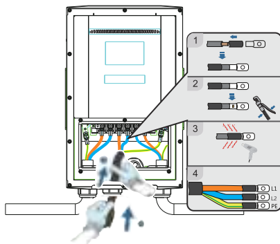
Dual Charge Coupler Input Wiring
