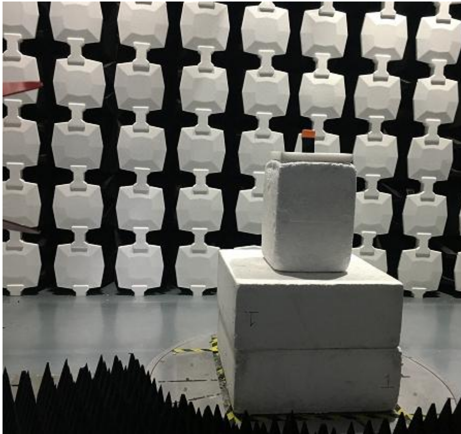
Description: Radiated Emission Test Setup (1 GHz -18GHz)
