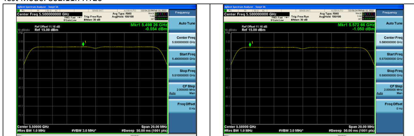
Test Mode:802.11n HT20 5500MHz Chain0
