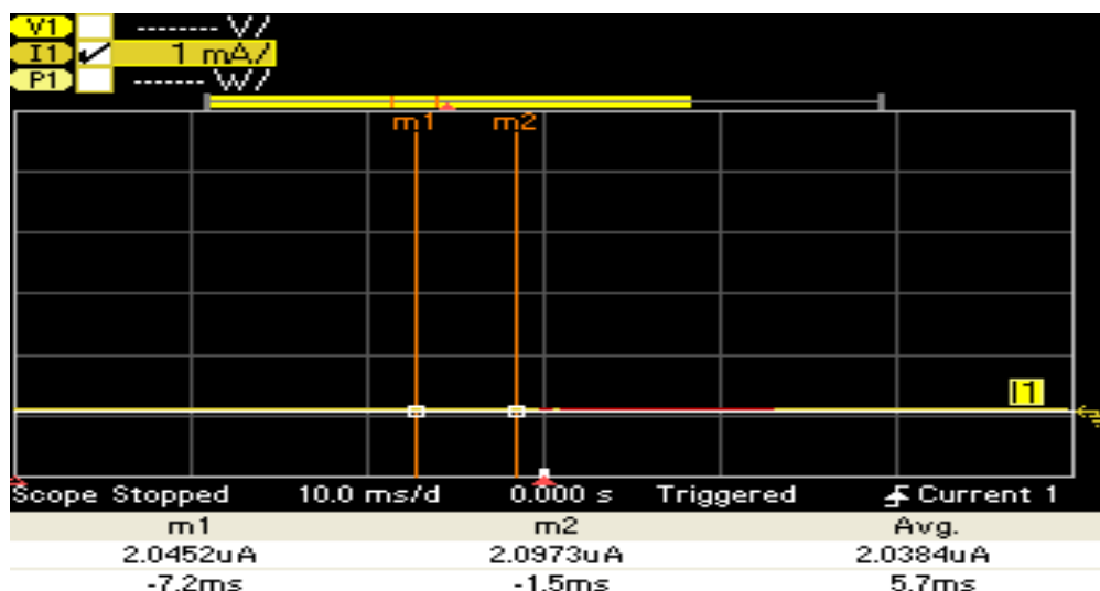
Figure 21: Supply current during Extended Sleep mode
