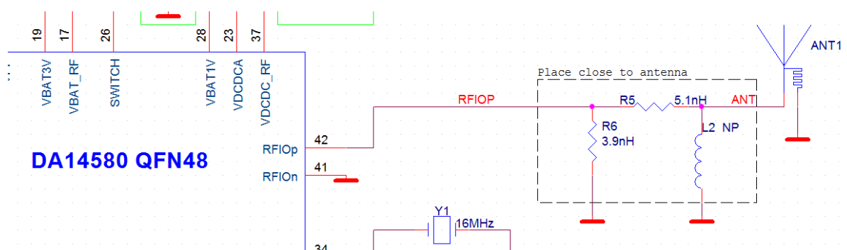
Figure 9: Matching network: R5 (5.1 nH) and R6 (3.9 nH)
