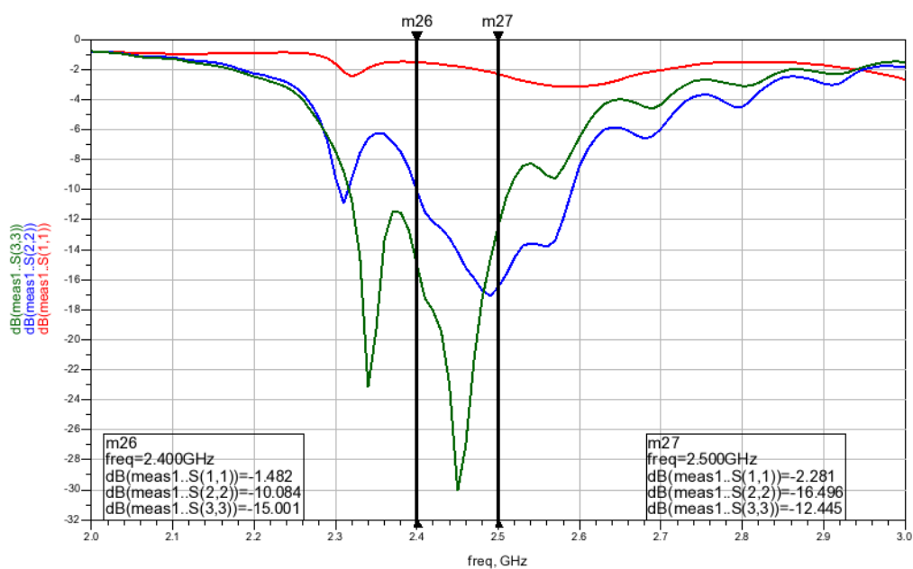
Figure 9: Matching network: R5 (5.1 nH) and R6 (3.9 nH)
