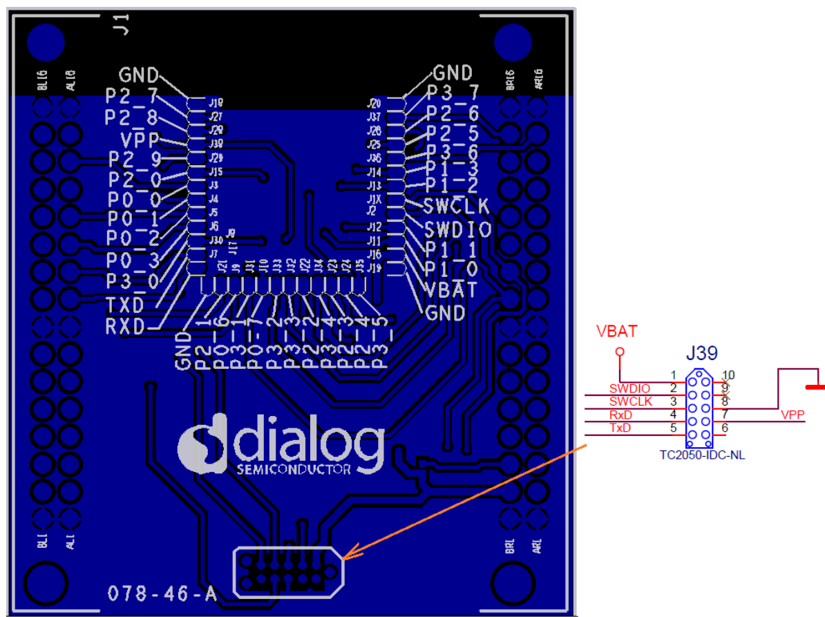
Figure 14: Interposer (078-46-A) for the QFN48 antenna module
