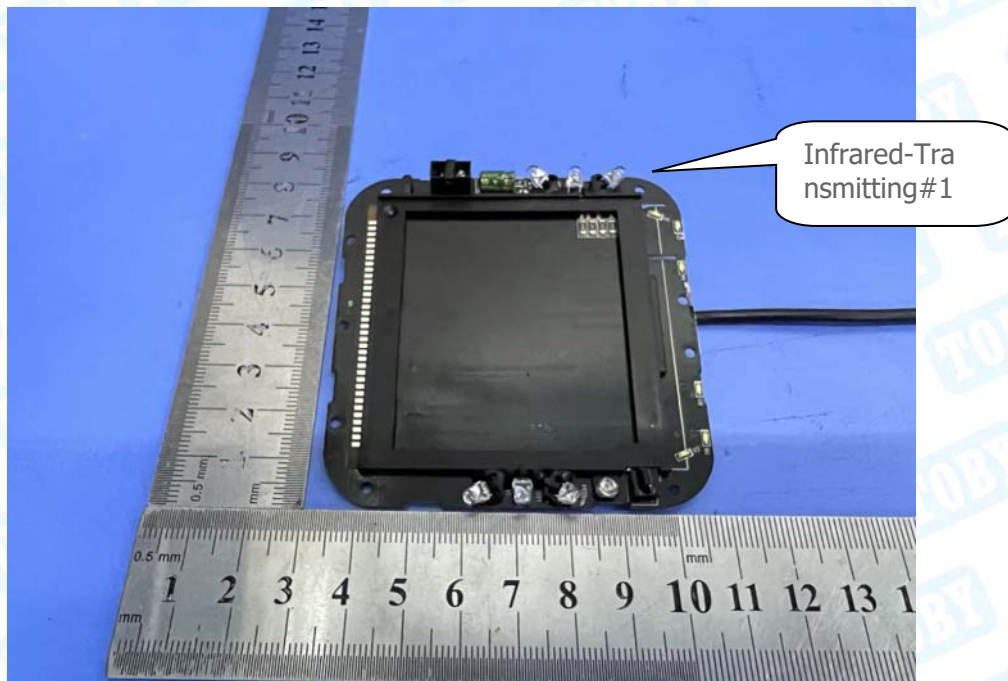
Photo 8 Internal of PCB
