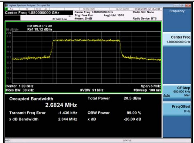
MCH_16QAM_15RB#0
