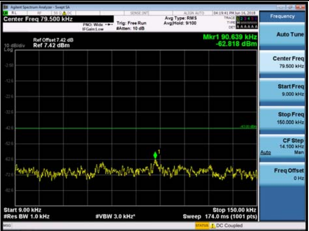
10MHz_LCH_QPSK_1RB#0
