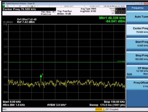
1.4MHz_LCH_QPSK_1RB#0
