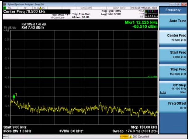
1.4MHz_LCH_QPSK_1RB#0
