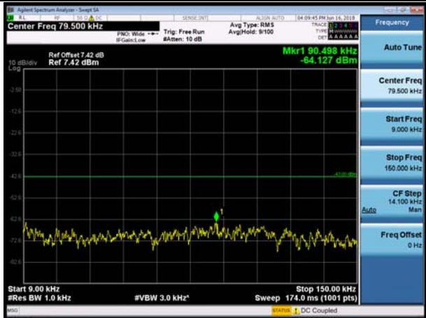
1.4MHz_LCH_QPSK_1RB#0
