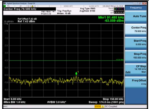
10MHz_LCH_QPSK_1RB#0
