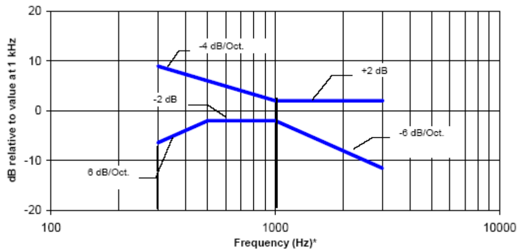
Figure 6.5-3 Magnetic field frequency response for WDs with a field strength of \leq -15 dB (A/m) at 1 kHz
