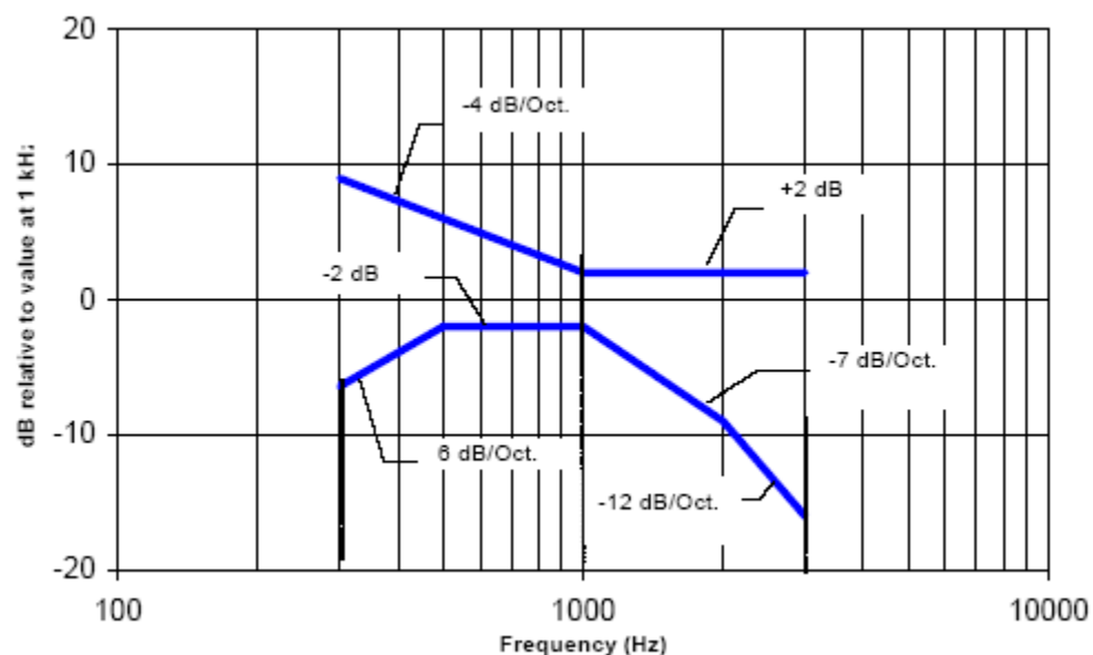
Figure 6.5-4 Magnetic field frequency response for WDs with a field strength that exceeds -15 dB(A/m) at 1 kHz
