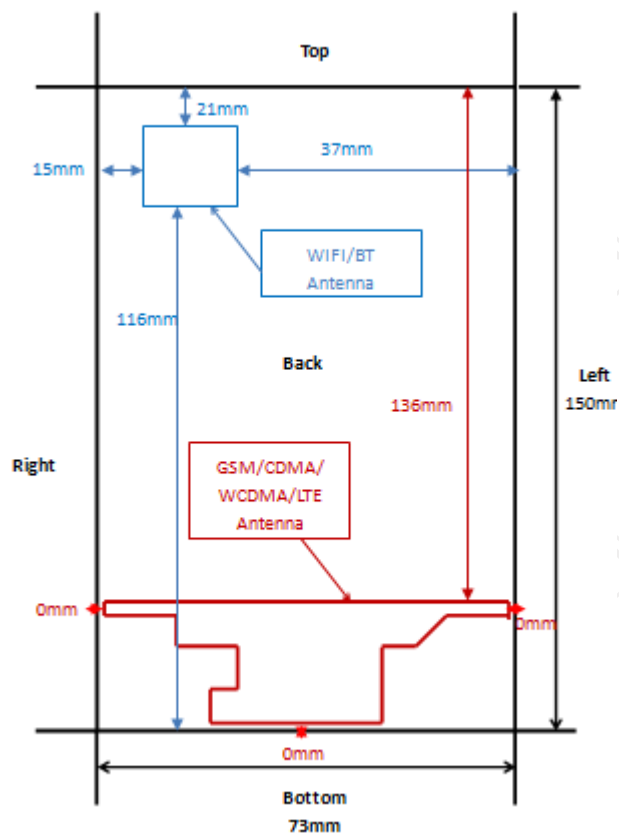
Antenna Configuration 1- LT60
