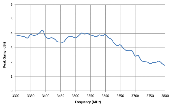
Peak Gain
