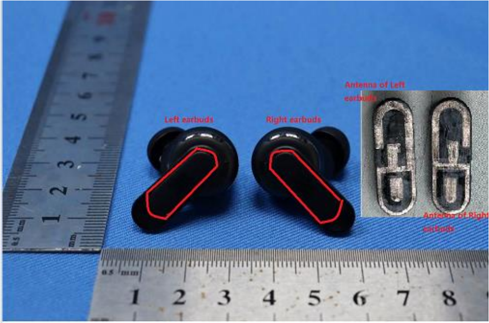
Antenna Location
