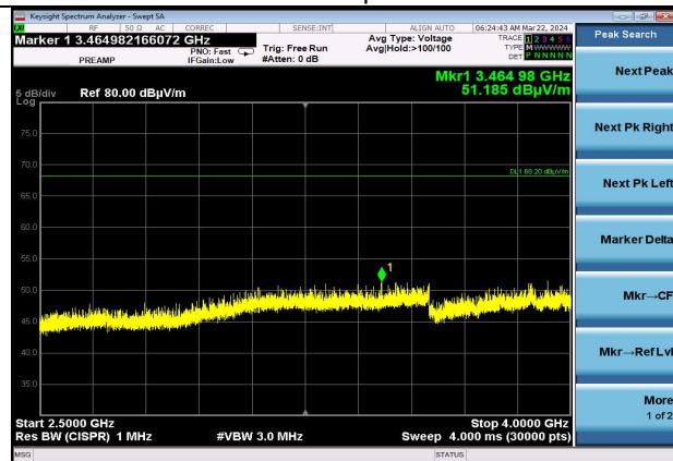
Channel 78 | Basic Rate | Single 2500-4000 MHz | Horizontal
