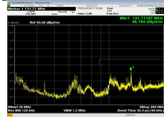
Channel 39 | Basic Rate | Single 30-200 MHz | Vertical
