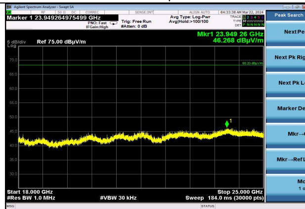
Channel 39 | Basic Rate | Single 18000-25000 MHz | Horizontal
