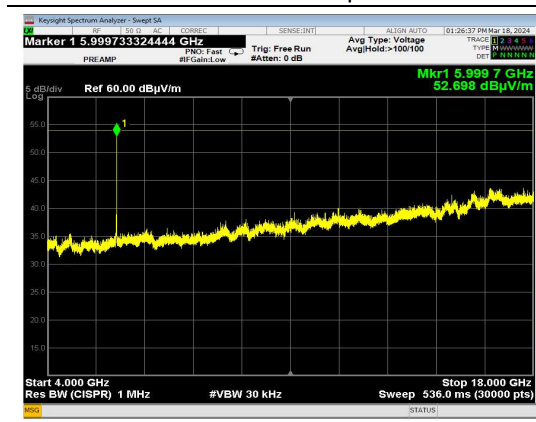
Channel 39 | Basic Rate | Single 4000-18000 MHz | Vertical
