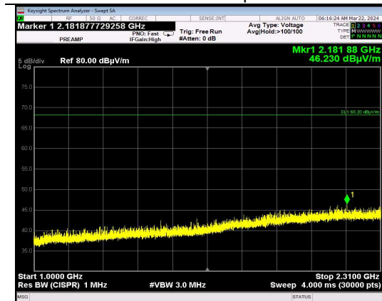
Channel 0 | Basic Rate | Single 1000-2310 MHz | Horizontal
