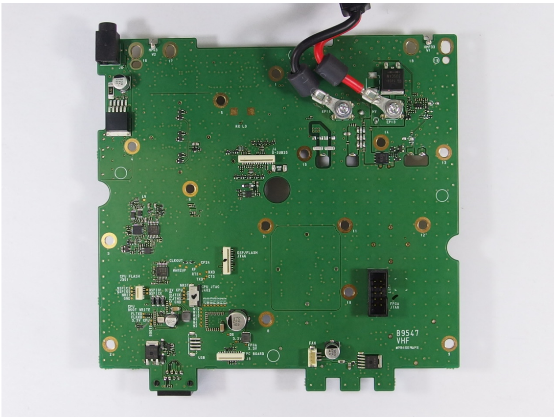
MAIN UNIT MAIN BOARD SIDE-A
