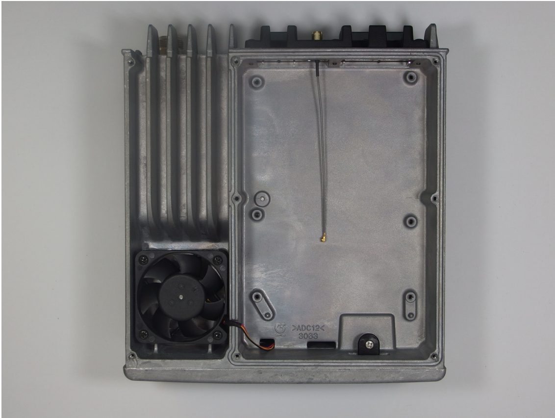
MAIN UNIT TOP IN SIDE
