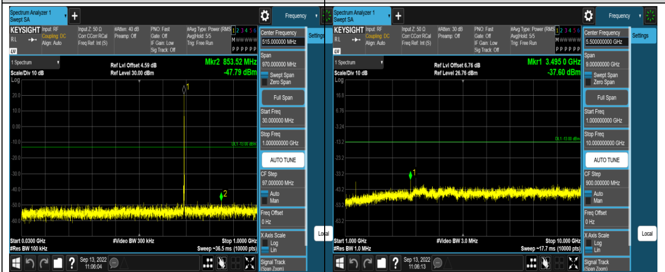
Band12-1.4MHz-16QAM-23017-1RB#0-Range1:30~1000MHz
