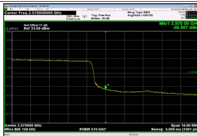
HighRange_FDD07_15MHz_2562.5_fullRB _HighQPSK
