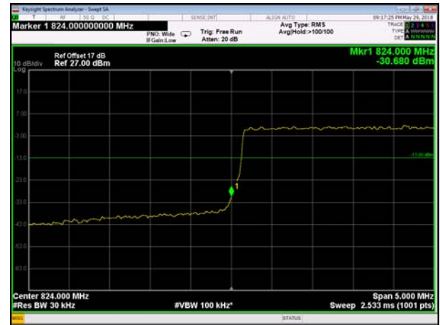
LowRange_FDD05_5MHz_826.5_OneRB _low_Q16
