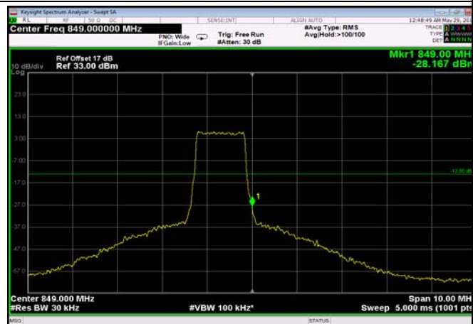
HighRange_FDD05_3MHz_847.5_OneRB _high_Q16 06
