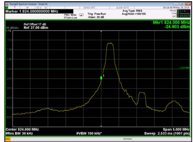
LowRange_FDD05_1.4MHz_824.7_fullRB _LowQ16
