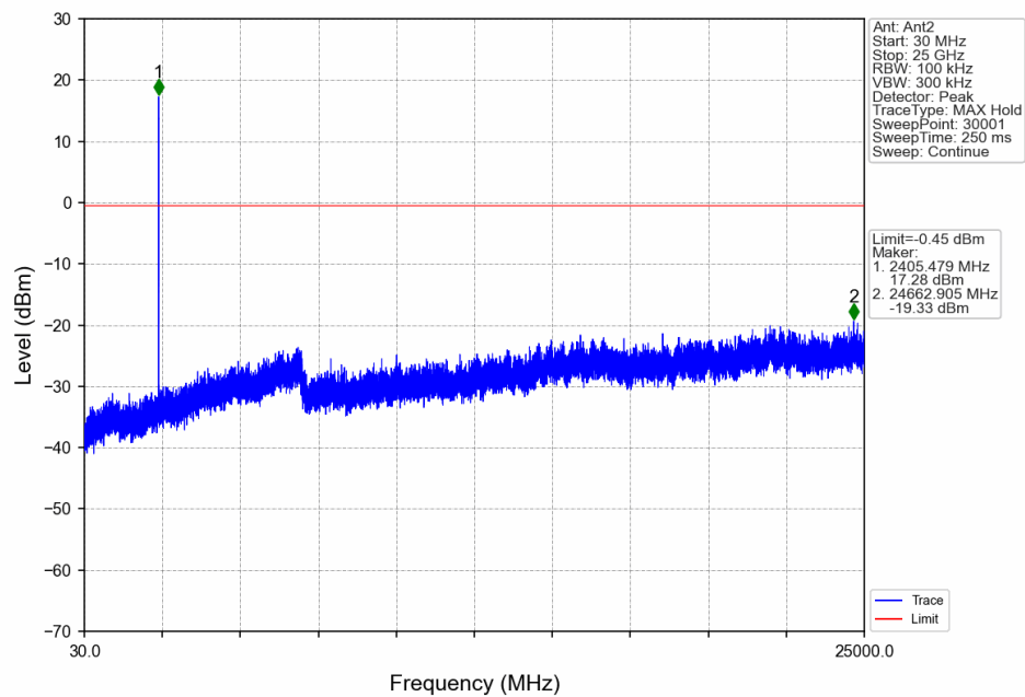
Slot5_LCH_2405MHz_Ant2_NTNV
