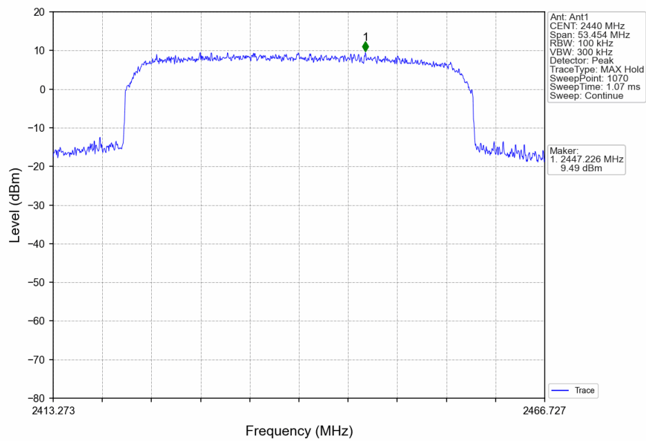
Slot40_MCH_2440MHz_Ant1_NTNV
