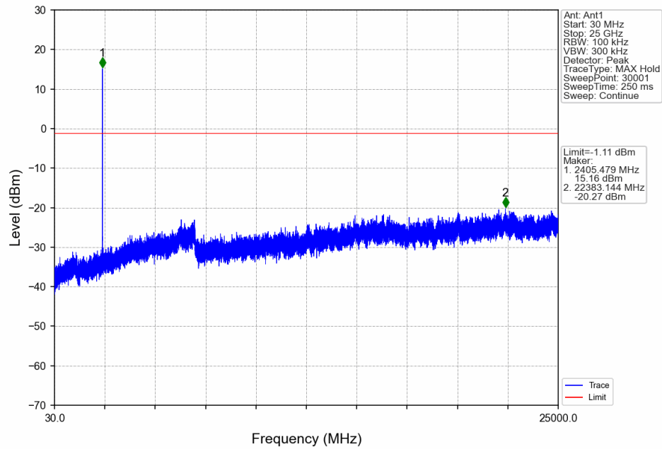
Slot5_LCH_2405MHz_Ant1_NTNV
