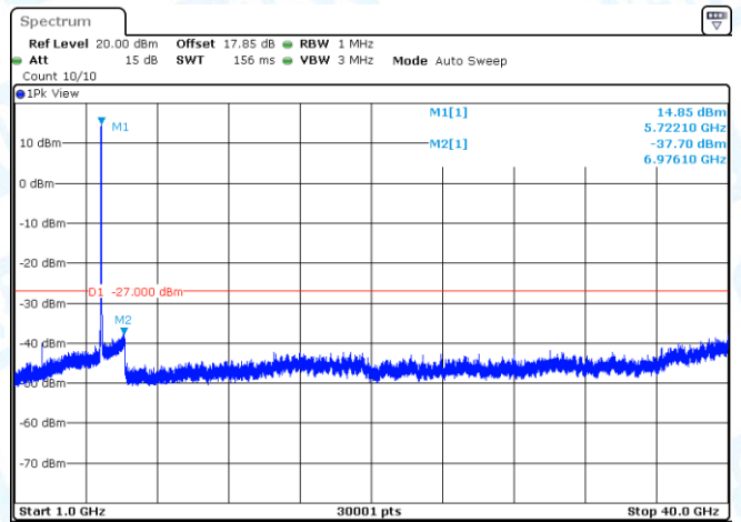
11N20MIMO-Ant1-5720-1000~40000-PASS
