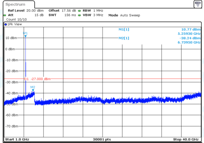
11AC20MIMO-Ant1-5260-1000~40000-PASS
