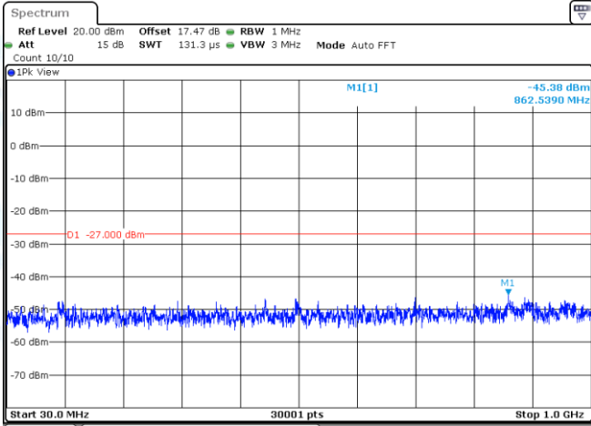
11AC20MIMO-Ant1-5260-30~1000-PASS
