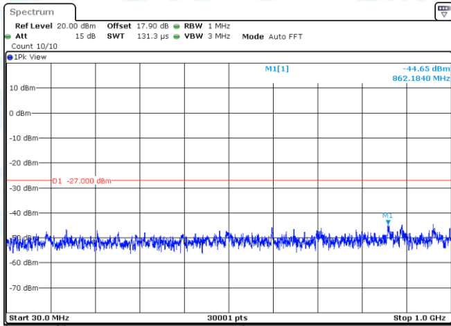
11N20MIMO-Ant2-5580-30~1000-PASS
