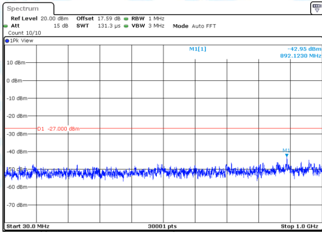
11N20MIMO-Ant2-5500-30~1000-PASS
