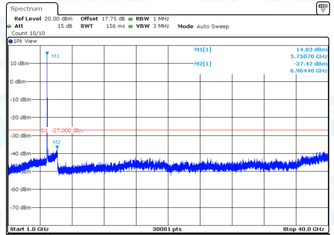
11N20MIMO-Ant1-5745-1000~40000-PASS
