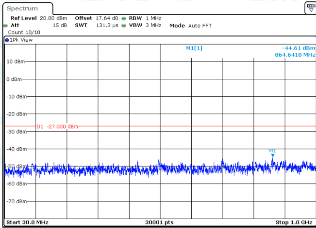
11N20MIMO-Ant1-5500-30~1000-PASS
