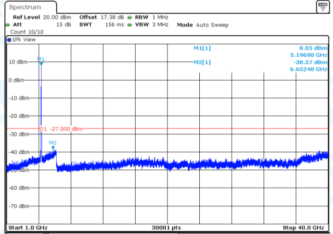
11N40MIMO-Ant1-5190-1000~40000-PASS
