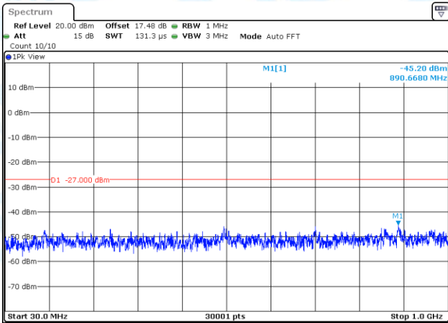
11N40MIMO-Ant2-5190-30~1000-PASS
