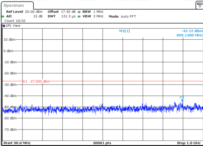
11AC20MIMO-Ant2-5260-30~1000-PASS
