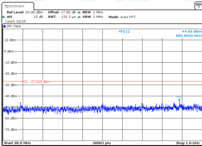
11N20MIMO-Ant1-5720-30~1000-PASS
