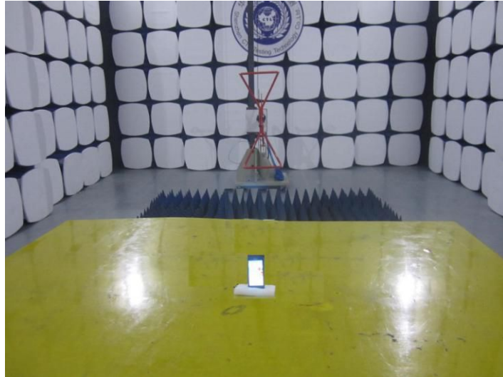
Test Setup Photos of the EUT_PCE
