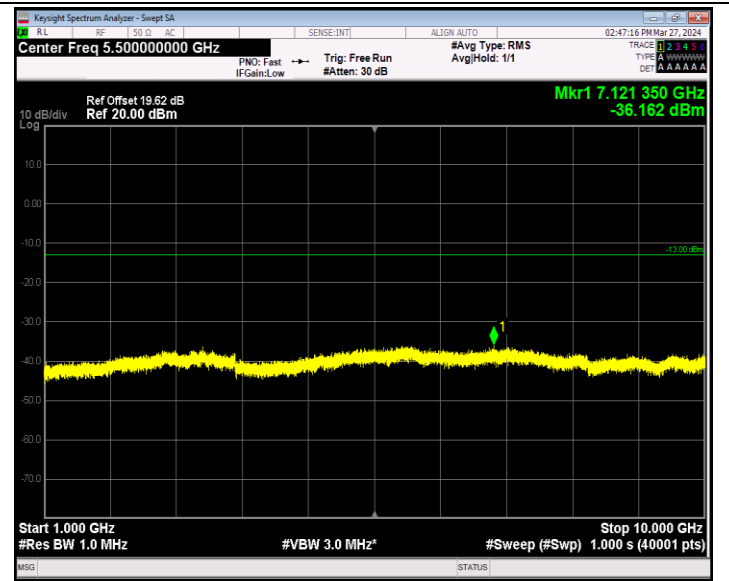
Band5_1.4MHz_QPSK_20407_1RB#0_1000~10000_1000~1000 0
