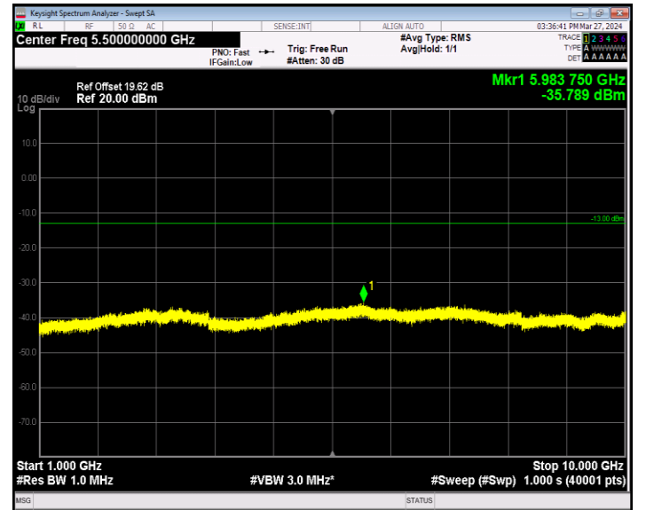
Band5_10MHz_16QAM_20525_1RB#0_1000~10000_1000~1000 0
