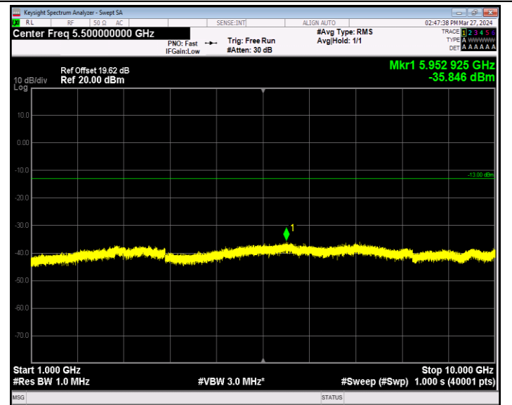
Band5_1.4MHz_16QAM_20407_1RB#0_1000~10000_1000~1000 00
