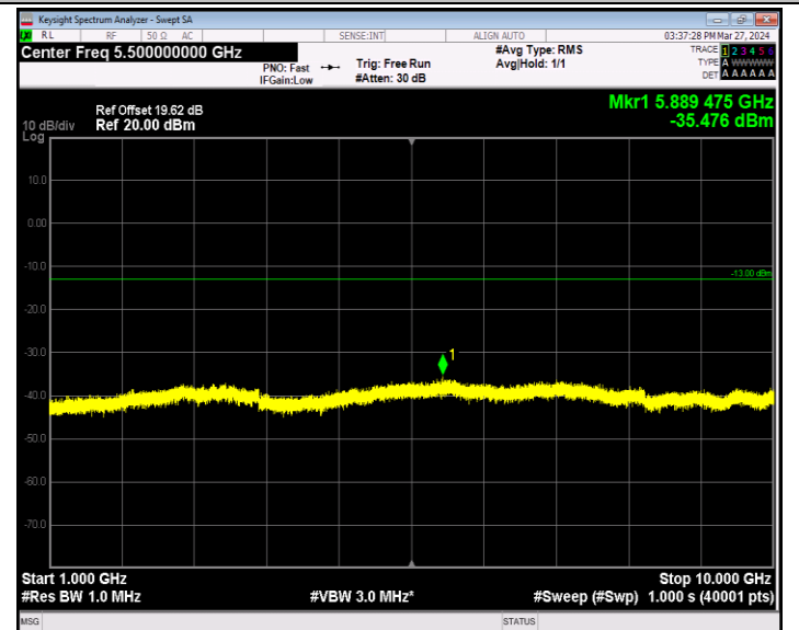
Band5_10MHz_QPSK_20600_1RB#0_1000~10000_1000~10000
