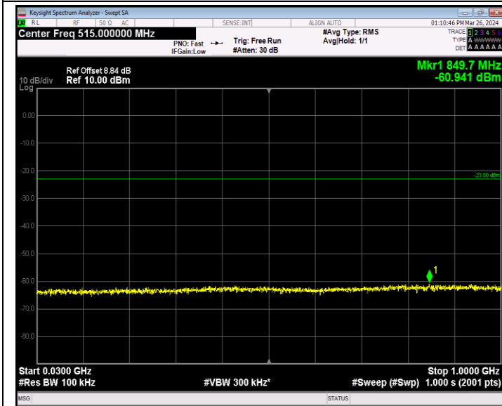
Band2_20MHz_64QAM_18700_1RB#0_30~1000_30~1000
