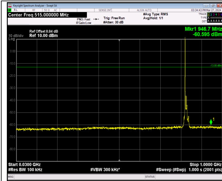
Band5_10MHz_16QAM_20450_1RB#0_30~1000_30~1000
