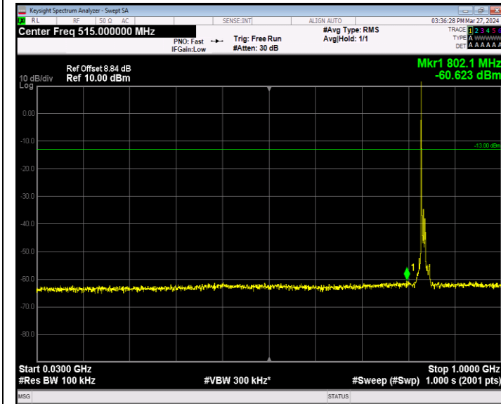
Band5_10MHz_16QAM_20525_1RB#0_30~1000_30~1000
