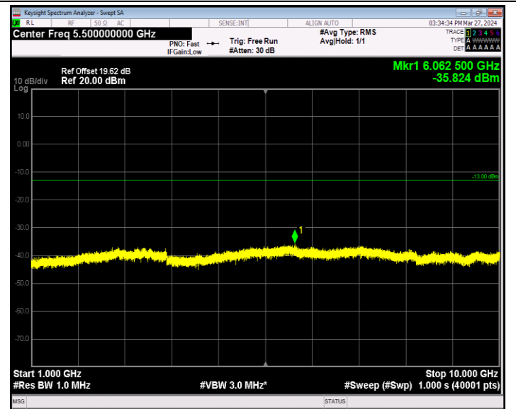
Band5_10MHz_QPSK_20450_1RB#0_1000~10000_1000~10000
