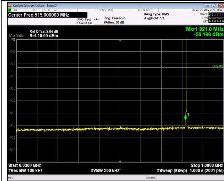
Band5_1.4MHz_16QAM_20407_1RB#0_30~1000_30~1000
