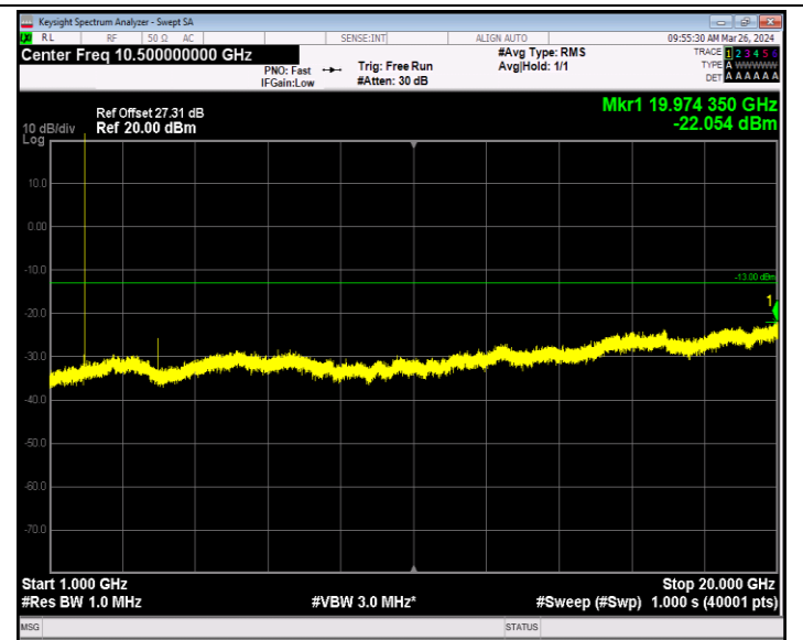
Band2_1.4MHz_64QAM_19193_1RB#0_1000~20000_1000~2000
