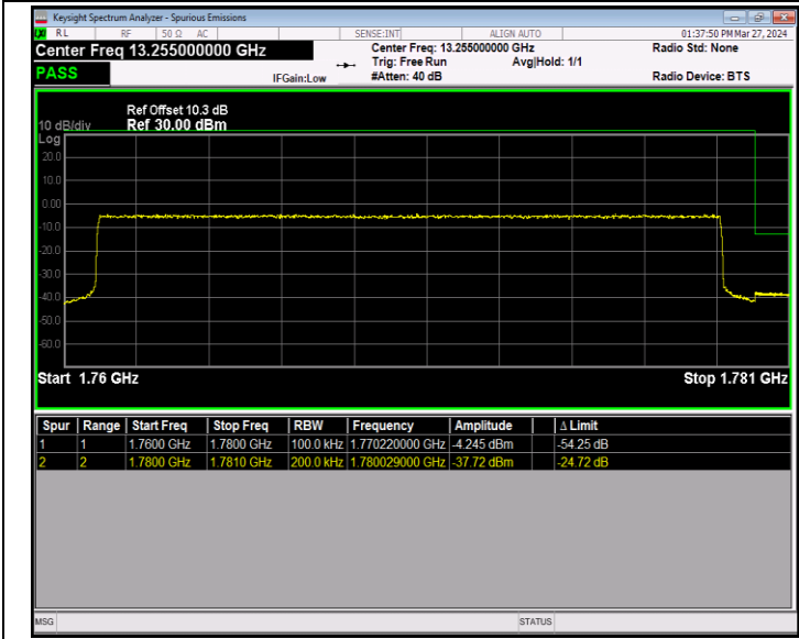
Band66_20MHz_64QAM_132572_100RB#0
