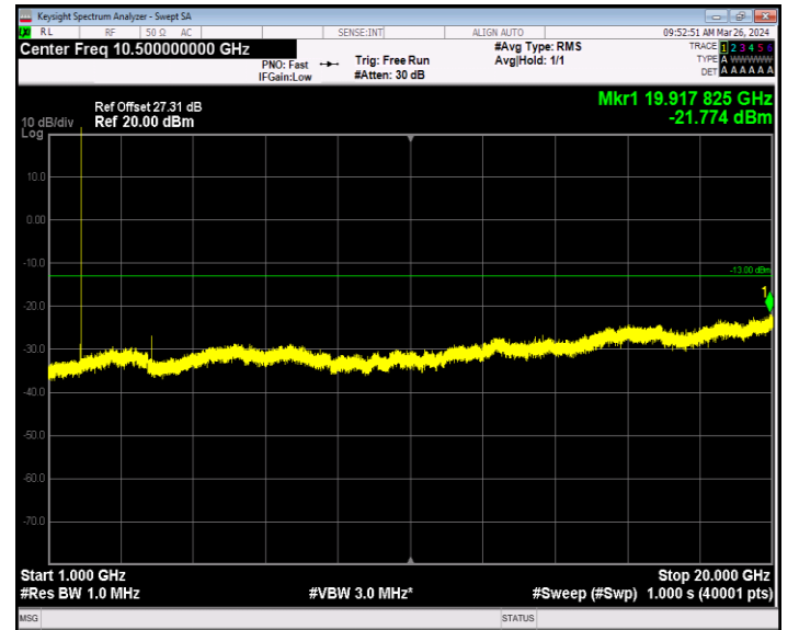
Band2_1.4MHz_16QAM_18607_1RB#0_1000~20000_1000~2000 00
