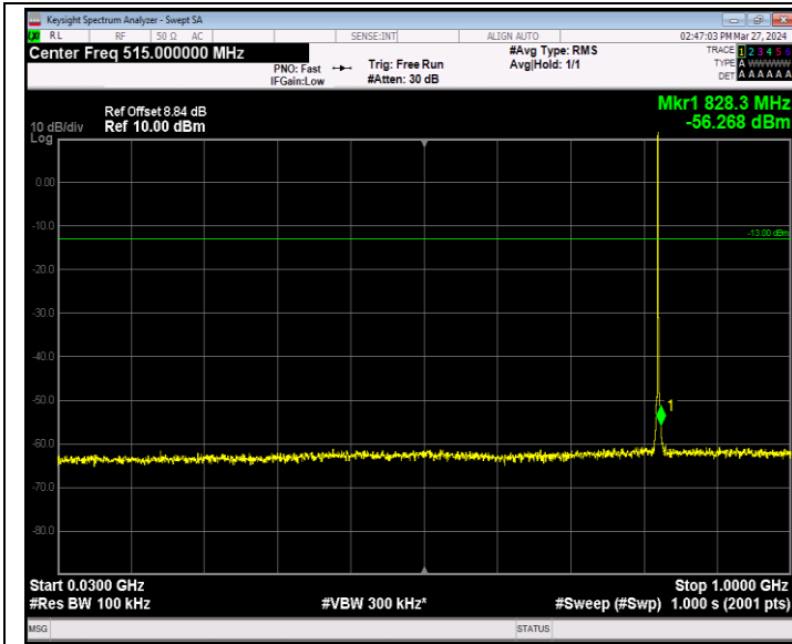
Band5_1.4MHz_QPSK_20407_1RB#0_30~1000_30~1000
