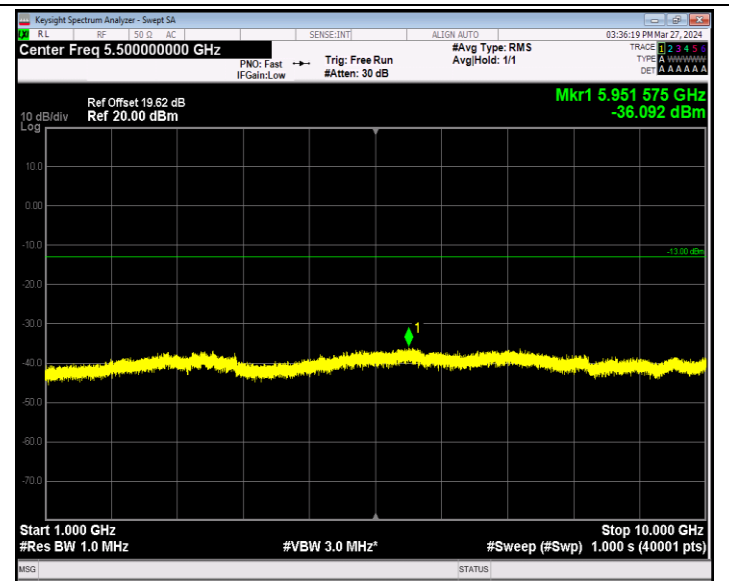
Band5_10MHz_QPSK_20525_1RB#0_1000~10000_1000~10000
