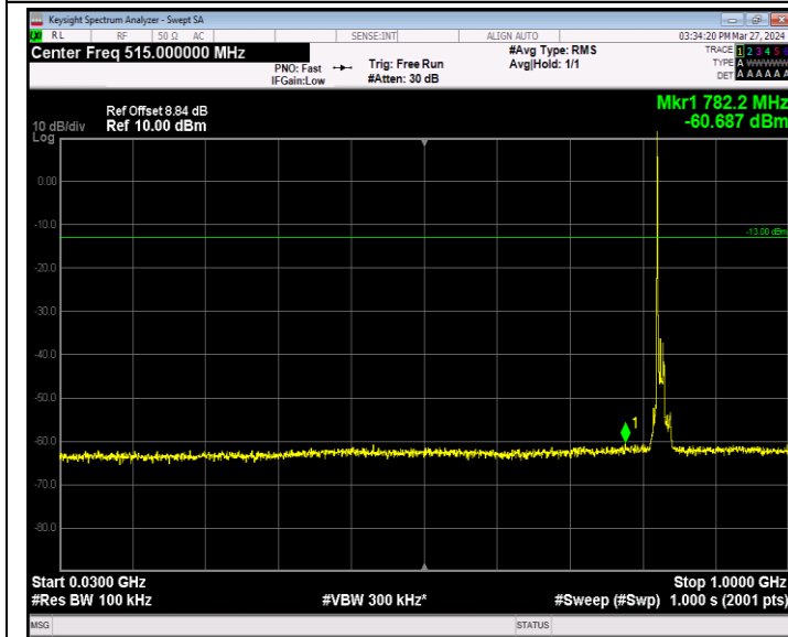
Band5_10MHz_QPSK_20450_1RB#0_30~1000_30~1000
