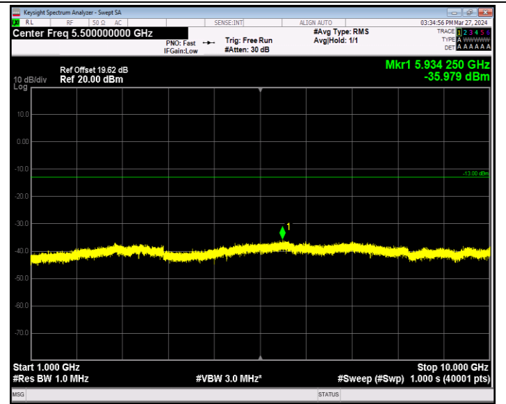
Band5_10MHz_16QAM_20450_1RB#0_1000~10000_1000~1000 0
