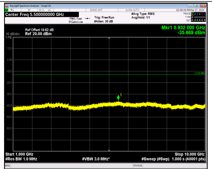
Band5_1.4MHz_16QAM_20525_1RB#0_1000~10000_1000~10000
