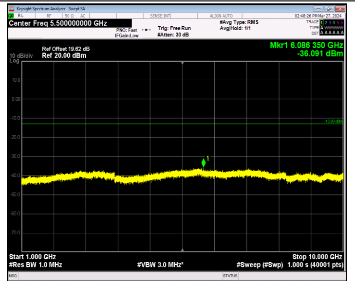
Band5_1.4MHz_QPSK_20525_1RB#0_1000~10000_1000~1000 0
