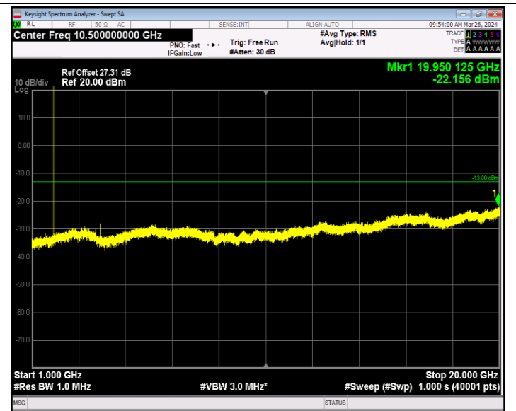
Band2_1.4MHz_16QAM_18900_1RB#0_1000~20000_1000~20000
