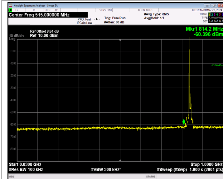
Band5_10MHz_QPSK_20600_1RB#0_30~1000_30~1000
