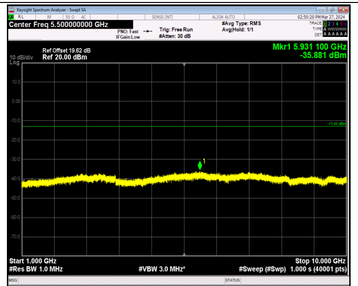
Band5_1.4MHz_64QAM_20643_1RB#0_1000~10000_1000~10000
