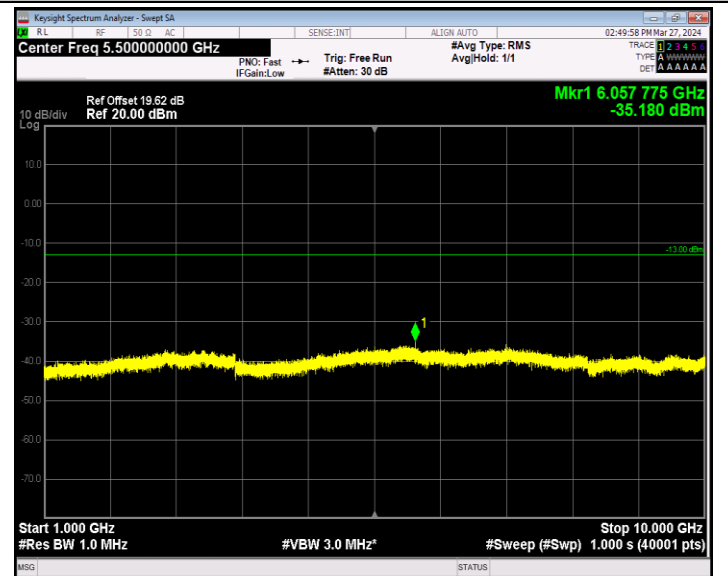
Band5_1.4MHz_16QAM_20643_1RB#0_1000~10000_1000~10000
