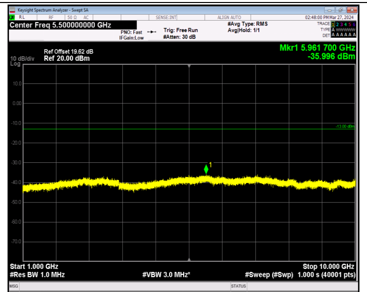
Band5_1.4MHz_64QAM_20407_1RB#0_1000~10000_1000~10000
