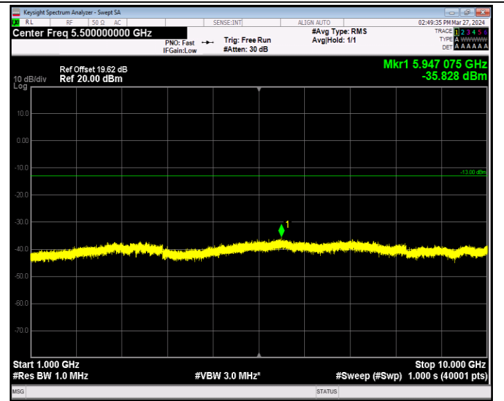
Band5_1.4MHz_QPSK_20643_1RB#0_1000~10000_1000~1000 0
