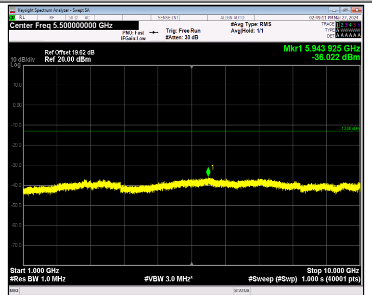
Band5_1.4MHz_64QAM_20525_1RB#0_1000~10000_1000~10000
