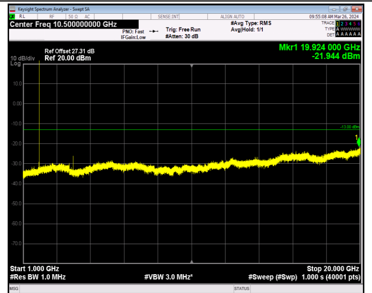
Band2_1.4MHz_16QAM_19193_1RB#0_1000~20000_1000~20000
