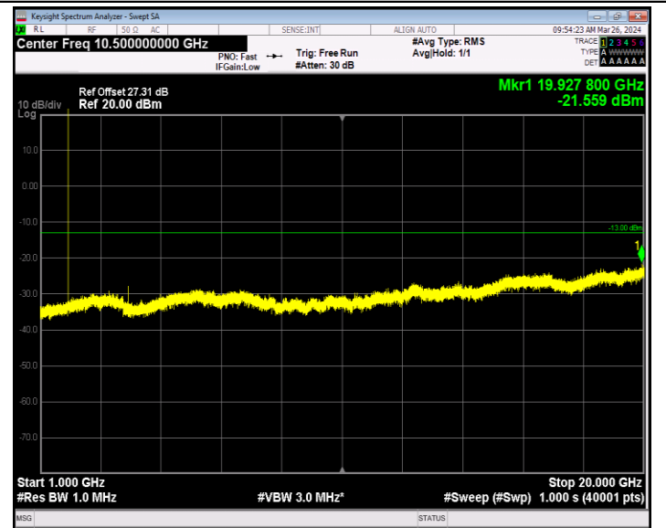
Band2_1.4MHz_64QAM_18900_1RB#0_1000~20000_1000~2000 00
