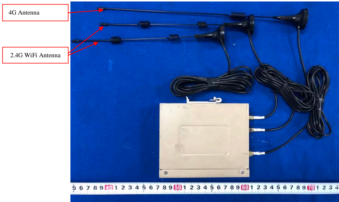
All View
