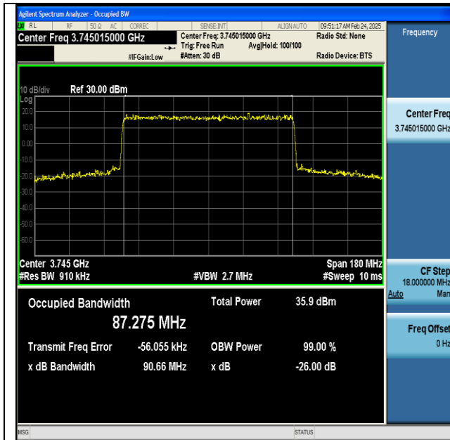
NTNV-n77(3700-3980)-PC2-30-90-L-CP-16QAM- Outer_Full-Ant1-PASS
