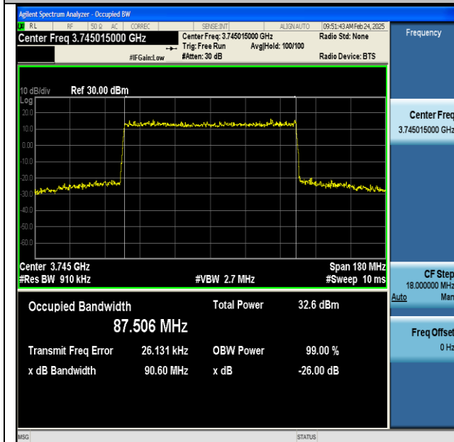
NTNV-n77(3700-3980)-PC2-30-90-L-CP-256QAM- Outer_Full-Ant1-PASS
