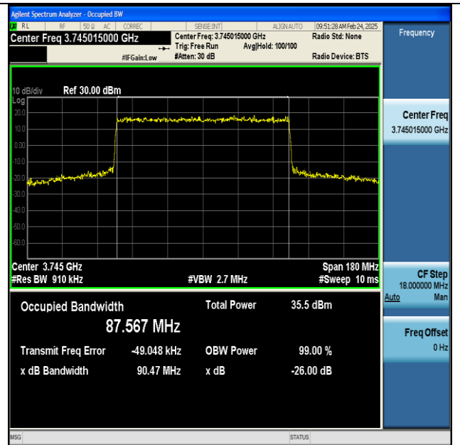
NTNV-n77(3700-3980)-PC2-30-90-L-CP-64QAM- Outer_Full-Ant1-PASS
