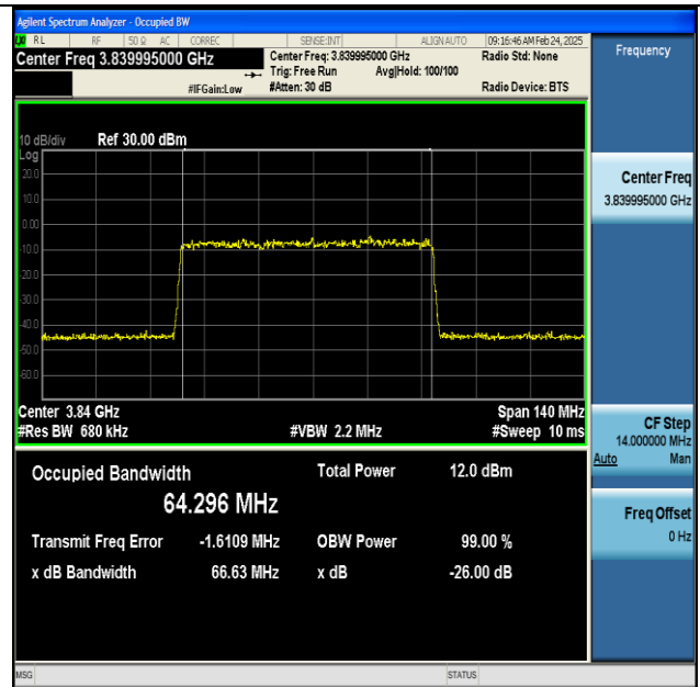
NTNV-n77(3700-3980)-PC2-30-70-M-DFT-BPSK- Outer_Full-Ant1-PASS
