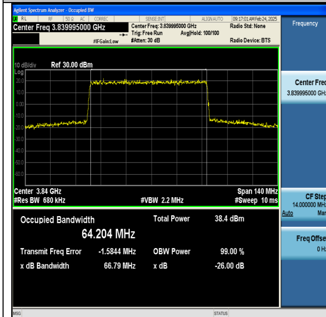
NTNV-n77(3700-3980)-PC2-30-70-M-DFT-QPSK- Outer_Full-Ant1-PASS
