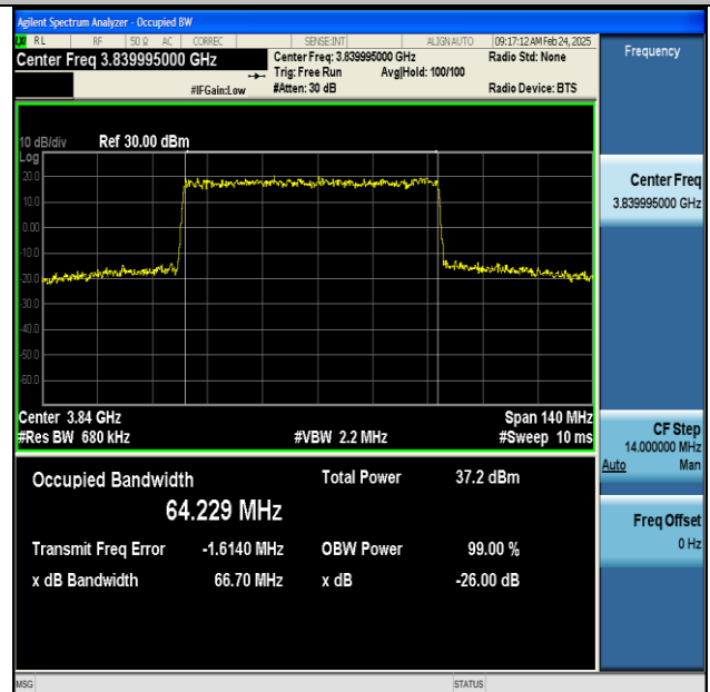
NTNV-n77(3700-3980)-PC2-30-70-M-DFT-16QAM- Outer_Full-Ant1-PASS
