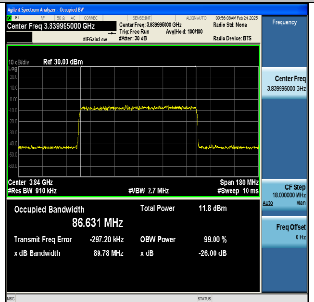
NTNV-n77(3700-3980)-PC2-30-90-M-DFT-BPSK- Outer_Full-Ant1-PASS
