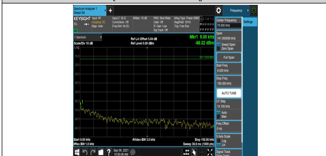
Band2-20MHz-16QAM-18700-1RB#0-Range1:0.009~0.15MHz
