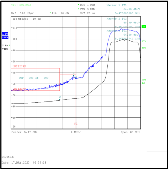
Lower Band Edge (CH100)
