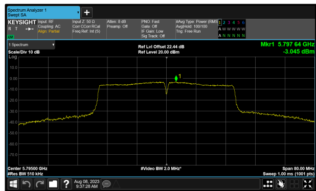
SP1-C0 5795 MHz (CH159)
