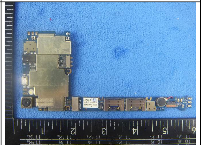
Mainboard with Shielding - Front View 2
