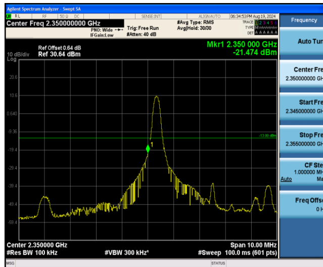
Band40-5MHz-16QAM-39175-1RB#24
