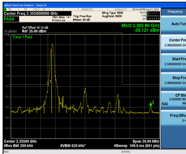
Band40-10MHz-16QAM-39200-1RB#49
