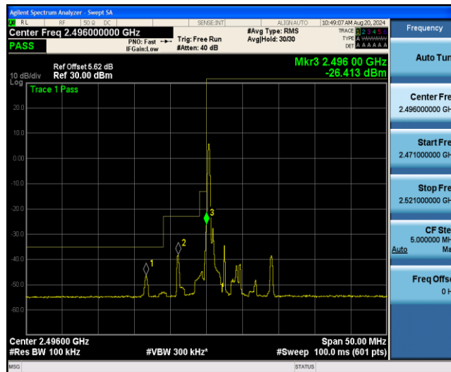
Band41-5MHz-16QAM-39675-1RB#24
