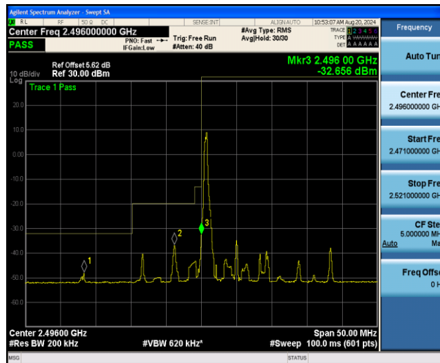
Band41-10MHz-QPSK-39700-1RB#49
