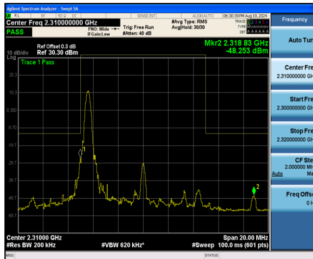
Band40-10MHz-QPSK-38750-1RB#49
