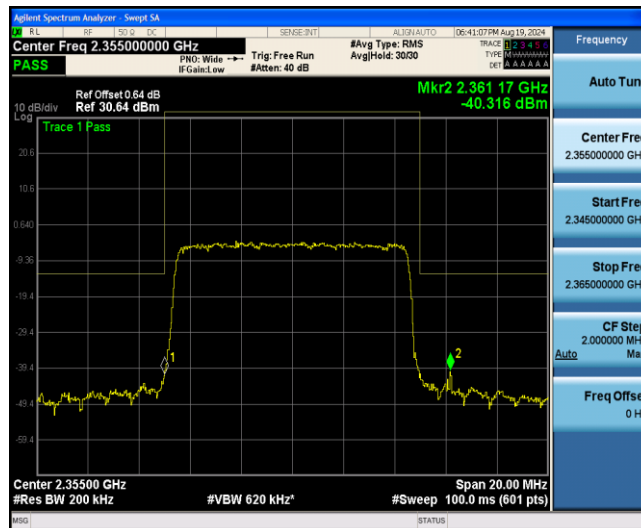
Band40-10MHz-QPSK-39200-1RB#49
