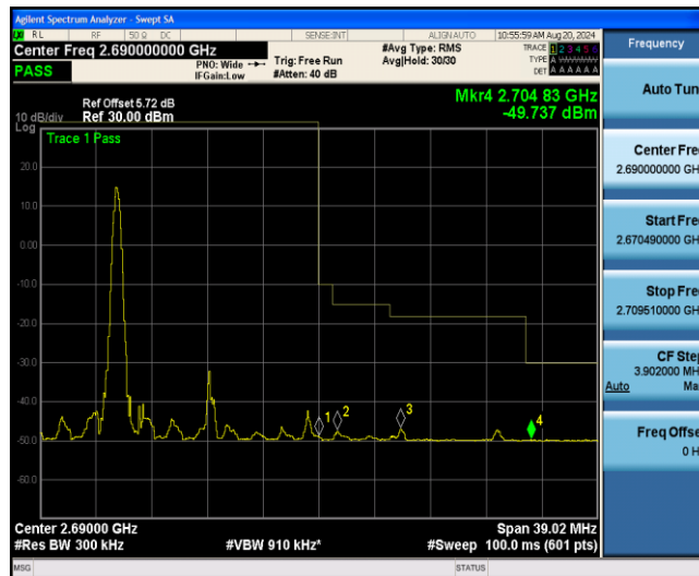
Band41-15MHz-QPSK-41515-1RB#74
