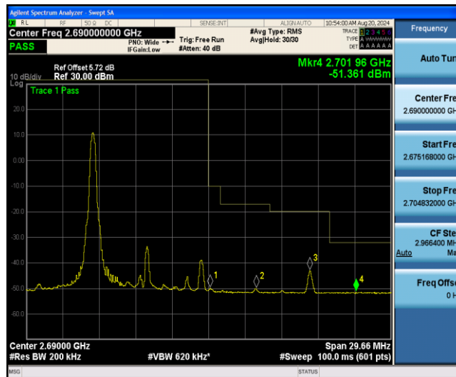
Band41-10MHz-QPSK-41540-1RB#49
