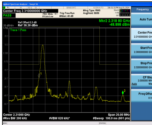
Band40-10MHz-16QAM-38750-1RB#49
