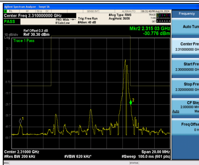
Band40-10MHz-16QAM-38750-27RB#0
