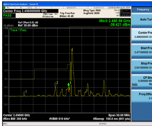
Band41-15MHz-QPSK-39725-1RB#74
