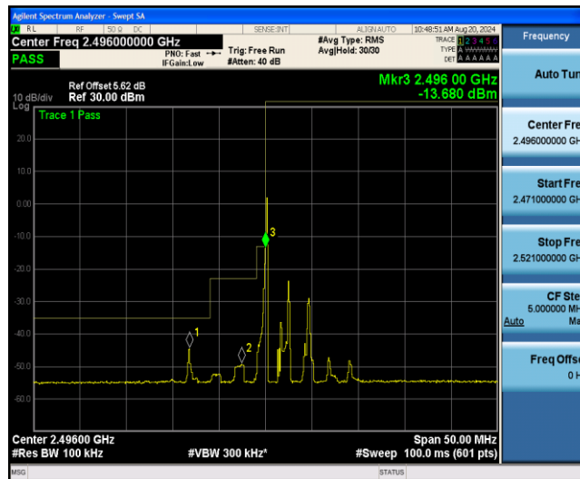
Band41-5MHz-QPSK-39675-1RB#24
