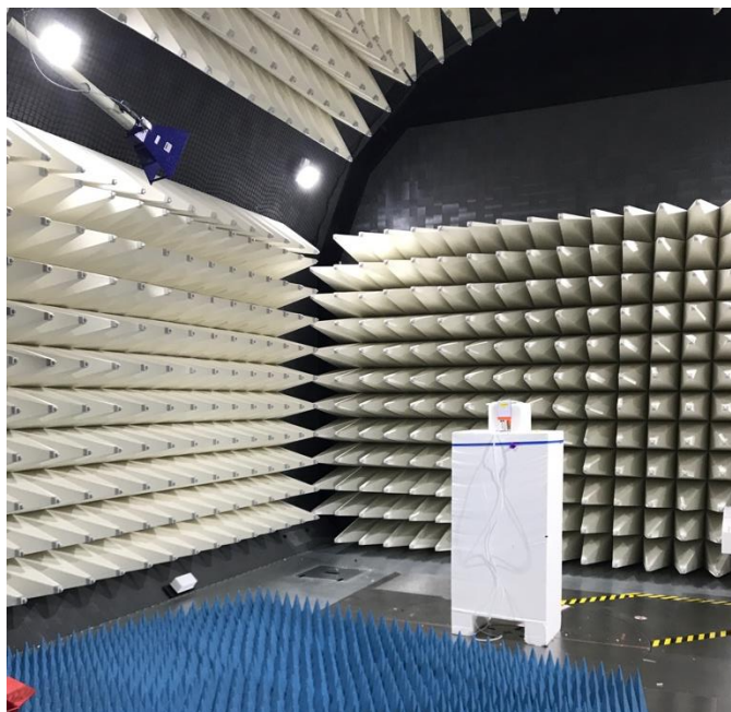
Photograph 2: Side View Test Set Up Radiated Emissions 1 – 17 GHz
