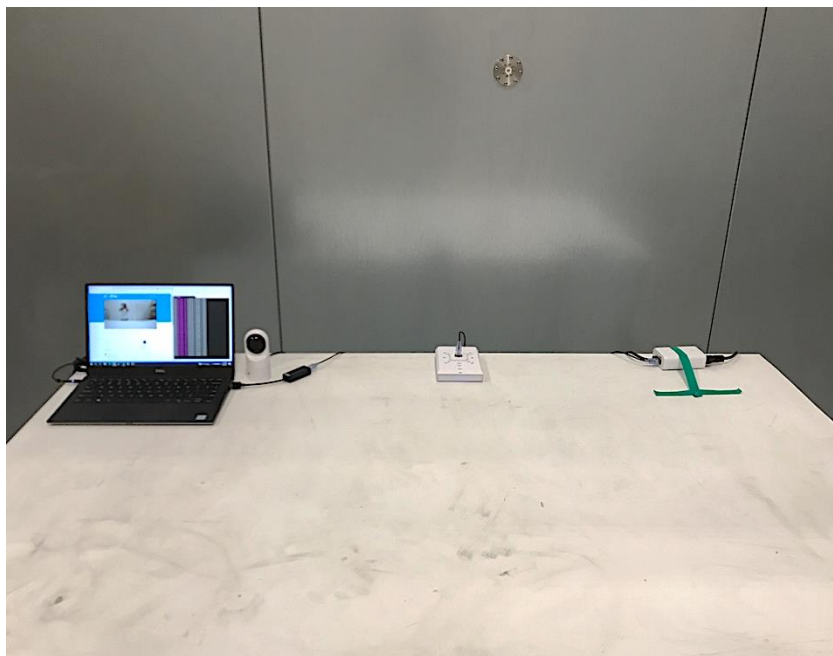
Photograph 4: Front View Test Set Up Conducted Emissions
