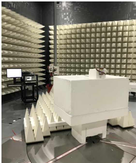
Photograph 3: Back View Test Set Up Radiated Emissions 17 – 40 GHz
