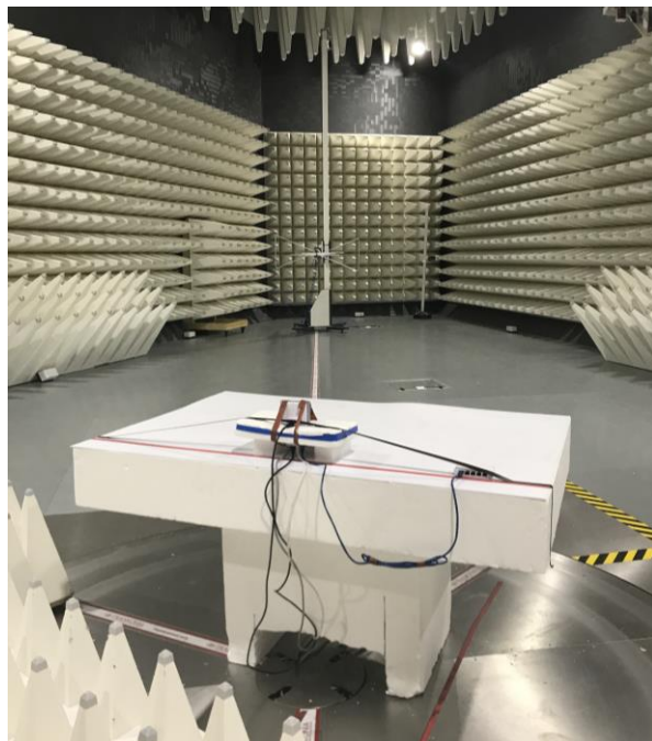
Photograph 1: Back View Test Set Up Radiated Emissions 30 – 1000 MHz
