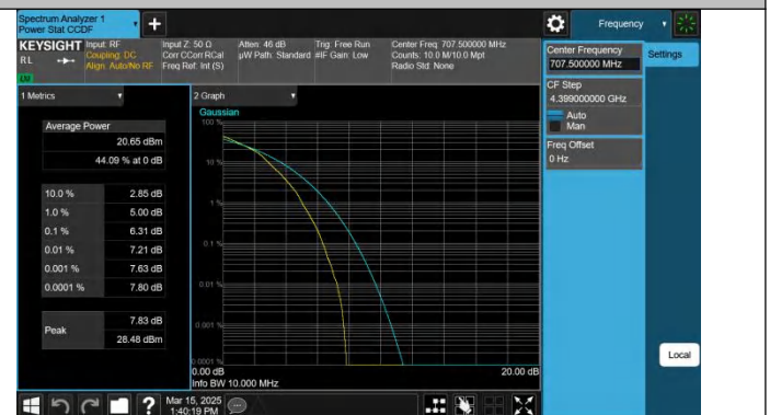
Band12-10MHz-16QAM-23095-27RB#0-PASS
