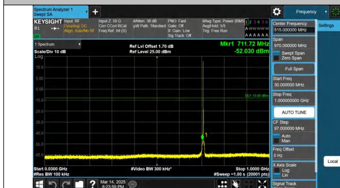
Band12-1.4MHz-QPSK-23173-1RB#0-30~1000-PASS
