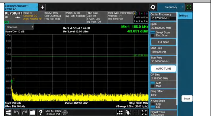
Band12-1.4MHz-QPSK-23173-1RB#0-0.15~30-PASS
