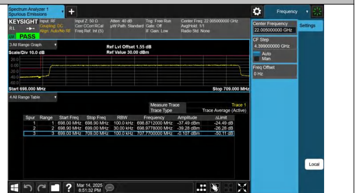
Band12-10MHz-QPSK-23060-50RB#0-PASS
