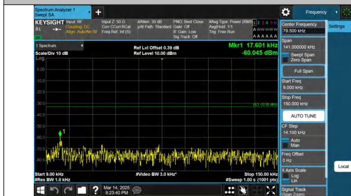
Band12-1.4MHz-QPSK-23173-1RB#0-0.009~0.15-PASS
