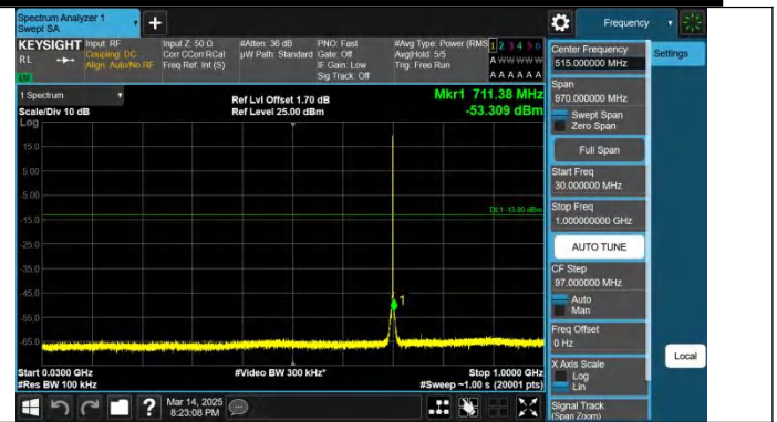
Band12-1.4MHz-QPSK-23095-1RB#5-30~1000-PASS
