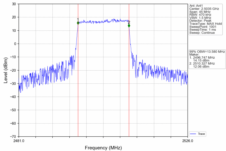
Band41_15MHz_16QAM_LCH_2503.5MHz_RB_75_0_NTNV
