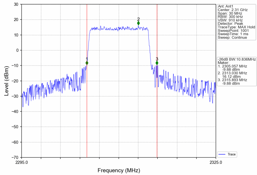
Band40a_10MHz_16QAM_HCH_2310MHz_RB_50_0_NTNV
