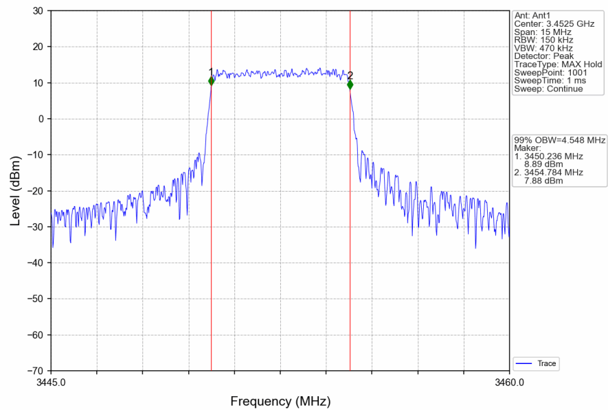
Band42a_5MHz_16QAM_LCH_3452.5MHz_RB_25_0_NTNV
