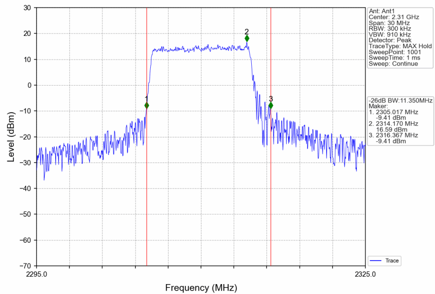
Band40a_10MHz_16QAM_HCH_2310MHz_RB_50_0_NTNV
