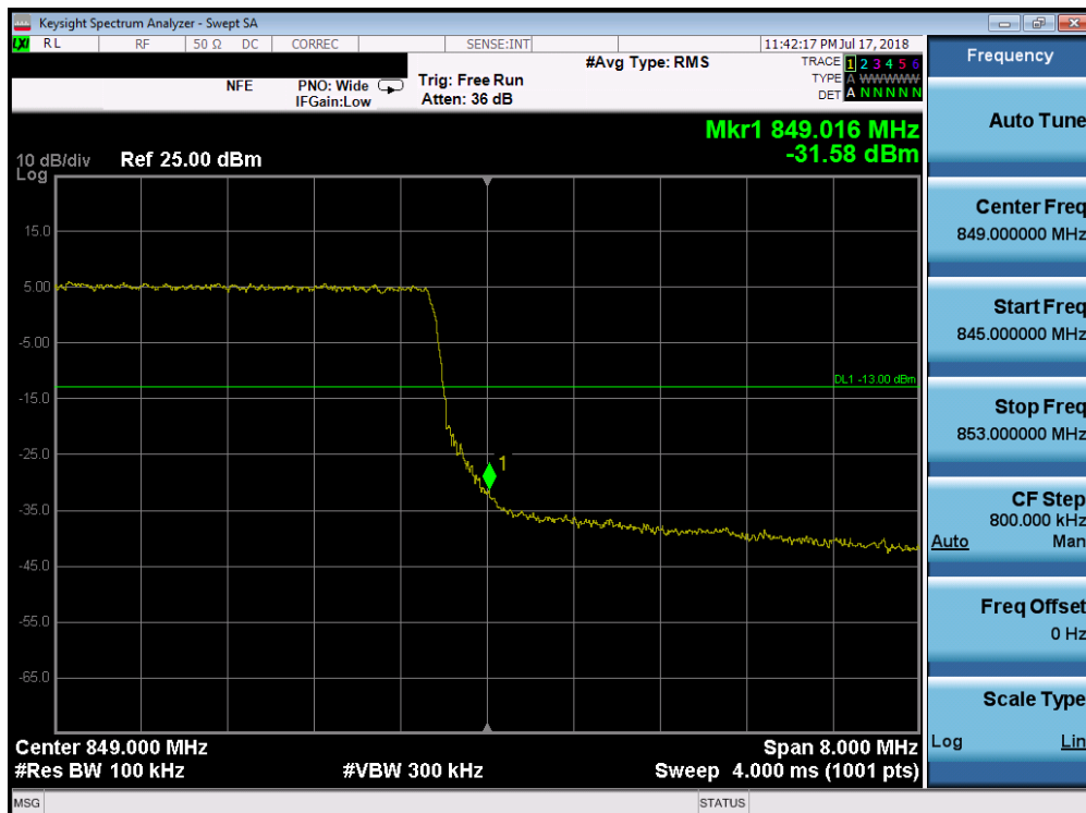
Plot 7-188. Upper Band Edge Plot (Band 26/5 - 10.0MHz QPSK - Full RB Configuration)
