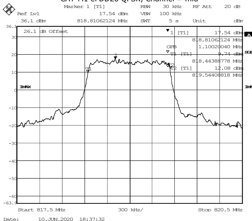
CAT-M1 eFDD26 QPSK, Channel = mid
