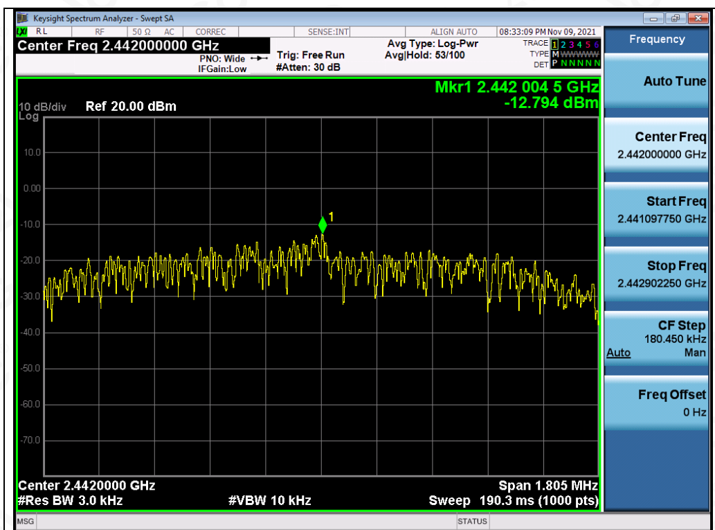
Test_Graph_LE2M_ANT1_2442_2Mbps_PSD
