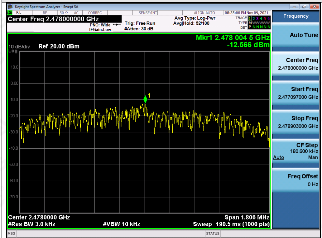
Test_Graph_LE2M_ANT1_2478_2Mbps_PSD
