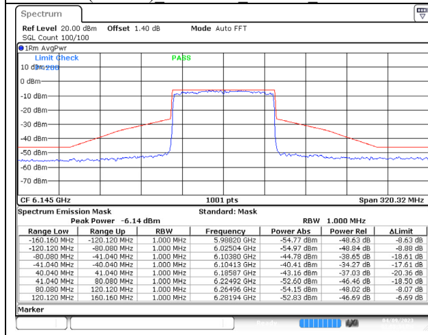
802.11ax (80MHz) 6145MHz Chain C NSS-4
