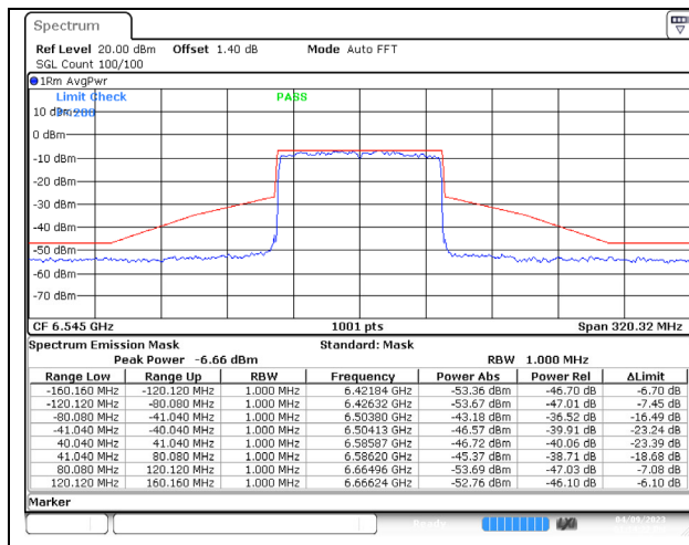
802.11ax (80MHz) 6545MHz Chain A NSS-4
