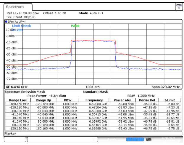
802.11ax (80MHz) 6545MHz Chain B NSS-4
