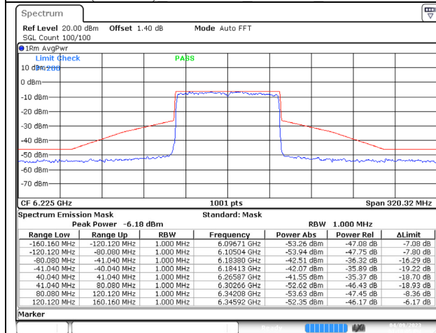
802.11ax (80MHz) 6225MHz Chain C NSS-4
