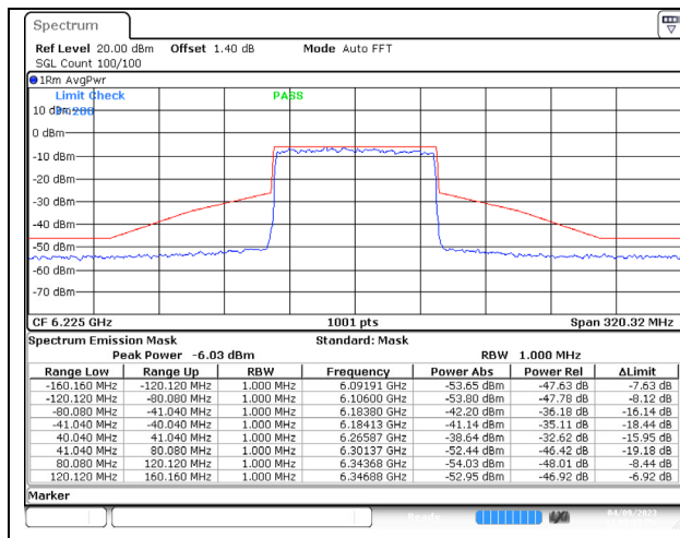
802.11ax (80MHz) 6225MHz Chain A NSS-4
