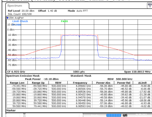
802.11ax (40MHz) 6925MHz Chain A NSS-4
