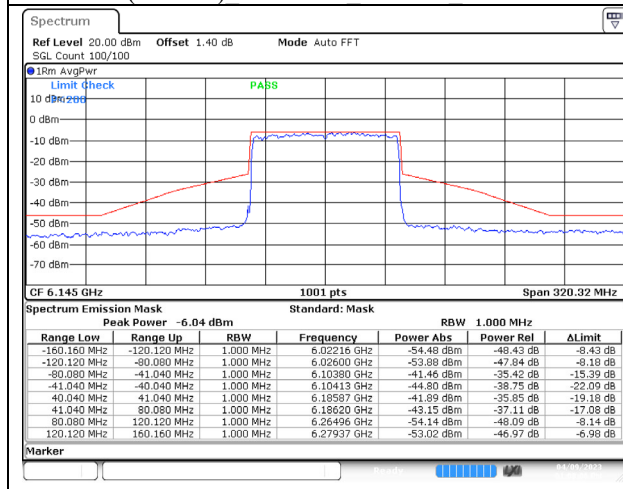
802.11ax (80MHz) 6145MHz Chain A NSS-4
