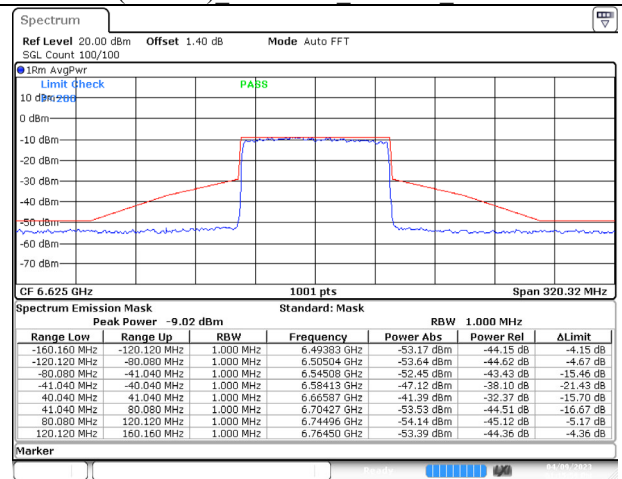
802.11ax (80MHz) 6625MHz Chain B NSS-4
