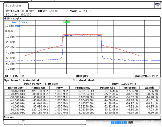
802.11ax (80MHz) 6145MHz Chain B NSS-4
