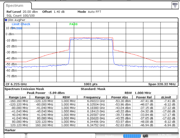
802.11ax (80MHz) 6225MHz Chain D NSS-4
