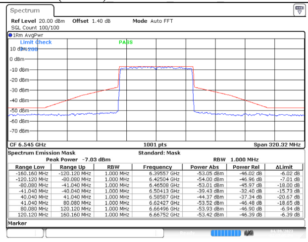
802.11ax (80MHz) 6545MHz Chain D NSS-4
