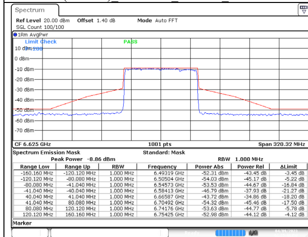
802.11ax (80MHz) 6625MHz Chain A NSS-4
