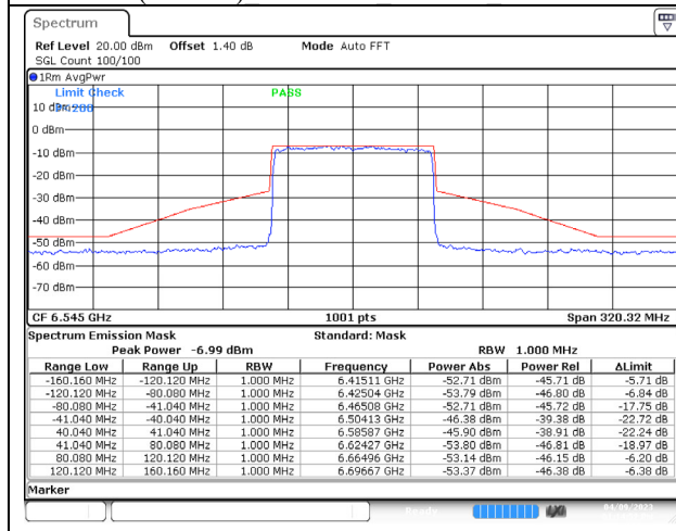
802.11ax (80MHz) 6545MHz Chain C NSS-4
