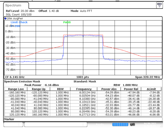
802.11ax (80MHz) 6145MHz Chain D NSS-4
