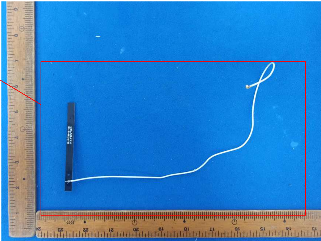
Ant B (For 5G)
