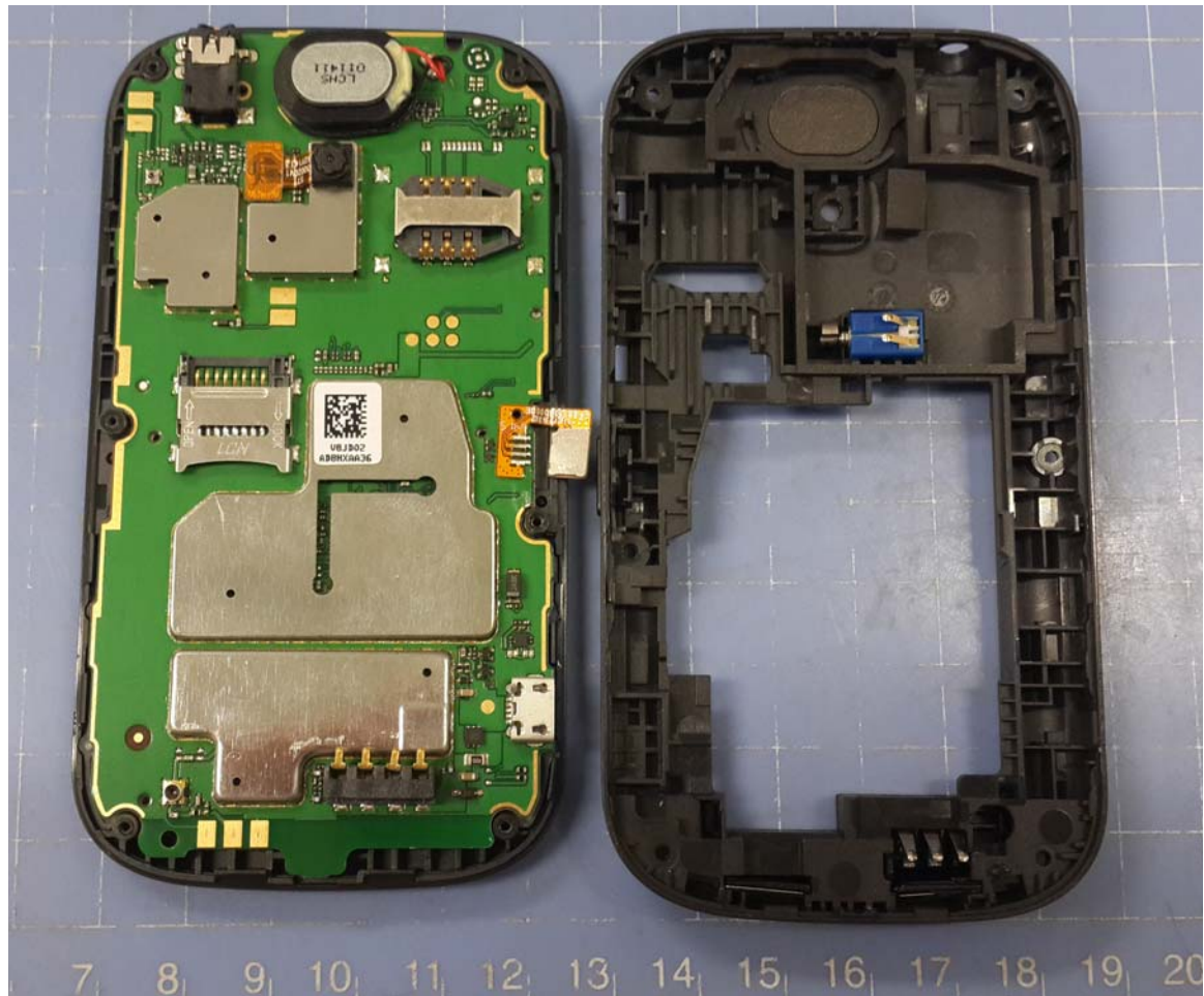
Mobile Phone
