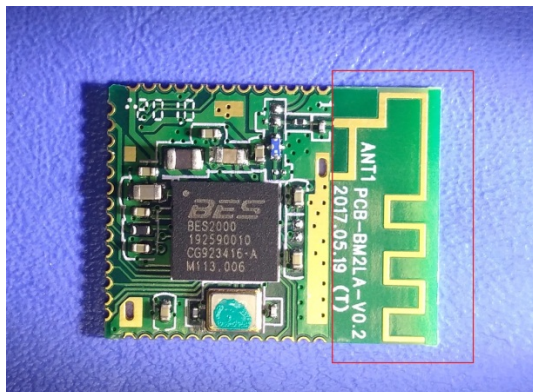
Module/antenna photo
