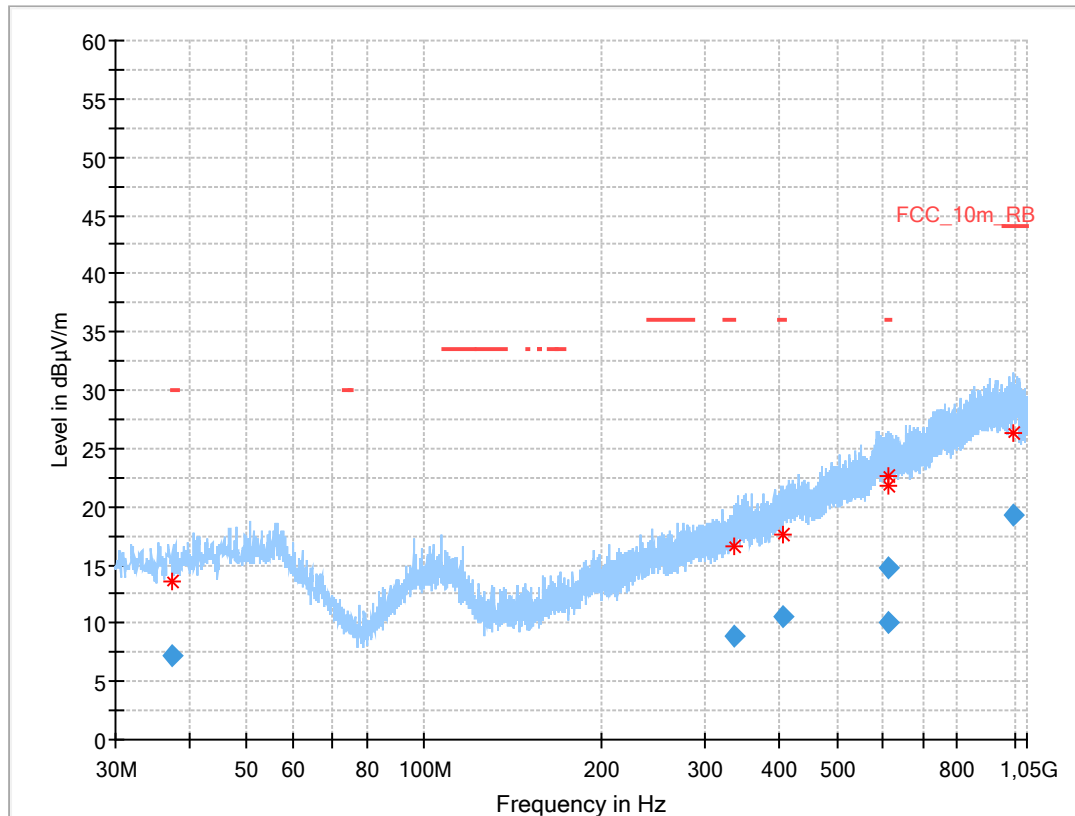
Plot 2: 30 MHz to 1 GHz, TX mode, vertical & horizontal polarization, 2 Msps, valid for all channels
