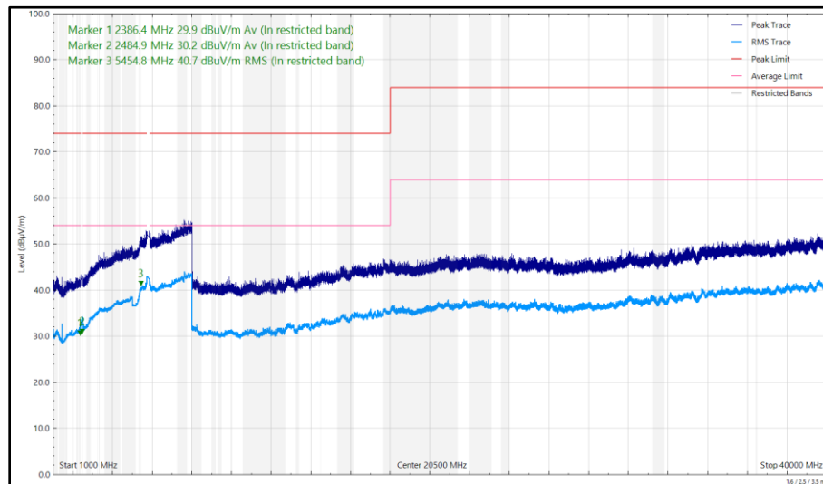
Figure 23 - 5785 MHz (CH157), HT20, CDD, Core 0 + Core 1 and 2441 MHz (CH39), 2DH5, ePA, Core 0 + Core 1, 1 GHz to 40 GHz, Horizontal
