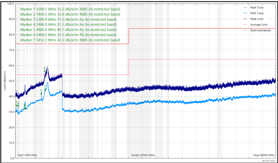
Figure 25 - 5785 MHz (CH157), HT20, CDD, Core 0 + Core 1 and 2441 MHz (CH39), 2DH5, ePA, Core 0 + Core 1, 1 GHz to 40 GHz, Vertical
