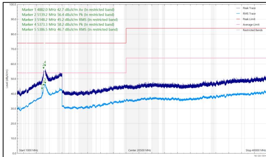
Figure 5 - 5240 MHz (CH48), HT20, CDD, Core 0 + Core 1 and 2441 MHz (CH39), DH5, iPA, Core 2, 1 GHz to 40 GHz, Vertical
