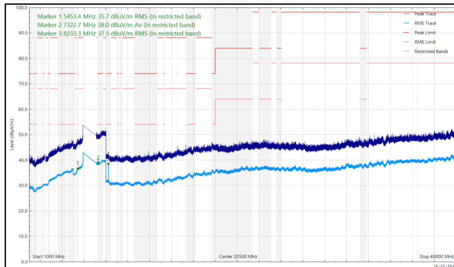
Figure 27 - 6175 MHz (CH45), HE20, SU, CDD, Core 0 + Core 1 and 2441 MHz (CH39), DH5, iPA, Core 2, 1 GHz to 40 GHz, Horizontal
