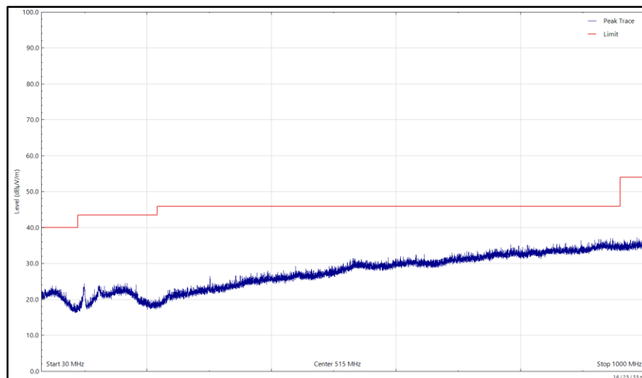
Figure 34 - 6175 MHz (CH45), HE20, SU, CDD, Core 0 + Core 1 and 2441 MHz (CH39), 2DH5, ePA, Core 0 + Core 1, 30 MHz to 1 GHz, Horizontal (Peak)
