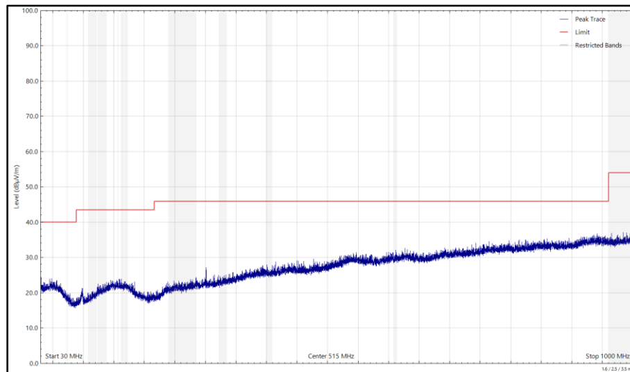
Figure 12 - 5785 MHz (CH157), HT20, CDD, Core 0 + Core 1 and 2441 MHz (CH39), DH5, iPA, Core 2, 30 MHz to 1 GHz, Vertical (Peak)
