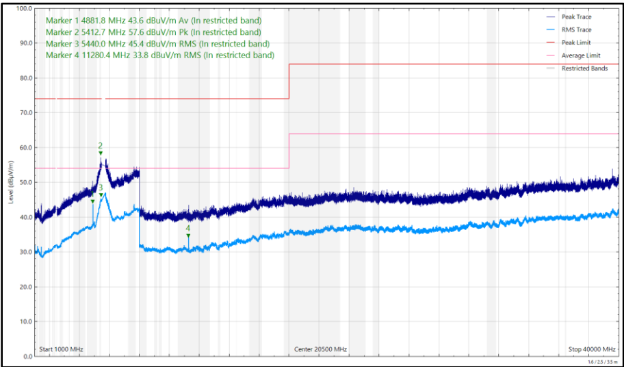
Figure 9 - 5640 MHz (CH128), HT20, CDD, Core 0 + Core 1 and 2441 MHz (CH39), DH5, iPA, Core 2, 1 GHz to 40 GHz, Vertical
