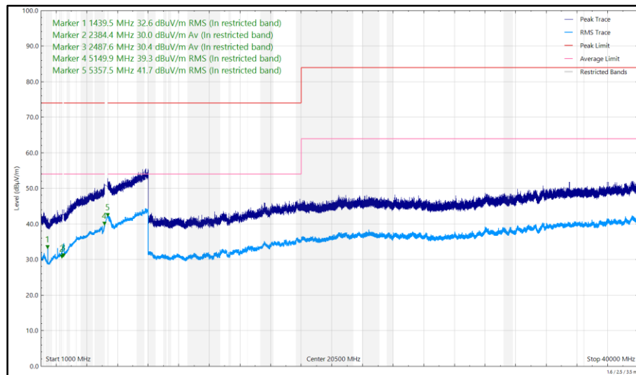
Figure 15 - 5240 MHz (CH48), HT20, CDD, Core 0 + Core 1 and 2441 MHz (CH39), 2DH5, ePA, Core 0 + Core 1, 1 GHz to 40 GHz, Horizontal
