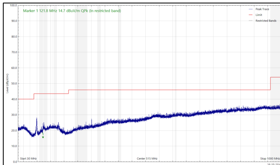
Figure 2 - 5240 MHz (CH48), HT20, CDD, Core 0 + Core 1 and 2441 MHz (CH39), DH5, iPA, Core 2, 30 MHz to 1 GHz, Horizontal (Peak)
