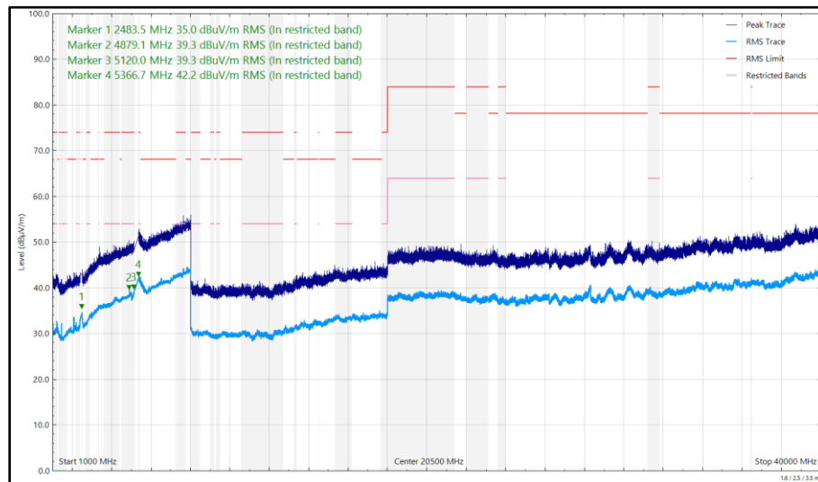
Figure 59 - 5240 MHz (CH48), HT20, CDD, Core 0 + Core 1 and 2440 MHz (CH18), Core 0, ePA, 1 GHz to 40 GHz, Horizontal
