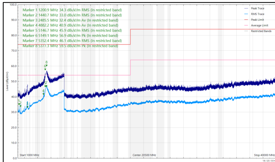
Figure 17 - 5240 MHz (CH48), HT20, CDD, Core 0 + Core 1 and 2441 MHz (CH39), 2DH5, ePA, Core 0 + Core 1, 1 GHz to 40 GHz, Vertical
