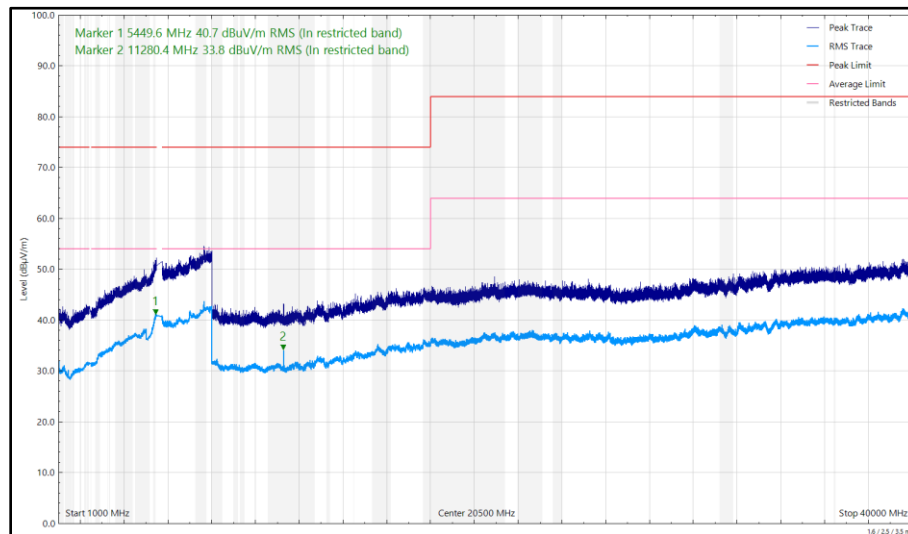
Figure 7 - 5640 MHz (CH128), HT20, CDD, Core 0 + Core 1 and 2441 MHz (CH39), DH5, iPA, Core 2, 1 GHz to 40 GHz, Horizontal
