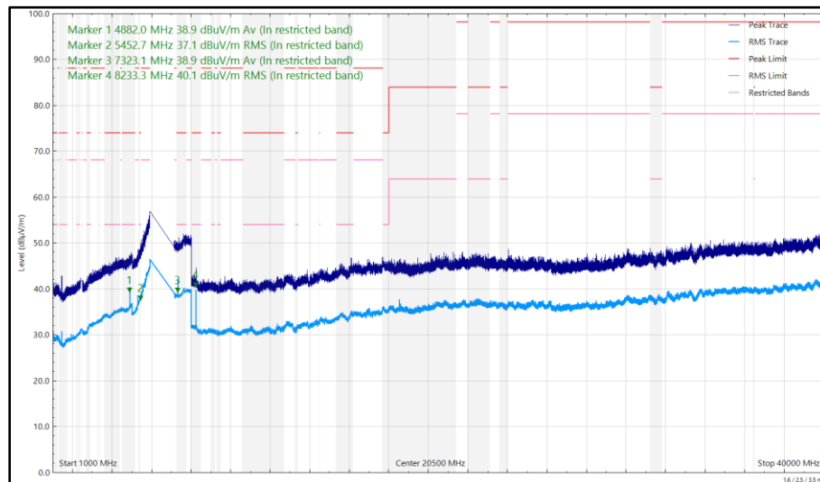
Figure 29 - 6175 MHz (CH45), HE20, SU, CDD, Core 0 + Core 1 and 2441 MHz (CH39), DH5, iPA, Core 2, 1 GHz to 40 GHz, Vertical
