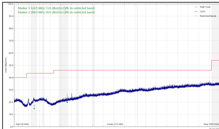
Figure 14 - 5240 MHz (CH48), HT20, CDD, Core 0 + Core 1 and 2441 MHz (CH39), 2DH5, ePA, Core 0 + Core 1, 30 MHz to 1 GHz, Horizontal (Peak)
