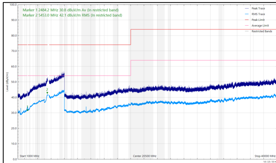
Figure 19 - 5640 MHz (CH128), HT20, CDD, Core 0 + Core 1 and 2441 MHz (CH39), 2DH5, ePA, Core 0 + Core 1, 1 GHz to 40 GHz, Horizontal
