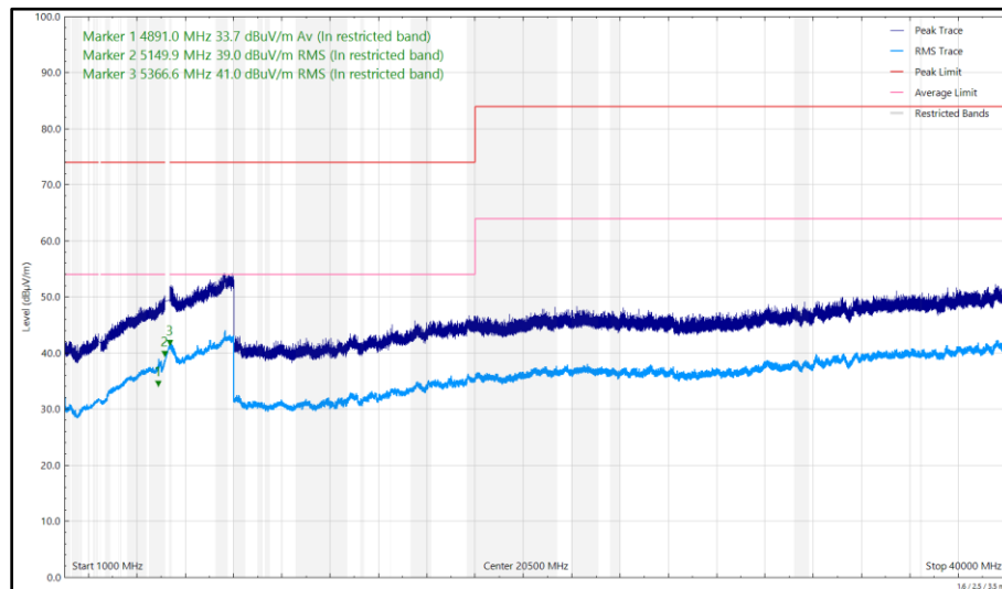
Figure 3 - 5240 MHz (CH48), HT20, CDD, Core 0 + Core 1 and 2441 MHz (CH39), DH5, iPA, Core 2, 1 GHz to 40 GHz, Horizontal
