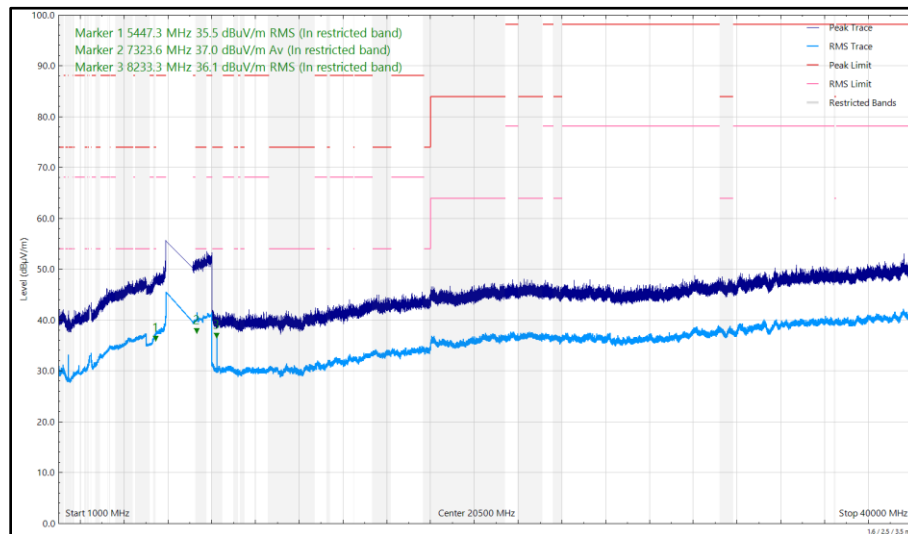
Figure 35 - 6175 MHz (CH45), HE20, SU, CDD, Core 0 + Core 1 and 2441 MHz (CH39), 2DH5, ePA, Core 0 + Core 1, 1 GHz to 40 GHz, Horizontal
