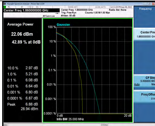
Band25-20MHz-16QAM-26140-27RB#0
