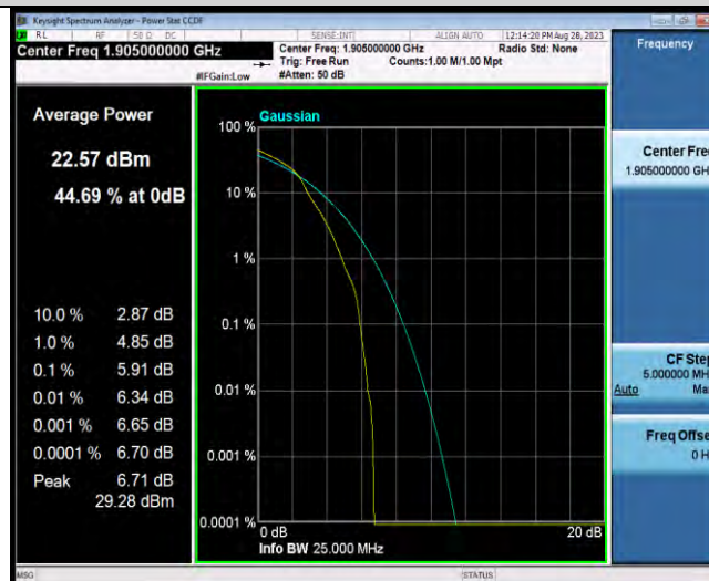
Band25-20MHz-16QAM-26590-27RB#0
