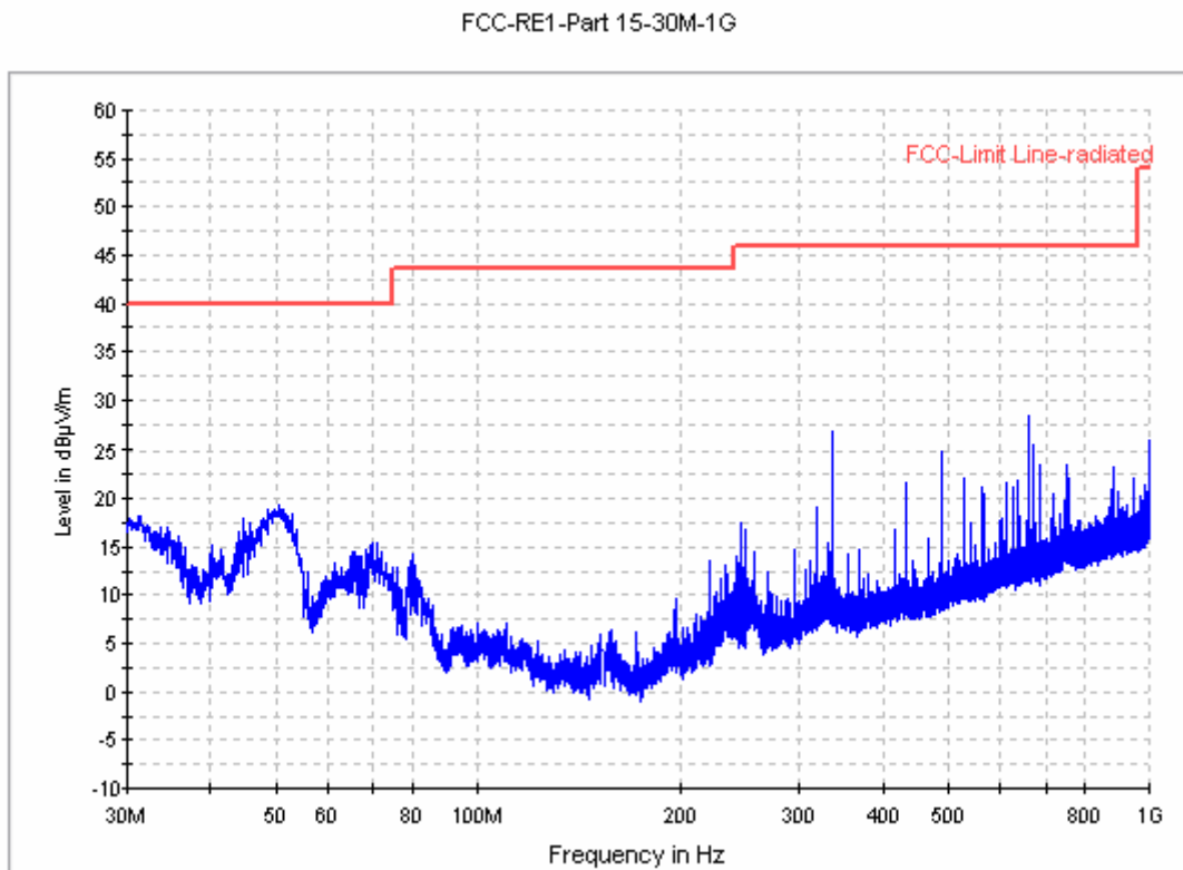
Figure A.3 Radiated Emission from 30MHz to 1GHz (Set.2, Charging mode)
