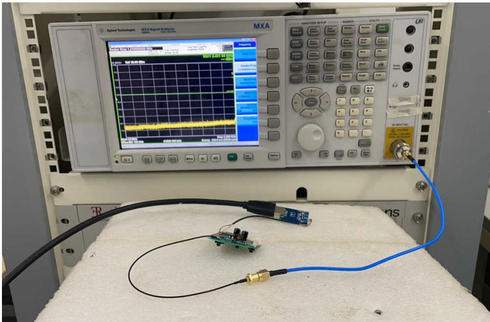
CONDUCTED TEST SETUP
