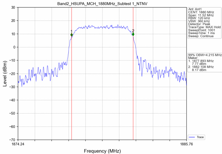
Band II_HSUPA_MCH_1880MHz_Subtest 1_NTNV
