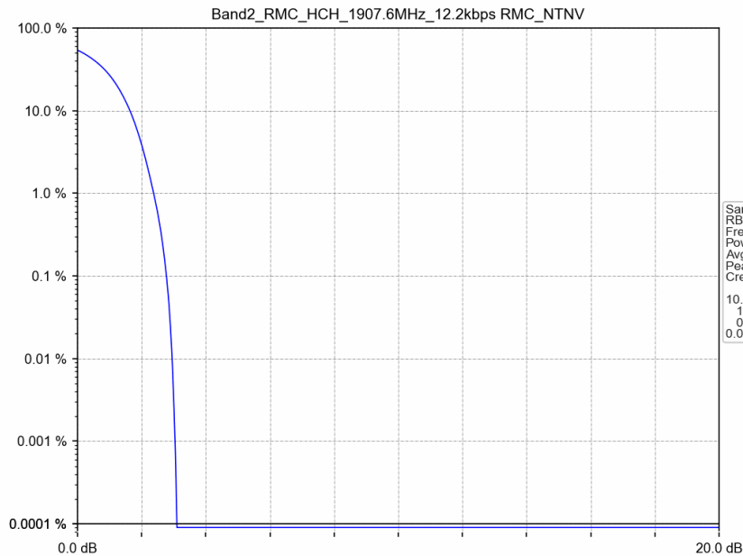
Band II_RMC_HCH_1907.6MHz_12.2kbps RMC_NTNV
