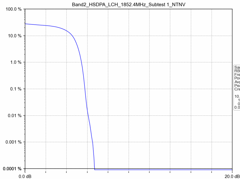
Band II_HSDPA_LCH_1852.4MHz_Subtest 1_NTNV
