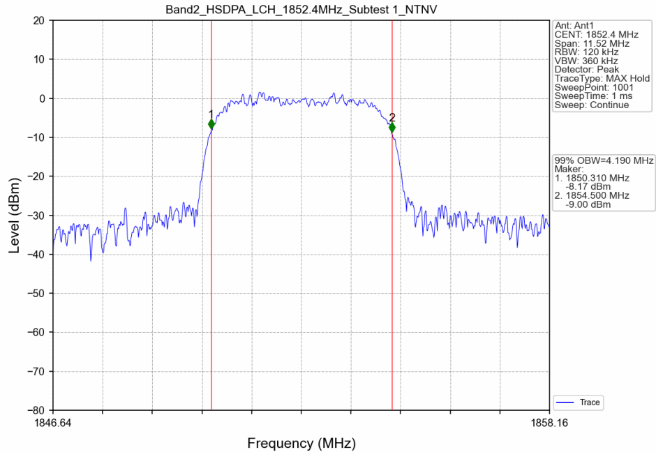
Band II_HSDPA_LCH_1852.4MHz_Subtest 1_NTNV
