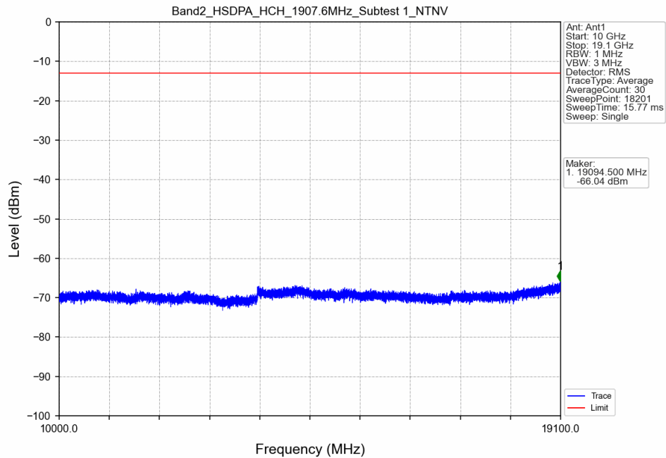
Band II_HSDPA_HCH_1907.6MHz_Subtest 1_NTNV
