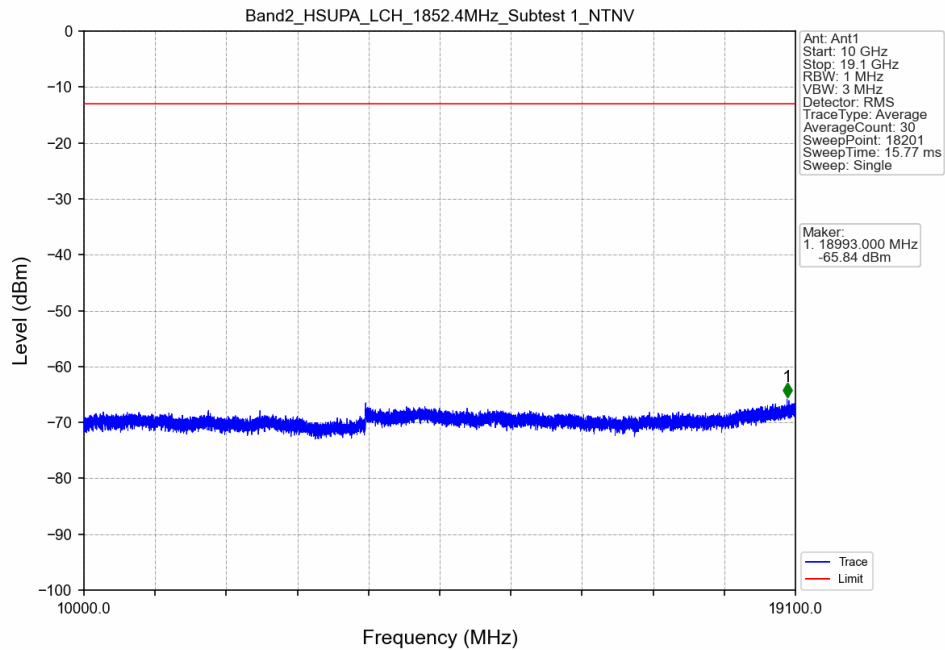
Band II_HSUPA_LCH_1852.4MHz_Subtest 1_NTNV
