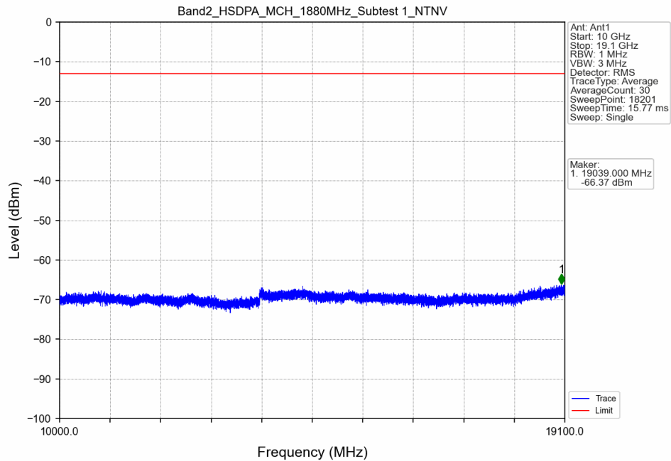
Band II_HSDPA_MCH_1880MHz_Subtest 1_NTNV
