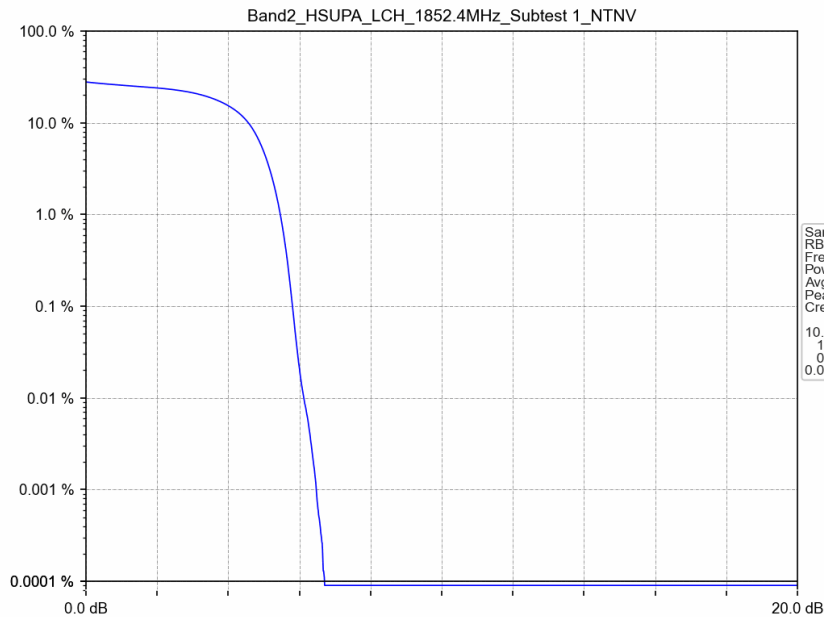
Band II_HSUPA_LCH_1852.4MHz_Subtest 1_NTNV
