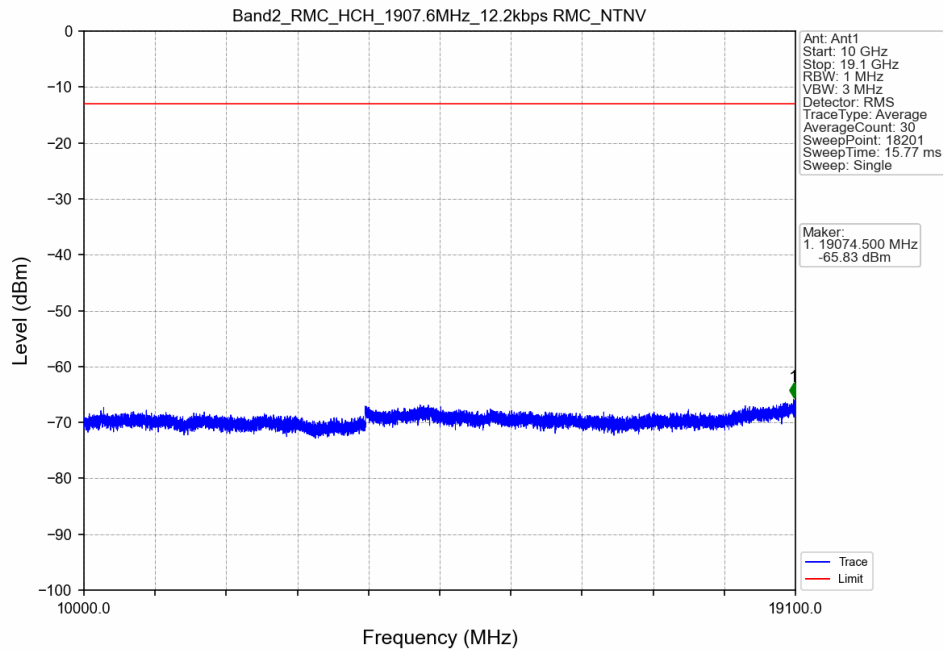
Band II_RMC_HCH_1907.6MHz_12.2kbps RMC_NTNV
