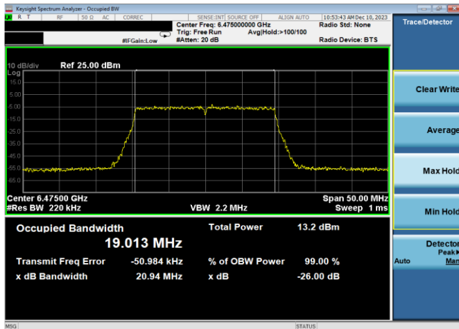
Plot 7-27. 26dB & 99% Bandwidth Plot Antenna WF7a (20MHz 802.11ax (UNII Band 6) – Ch. 105, MCS4)
