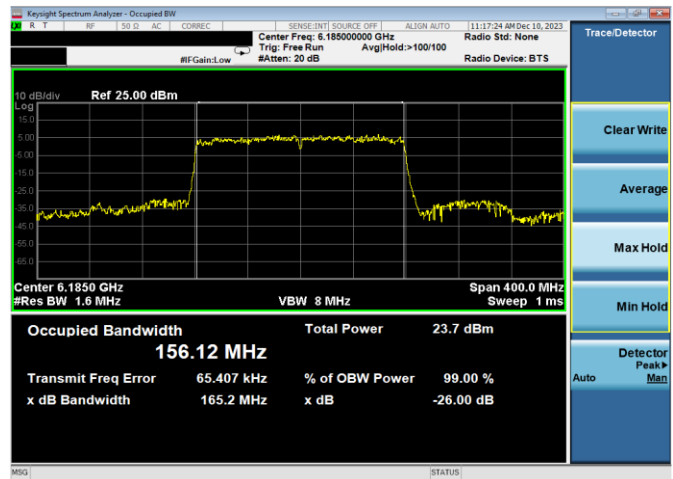
Plot 7-45. 26dB & 99% Bandwidth Plot Antenna WF7a (160MHz 802.11ax (UNII Band 5) – Ch. 47, MCS11)
