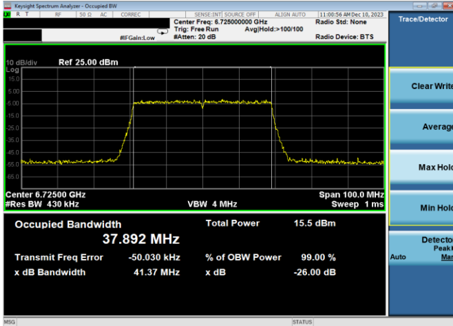
Plot 7-33. 26dB & 99% Bandwidth Plot Antenna WF7a (40MHz 802.11ax (UNII Band 7) – Ch. 155, MCS4)
