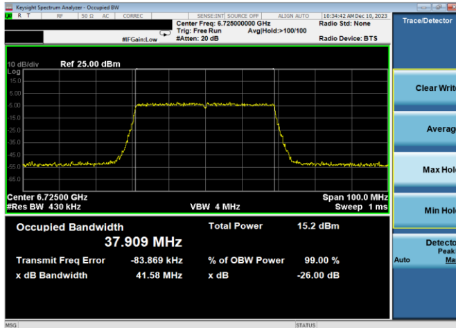
Plot 7-13. 26dB & 99% Bandwidth Plot Antenna WF7a (40MHz 802.11ax (UNII Band 7) – Ch. 155, MCS2)
