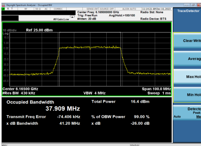
Plot 7-43. 26dB & 99% Bandwidth Plot Antenna WF7a (40MHz 802.11ax (UNII Band 5) – Ch. 43, MCS11)
