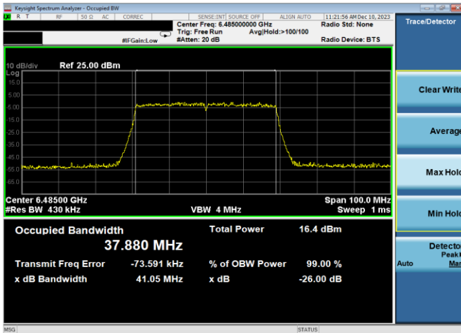
Plot 7-48. 26dB & 99% Bandwidth Plot Antenna WF7a (40MHz 802.11ax (UNII Band 6) – Ch. 107, MCS11)
