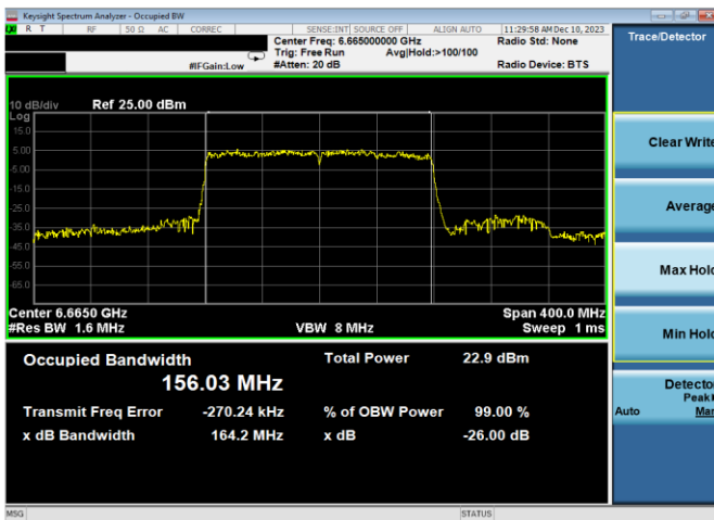
Plot 7-55. 26dB & 99% Bandwidth Plot Antenna WF7a (160MHz 802.11ax (UNII Band 7) – Ch. 143, MCS11)
