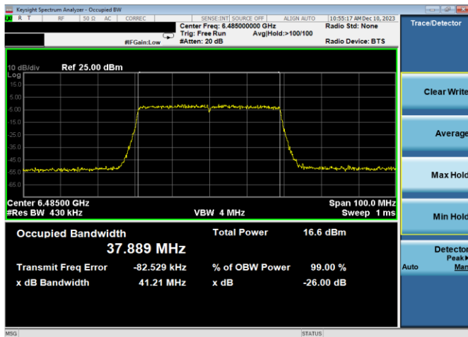
Plot 7-28. 26dB & 99% Bandwidth Plot Antenna WF7a (40MHz 802.11ax (UNII Band 6) – Ch. 107, MCS4)
