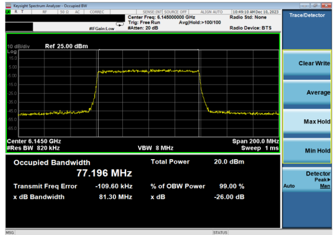
Plot 7-24. 26dB & 99% Bandwidth Plot Antenna WF7a (80MHz 802.11ax (UNII Band 5) – Ch. 39, MCS4)
