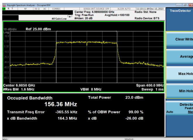
Plot 7-40. 26dB & 99% Bandwidth Plot Antenna WF7a (160MHz 802.11ax (UNII Band 8) – Ch. 207, MCS4)
