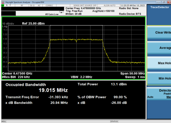
Plot 7-47. 26dB & 99% Bandwidth Plot Antenna WF7a (20MHz 802.11ax (UNII Band 6) – Ch. 105, MCS11)
