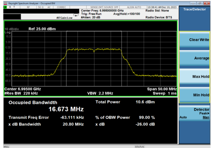
Plot 7-16. 26dB & 99% Bandwidth Plot Antenna WF7a (20MHz 802.11a (UNII Band 8) – Ch. 209, 12Mbps)
