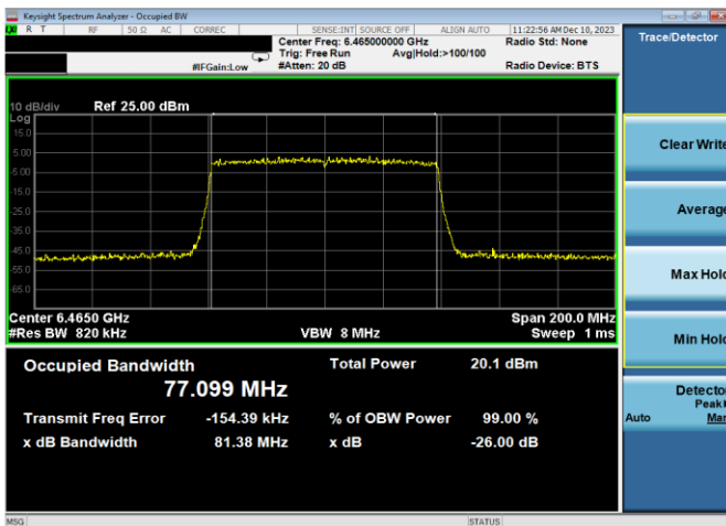
Plot 7-49. 26dB & 99% Bandwidth Plot Antenna WF7a (80MHz 802.11ax (UNII Band 6) – Ch. 103, MCS11)
