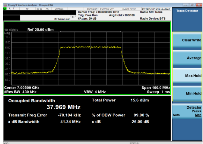
Plot 7-18. 26dB & 99% Bandwidth Plot Antenna WF7a (40MHz 802.11ax (UNII Band 8) – Ch. 211, MCS2)
