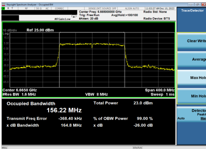
Plot 7-35. 26dB & 99% Bandwidth Plot Antenna WF7a (160MHz 802.11ax (UNII Band 7) – Ch. 143, MCS4)
