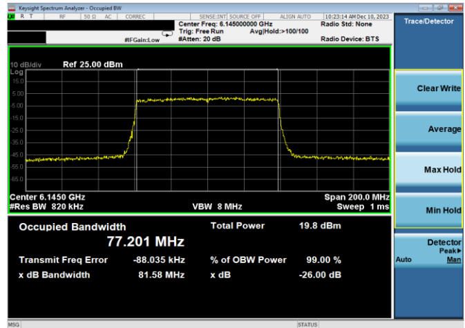
Plot 7-4. 26dB & 99% Bandwidth Plot Antenna WF7a (80MHz 802.11ax (UNII Band 5) – Ch. 39, MCS2)
