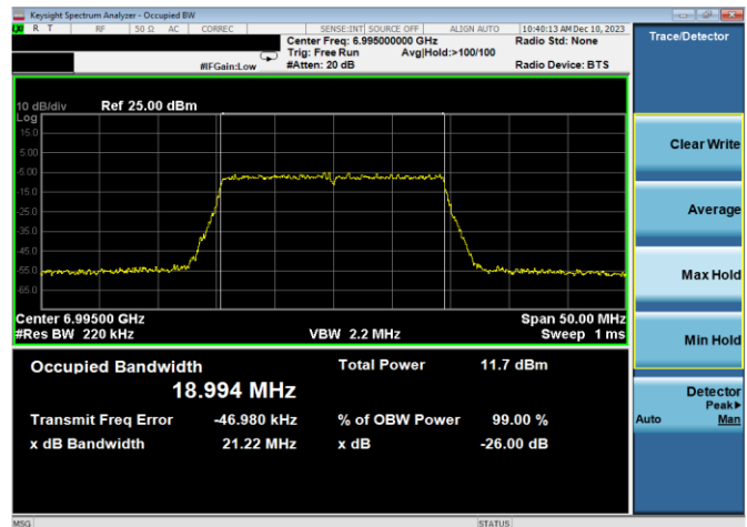
Plot 7-17. 26dB & 99% Bandwidth Plot Antenna WF7a (20MHz 802.11ax (UNII Band 8) – Ch. 209, MCS2)
