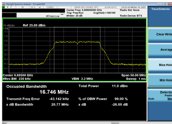
Plot 7-11. 26dB & 99% Bandwidth Plot Antenna WF7a (20MHz 802.11a (UNII Band 7) – Ch. 149, 12Mbps)
