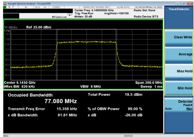
Plot 7-64. 26dB & 99% Bandwidth Plot Antenna WF2a (80MHz 802.11ax (UNII Band 5) – Ch. 39, MCS2)
