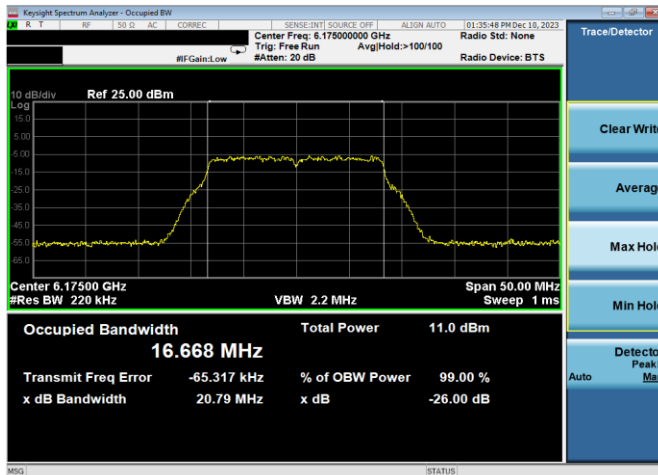
Plot 7-61. 26dB & 99% Bandwidth Plot Antenna WF2a (20MHz 802.11a (UNII Band 5) – Ch. 45, 12Mbps)
