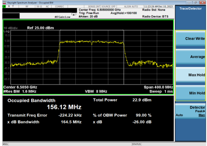
Plot 7-50. 26dB & 99% Bandwidth Plot Antenna WF7a (160MHz 802.11ax (UNII Band 6) – Ch. 111, MCS11)
