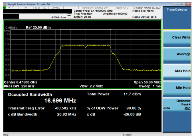
Plot 7-6. 26dB & 99% Bandwidth Plot Antenna WF7a (20MHz 802.11a (UNII Band 6) – Ch. 105, 12Mbps)
