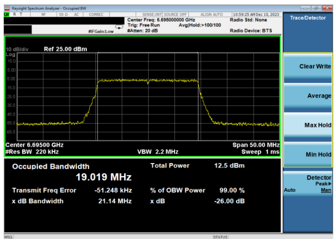
Plot 7-32. 26dB & 99% Bandwidth Plot Antenna WF7a (20MHz 802.11ax (UNII Band 7) – Ch. 149, MCS4)
