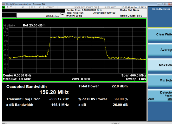
Plot 7-10. 26dB & 99% Bandwidth Plot Antenna WF7a (160MHz 802.11ax (UNII Band 6) – Ch. 111, MCS2)
