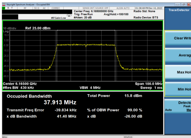
Plot 7-63. 26dB & 99% Bandwidth Plot Antenna WF2a (40MHz 802.11ax (UNII Band 5) – Ch. 43, MCS2)
