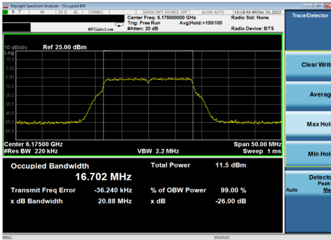
Plot 7-1. 26dB & 99% Bandwidth Plot Antenna WF7a (20MHz 802.11a (UNII Band 5) – Ch. 45, 12Mbps)
