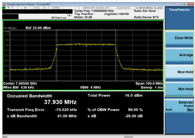
Plot 7-38. 26dB & 99% Bandwidth Plot Antenna WF7a (40MHz 802.11ax (UNII Band 8) – Ch. 211, MCS4)
