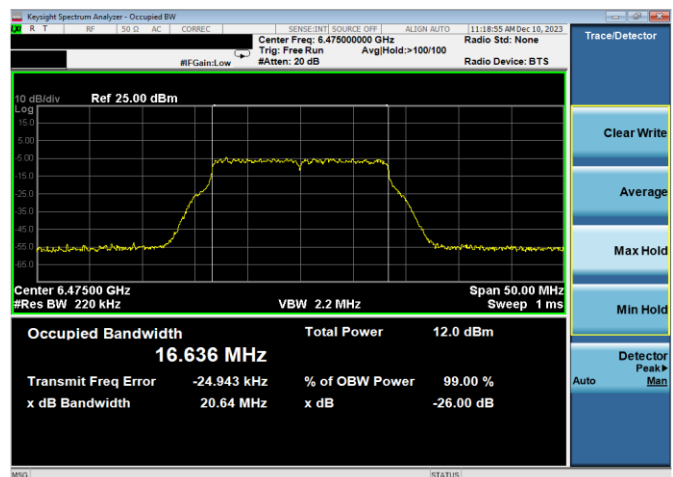
Plot 7-46. 26dB & 99% Bandwidth Plot Antenna WF7a (20MHz 802.11a (UNII Band 6) – Ch. 105, 54Mbps)
