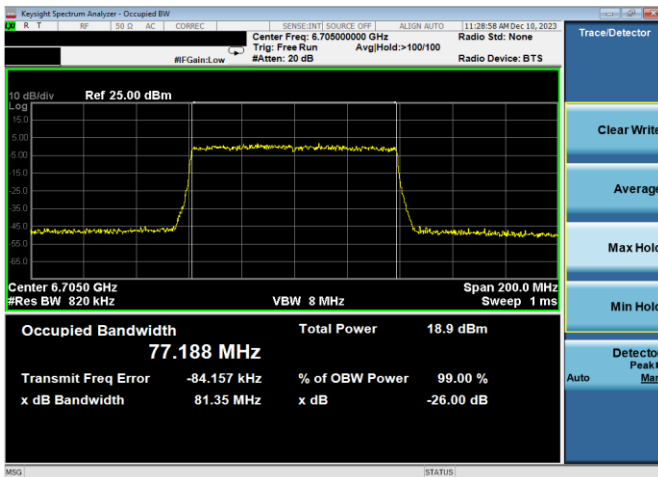
Plot 7-54. 26dB & 99% Bandwidth Plot Antenna WF7a (80MHz 802.11ax (UNII Band 7) – Ch. 151, MCS11)
