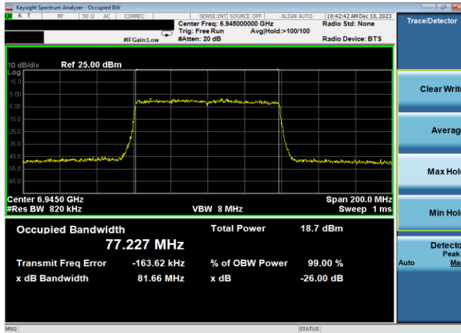
Plot 7-19. 26dB & 99% Bandwidth Plot Antenna WF7a (80MHz 802.11ax (UNII Band 8) – Ch. 199, MCS2)
