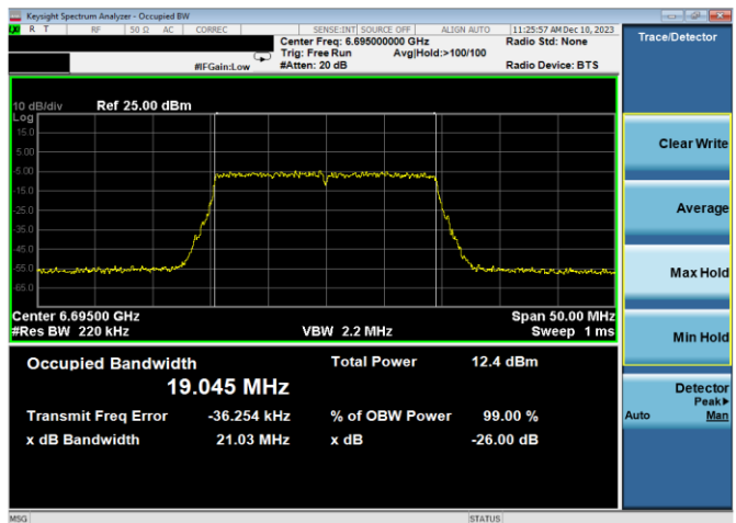
Plot 7-52. 26dB & 99% Bandwidth Plot Antenna WF7a (20MHz 802.11ax (UNII Band 7) – Ch. 149, MCS11)
