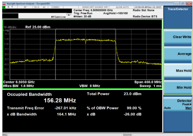
Plot 7-30. 26dB & 99% Bandwidth Plot Antenna WF7a (160MHz 802.11ax (UNII Band 6) – Ch. 111, MCS4)
