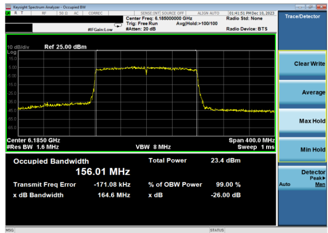
Plot 7-65. 26dB & 99% Bandwidth Plot Antenna WF2a (160MHz 802.11ax (UNII Band 5) – Ch. 47, MCS2)
