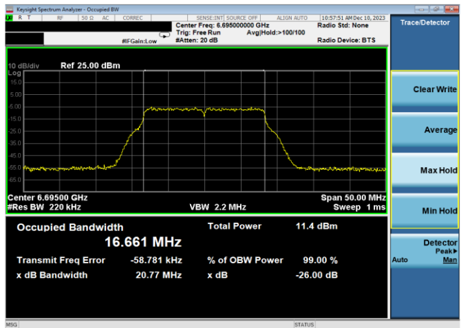
Plot 7-31. 26dB & 99% Bandwidth Plot Antenna WF7a (20MHz 802.11a (UNII Band 7) – Ch. 149, 24Mbps)
