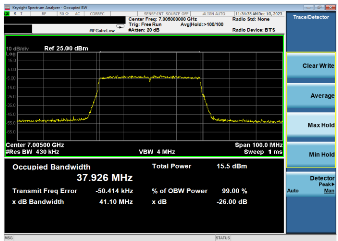
Plot 7-58. 26dB & 99% Bandwidth Plot Antenna WF7a (40MHz 802.11ax (UNII Band 8) – Ch. 211, MCS11)
