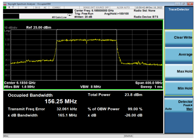
Plot 7-25. 26dB & 99% Bandwidth Plot Antenna WF7a (160MHz 802.11ax (UNII Band 5) – Ch. 47, MCS4)
