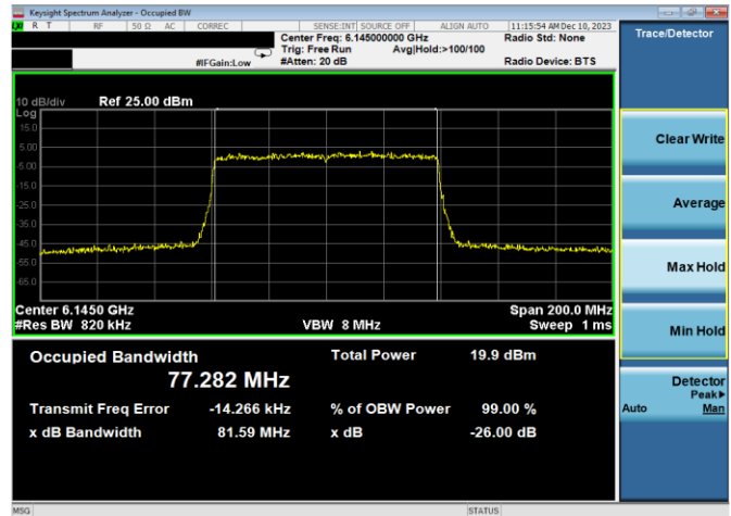
Plot 7-44. 26dB & 99% Bandwidth Plot Antenna WF7a (80MHz 802.11ax (UNII Band 5) – Ch. 39, MCS11)
