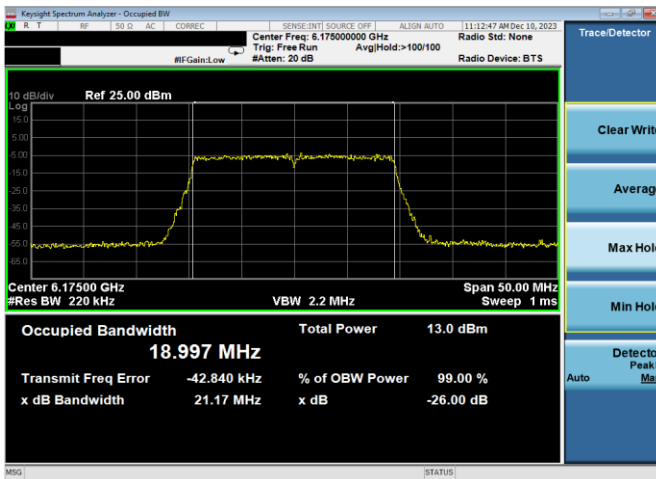
Plot 7-42. 26dB & 99% Bandwidth Plot Antenna WF7a (20MHz 802.11ax (UNII Band 5) – Ch. 45, MCS11)
