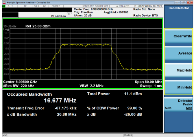
Plot 7-36. 26dB & 99% Bandwidth Plot Antenna WF7a (20MHz 802.11a (UNII Band 8) – Ch. 209, 24Mbps)
