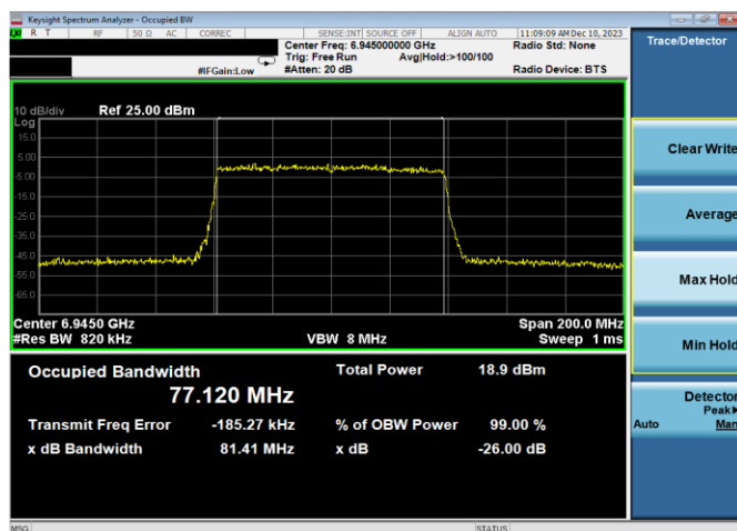
Plot 7-39. 26dB & 99% Bandwidth Plot Antenna WF7a (80MHz 802.11ax (UNII Band 8) – Ch. 199, MCS4)
