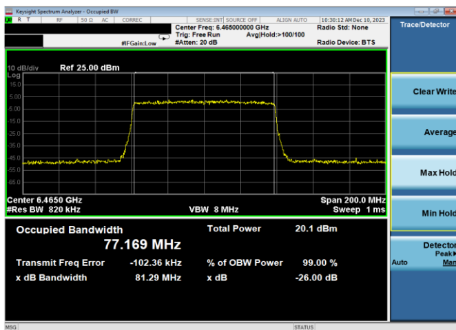
Plot 7-9. 26dB & 99% Bandwidth Plot Antenna WF7a (80MHz 802.11ax (UNII Band 6) – Ch. 103, MCS2)
