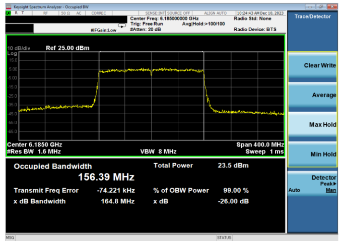
Plot 7-5. 26dB & 99% Bandwidth Plot Antenna WF7a (160MHz 802.11ax (UNII Band 5) – Ch. 47, MCS2)
