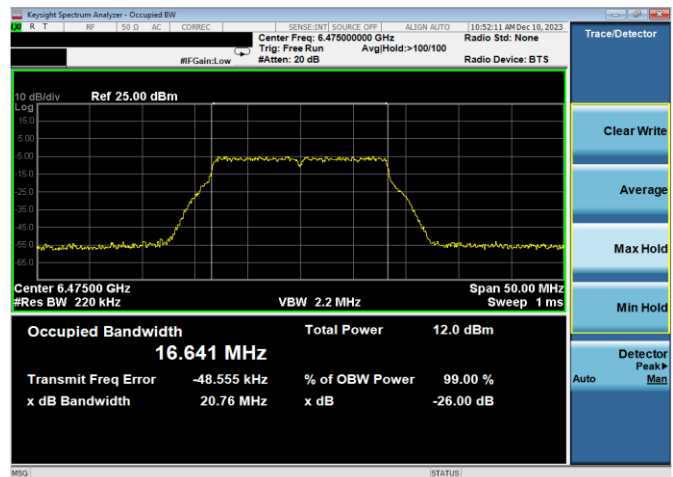
Plot 7-26. 26dB & 99% Bandwidth Plot Antenna WF7a (20MHz 802.11a (UNII Band 6) – Ch. 105, 24Mbps)
