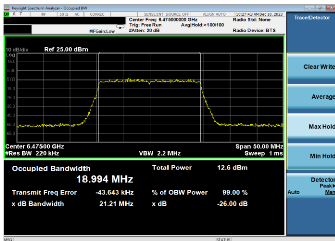
Plot 7-7. 26dB & 99% Bandwidth Plot Antenna WF7a (20MHz 802.11ax (UNII Band 6) – Ch. 105, MCS2)
