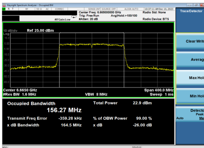
Plot 7-15. 26dB & 99% Bandwidth Plot Antenna WF7a (160MHz 802.11ax (UNII Band 7) – Ch. 143, MCS2)
