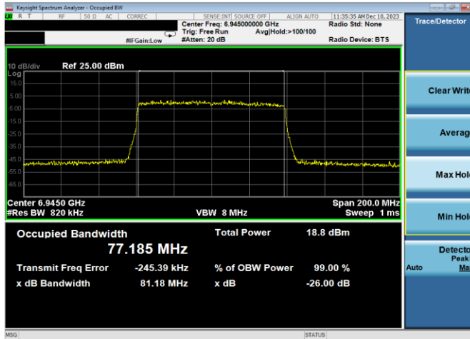
Plot 7-59. 26dB & 99% Bandwidth Plot Antenna WF7a (80MHz 802.11ax (UNII Band 8) – Ch. 199, MCS11)
