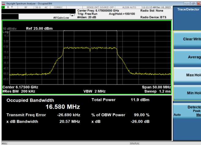
Plot 7-41. 26dB & 99% Bandwidth Plot Antenna WF7a (20MHz 802.11a (UNII Band 5) – Ch. 45, 54Mbps)
