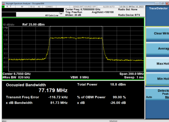
Plot 7-14. 26dB & 99% Bandwidth Plot Antenna WF7a (80MHz 802.11ax (UNII Band 7) – Ch. 151, MCS2)
