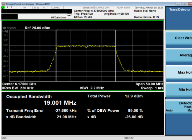
Plot 7-22. 26dB & 99% Bandwidth Plot Antenna WF7a (20MHz 802.11ax (UNII Band 5) – Ch. 45, MCS4)
