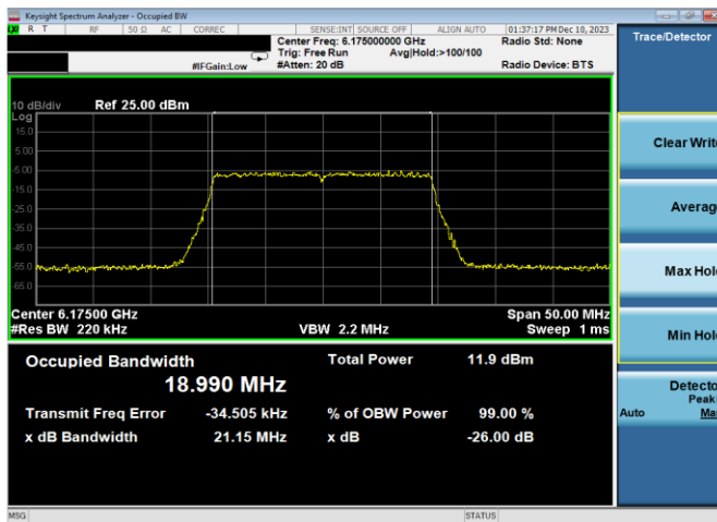
Plot 7-62. 26dB & 99% Bandwidth Plot Antenna WF2a (20MHz 802.11ax (UNII Band 5) – Ch. 45, MCS2)
