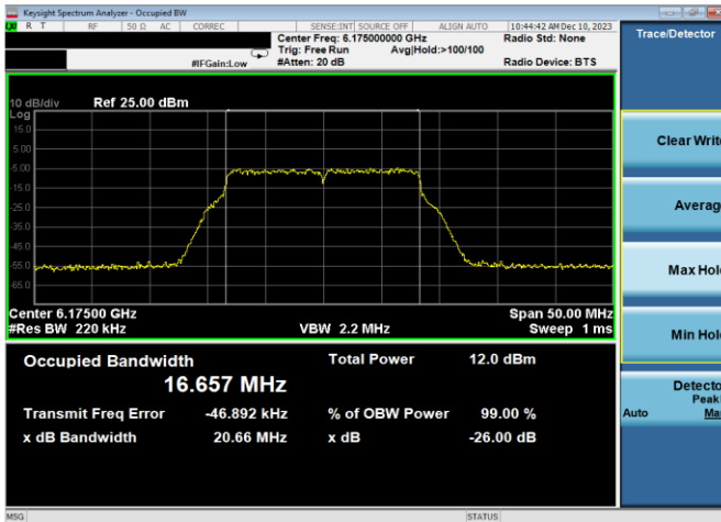
Plot 7-21. 26dB & 99% Bandwidth Plot Antenna WF7a (20MHz 802.11a (UNII Band 5) – Ch. 45, 24Mbps)
