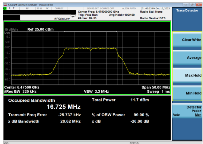
Plot 7-66. 26dB & 99% Bandwidth Plot Antenna WF2a (20MHz 802.11a (UNII Band 6) – Ch. 105, 12Mbps)
