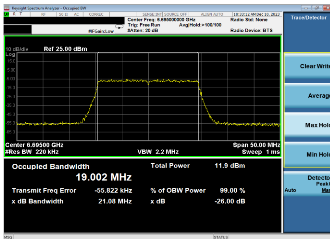
Plot 7-12. 26dB & 99% Bandwidth Plot Antenna WF7a (20MHz 802.11ax (UNII Band 7) – Ch. 149, MCS2)
