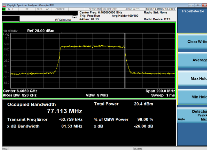
Plot 7-29. 26dB & 99% Bandwidth Plot Antenna WF7a (80MHz 802.11ax (UNII Band 6) – Ch. 103, MCS4)
