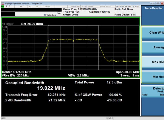
Plot 7-2. 26dB & 99% Bandwidth Plot Antenna WF7a (20MHz 802.11ax (UNII Band 5) – Ch. 45, MCS2)
