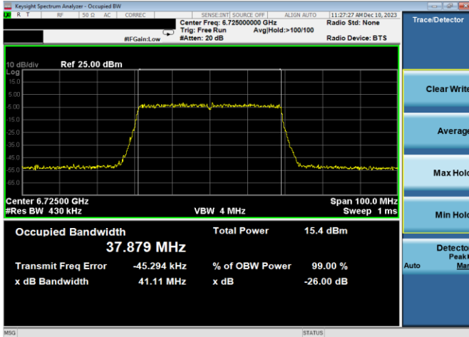
Plot 7-53. 26dB & 99% Bandwidth Plot Antenna WF7a (40MHz 802.11ax (UNII Band 7) – Ch. 155, MCS11)
