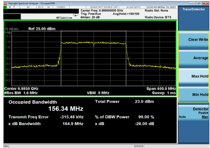
Plot 7-20. 26dB & 99% Bandwidth Plot Antenna WF7a (160MHz 802.11ax (UNII Band 8) – Ch. 207, MCS2)
