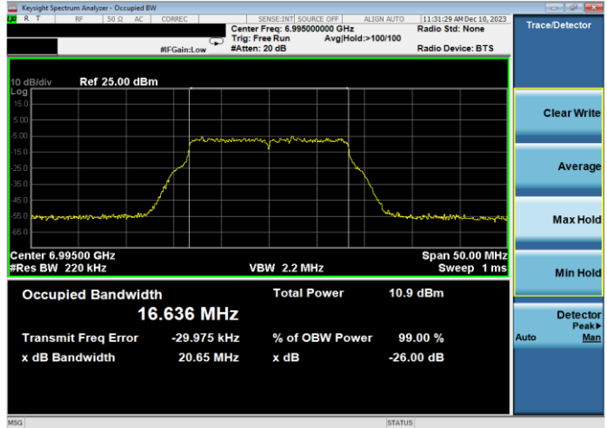
Plot 7-56. 26dB & 99% Bandwidth Plot Antenna WF7a (20MHz 802.11a (UNII Band 8) – Ch. 209, 54Mbps)
