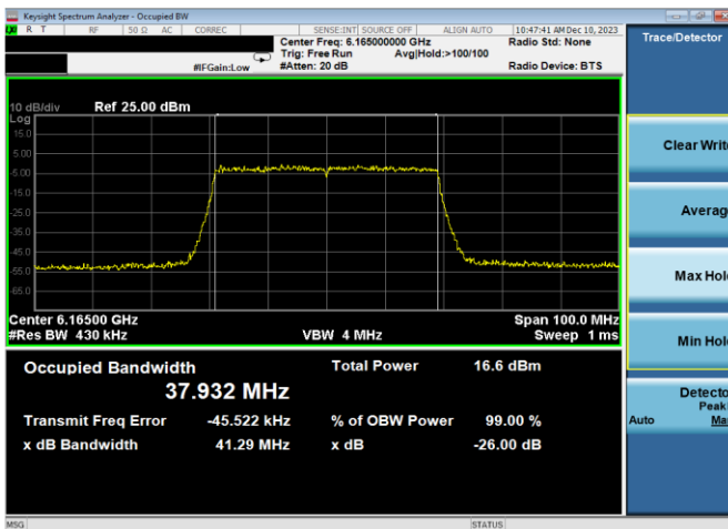
Plot 7-23. 26dB & 99% Bandwidth Plot Antenna WF7a (40MHz 802.11ax (UNII Band 5) – Ch. 43, MCS4)
