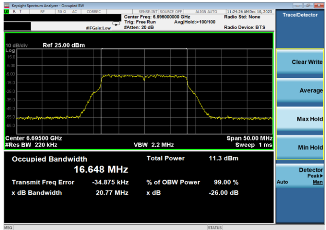
Plot 7-51. 26dB & 99% Bandwidth Plot Antenna WF7a (20MHz 802.11a (UNII Band 7) – Ch. 149, 54Mbps)
