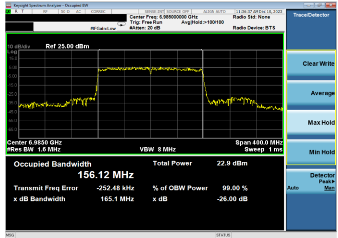
Plot 7-60. 26dB & 99% Bandwidth Plot Antenna WF7a (160MHz 802.11ax (UNII Band 8) – Ch. 207, MCS11)
