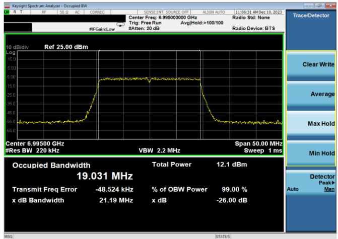
Plot 7-37. 26dB & 99% Bandwidth Plot Antenna WF7a (20MHz 802.11ax (UNII Band 8) – Ch. 209, MCS4)
