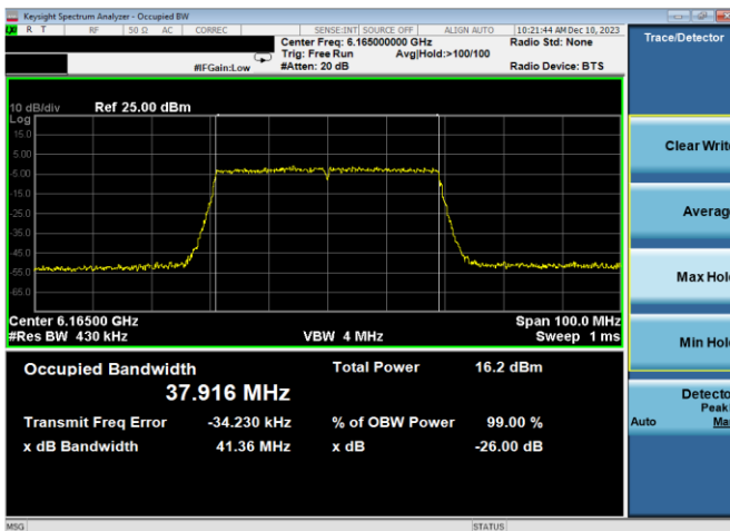
Plot 7-3. 26dB & 99% Bandwidth Plot Antenna WF7a (40MHz 802.11ax (UNII Band 5) – Ch. 43, MCS2)
