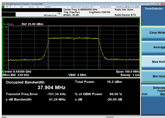
Plot 7-8. 26dB & 99% Bandwidth Plot Antenna WF7a (40MHz 802.11ax (UNII Band 6) – Ch. 107, MCS2)
