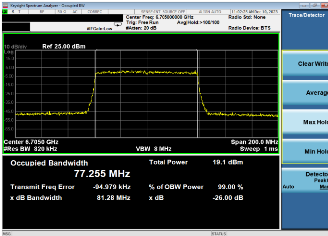
Plot 7-34. 26dB & 99% Bandwidth Plot Antenna WF7a (80MHz 802.11ax (UNII Band 7) – Ch. 151, MCS4)
