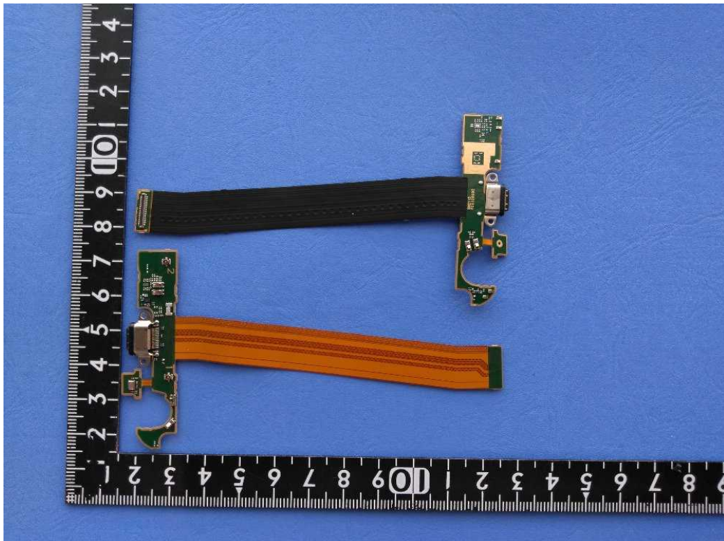
USB PCB
