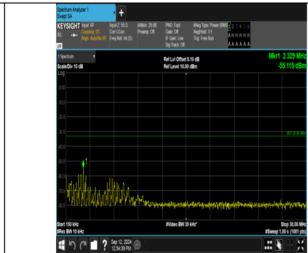
Band2_5MHz_QPSK_18625_1RB#0_0.15~30_0.15~30
