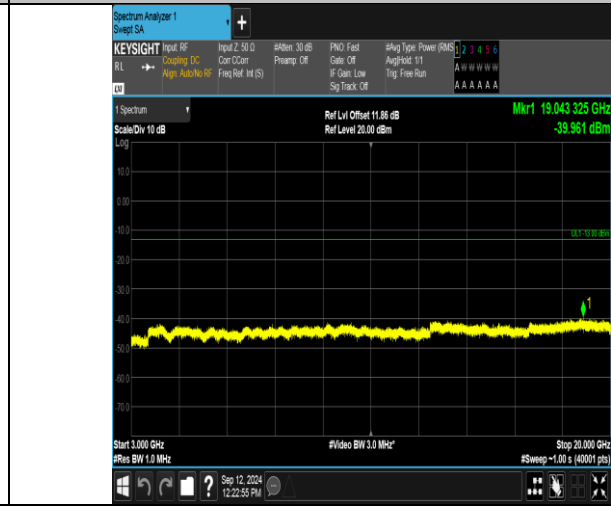
Band2_3MHz_16QAM_19185_15RB#0_3000-20000_3000-20000
