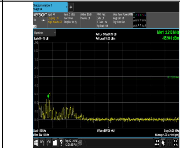
Band2_3MHz_QPSK_19185_15RB#0_0.15~30_0.15~30
