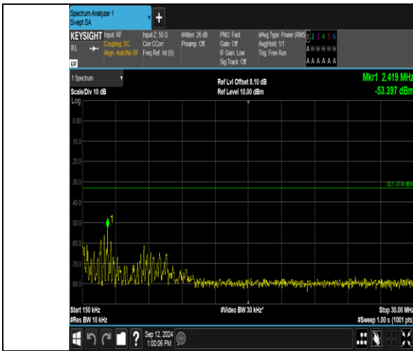
Band2_5MHz_16QAM_18900_1RB#0_0.15~30_0.15~30
