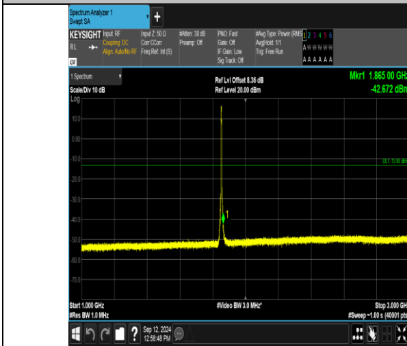
Band2_5MHz_16QAM_18625_25RB#0_1000-3000_1000-3000
