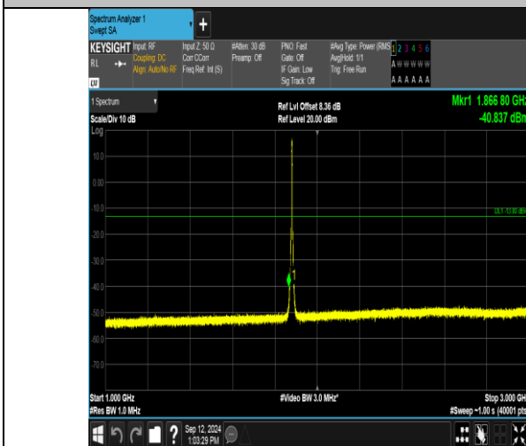
Band2_5MHz_16QAM_18900_25RB#0_1000-3000_1000-3000
