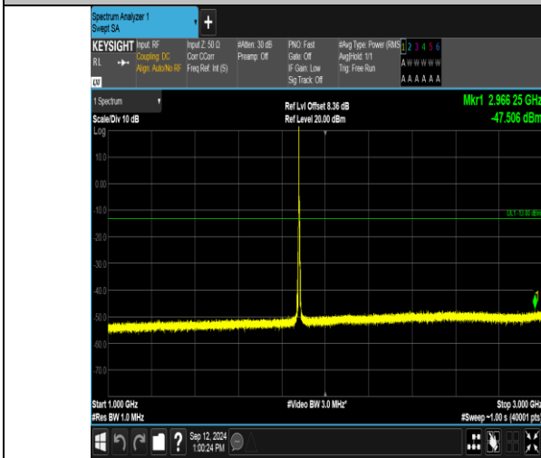
Band2_5MHz_16QAM_18900_1RB#0_1000~3000_1000~3000
