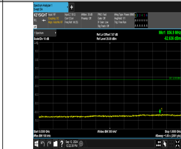
Band2_3MHz_16QAM_19185_15RB#0_30-1000_30-1000
