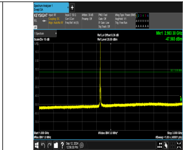
Band2_5MHz_QPSK_18625_1RB#24_1000~3000_1000~3000
