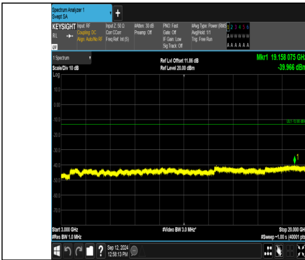
Band2_5MHz_QPSK_18625_25RB#0_3000-20000_3000-20000
