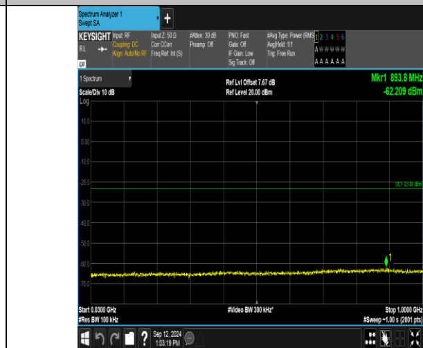
Band2_5MHz_16QAM_18900_25RB#0_30-1000_30-1000
