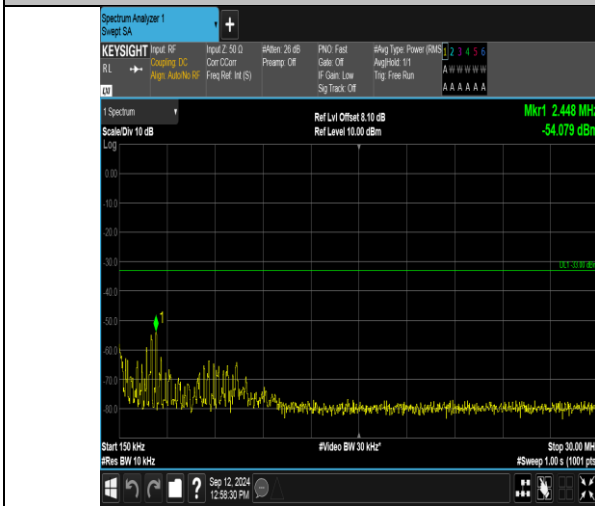
Band2_5MHz_16QAM_18625_25RB#0_0.15-30_0.15-30
