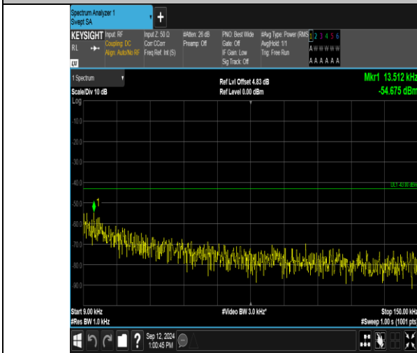
Band2_5MHz_QPSK_18900_1RB#24_0.009~0.15_0.009~0.15
