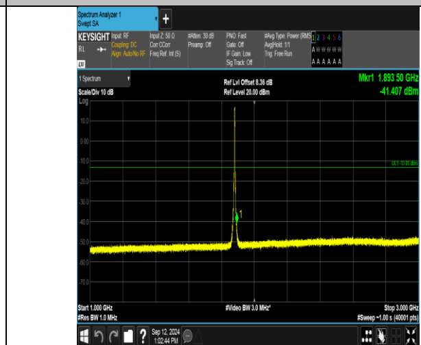
Band2_5MHz_QPSK_18900_25RB#0_1000~3000_1000~3000
