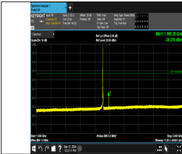
Band2_3MHz_16QAM_19185_1RB#14_1000~3000_1000~3000
