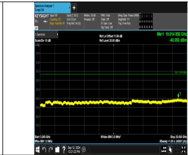
Band2_3MHz_16QAM_19185_1RB#14_3000~20000_3000~20000
