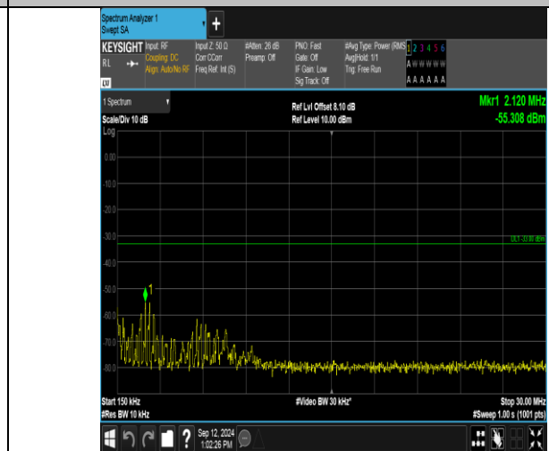
Band2_5MHz_QPSK_18900_25RB#0_0.15~30_0.15~30
