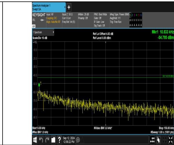
Band2_5MHz_16QAM_18625_25RB#0_0.009-0.15_0.009-0.15
