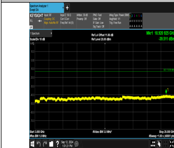
Band2_5MHz_QPSK_18900_1RB#24_3000~20000_3000~20000
