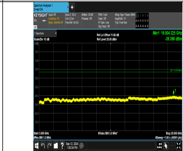
Band2_5MHz_16QAM_18900_1RB#0_3000~20000_3000~20000
