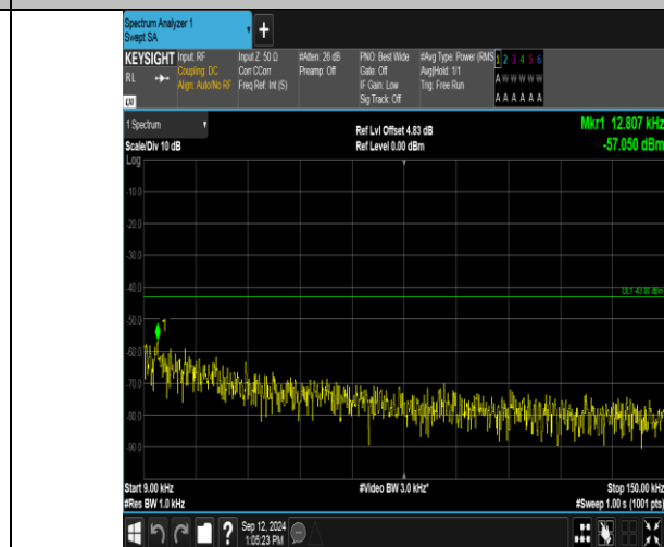
Band2_5MHz_16QAM_19175_1RB#0_0.009~0.15_0.009~0.15
