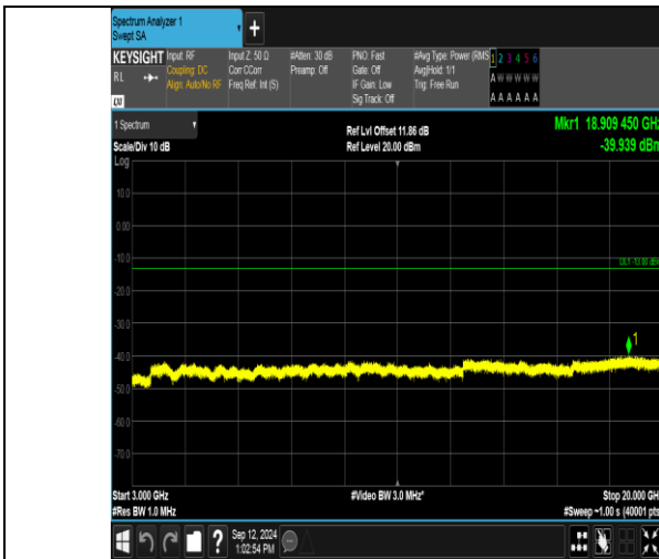
Band2_5MHz_QPSK_18900_25RB#0_3000-20000_3000-20000
