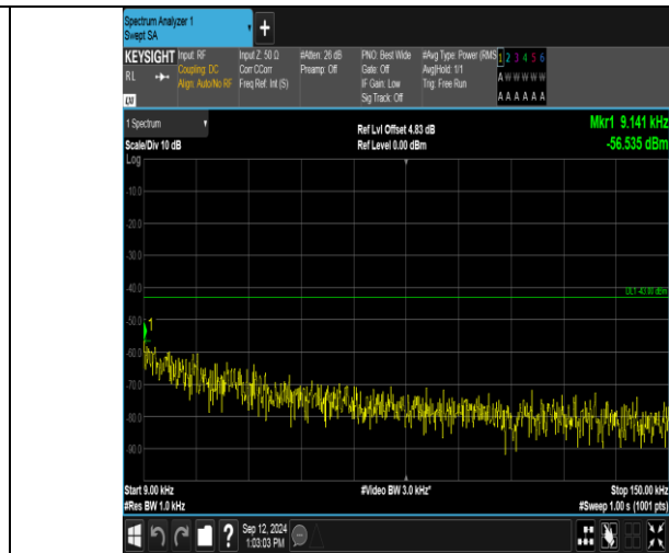
Band2_5MHz_16QAM_18900_25RB#0_0.009-0.15_0.009-0.15
