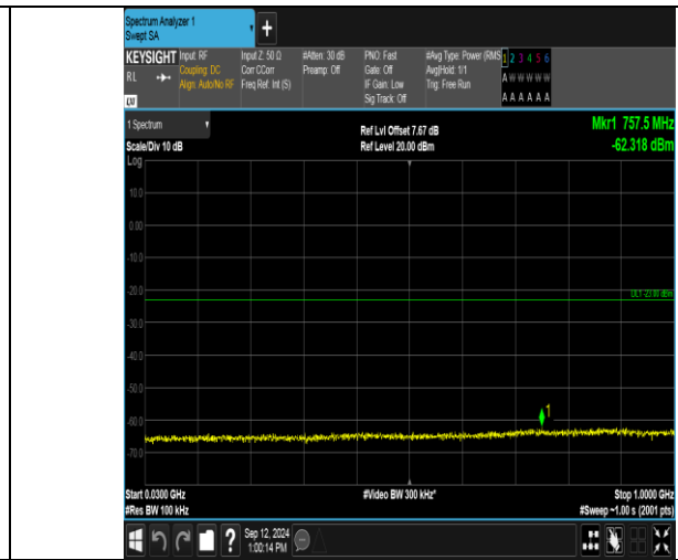
Band2_5MHz_16QAM_18900_1RB#0_30~1000_30~1000
