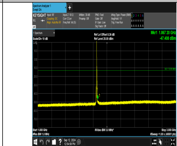
Band2_5MHz_QPSK_18625_1RB#0_1000~3000_1000~3000
