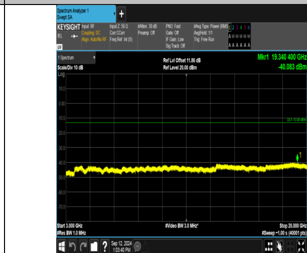
Band2_5MHz_16QAM_18900_25RB#0_3000-20000_3000-20000
