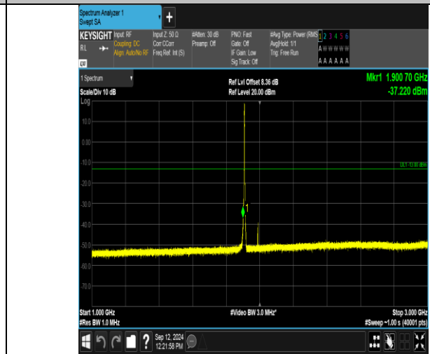
Band2_3MHz_QPSK_19185_15RB#0_1000~3000_1000~3000
