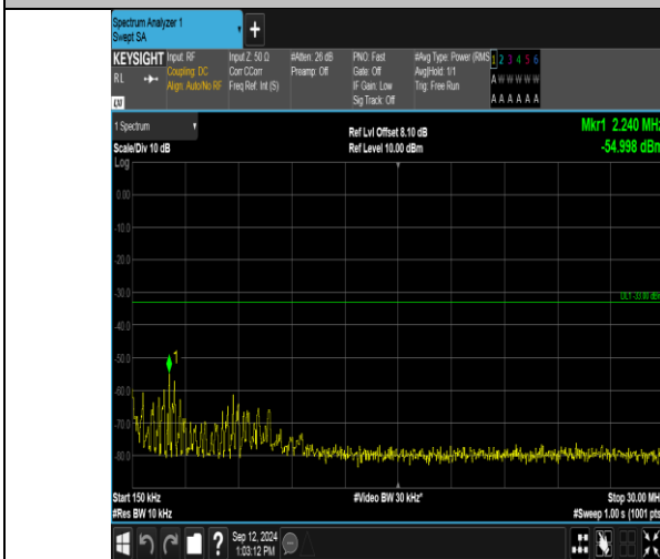
Band2_5MHz_16QAM_18900_25RB#0_0.15-30_0.15-30
