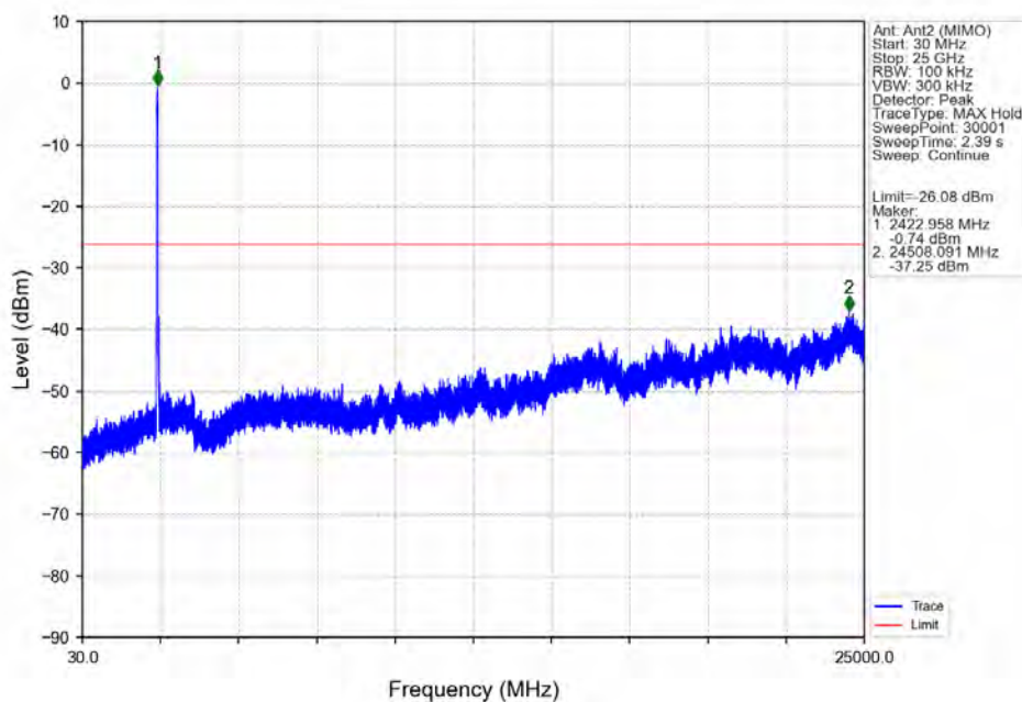
802.11ac(VHT40) LCH 2422MHz Ant2 (MIMO) NTN
