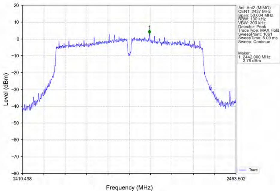
802.11ac(VHT40) MCH 2437MHz Ant2 (MIMO) NTN
