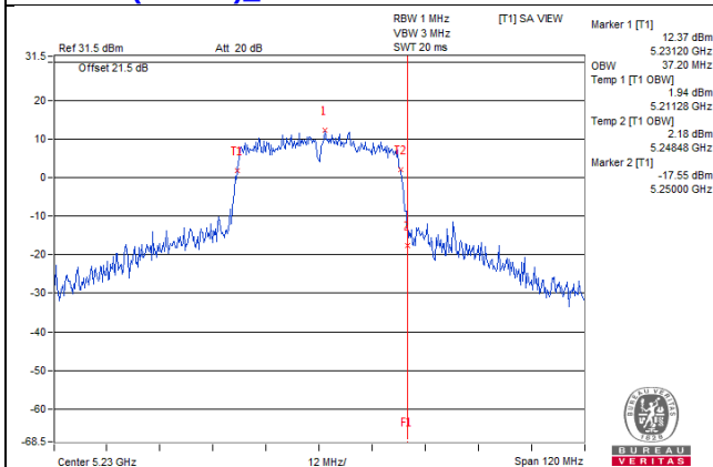
802.11ac(VHT40)_Chain0 / CH46
