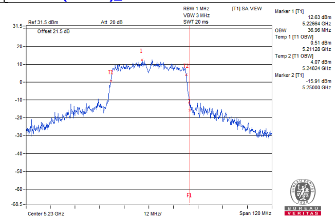
802.11ac(VHT40)_Chain1 / CH46
