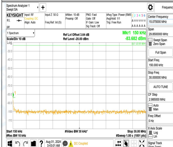
Band12_1.4MHz_QPSK_23095_1RB#0_0.15~30_0.15~30
