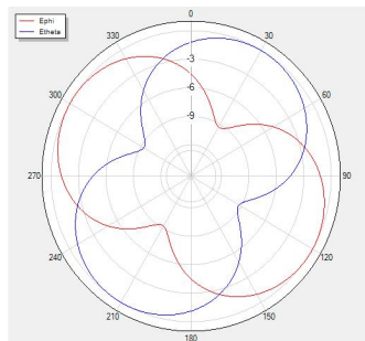
H Theta=90 freq=2450MHz
